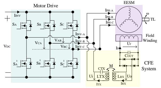
Fig. 2. The circuit diagram of the proposed system.
