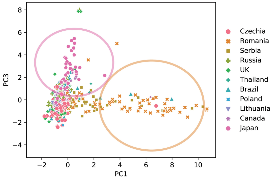
Extended Data Fig. 2 | Principal component analysis of relative mutation counts. PCA performed on relative mutation counts of all ccRCC tumors incorporating the six mutation classes (C > A, C > G, C > T, T > A, T > C, T > G). Principal component 1 (PC1) clearly separates the cluster of mostly Romanian
