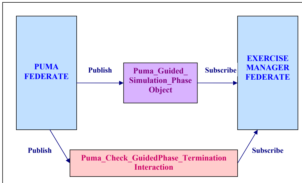
Figure 33 Federates and Relations in Guided Phase
