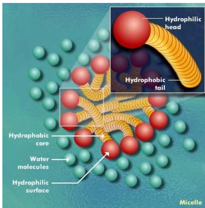
Figure 1.1 The schematic representation of a micelle.
