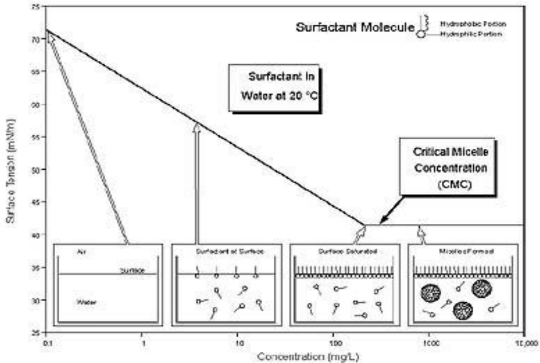
Figure 1.2 Schematic representation of micelle formation [97].
