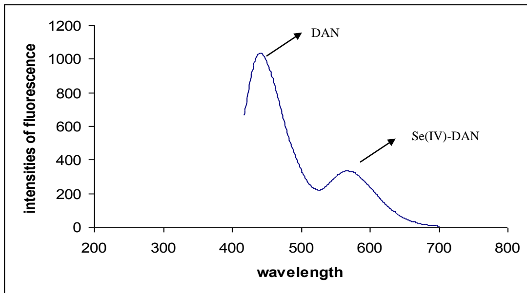
Figure 3.1 Fluorescence emission signals of DAN and Se(IV)-DAN complex in water ( \lambda_{em} = 440 nm for DAN and \lambda_{em} = 570 nm for Se(IV)-DAN complex).
