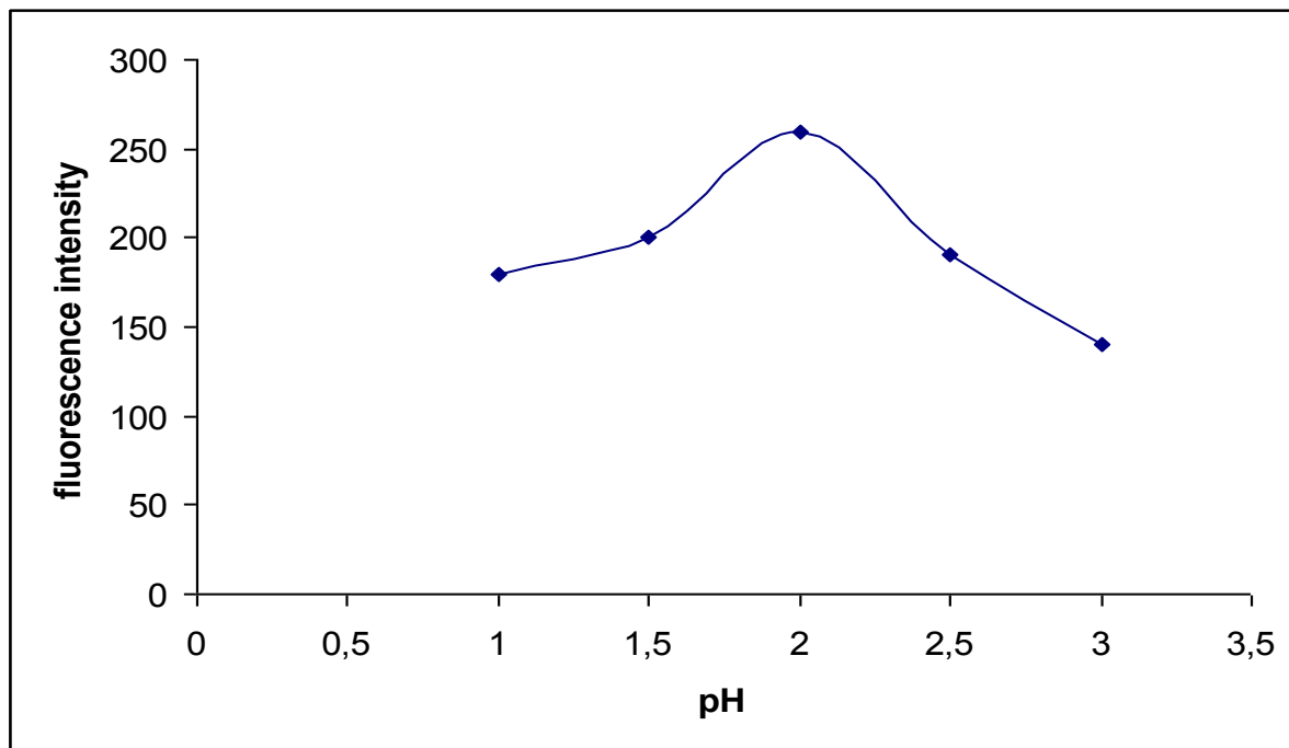
Figure 3.2 Effect of pH on the formation of Se(IV)-DAN complex. ( \lambda_{em} = 570 nm for Se(IV)-DAN complex).
