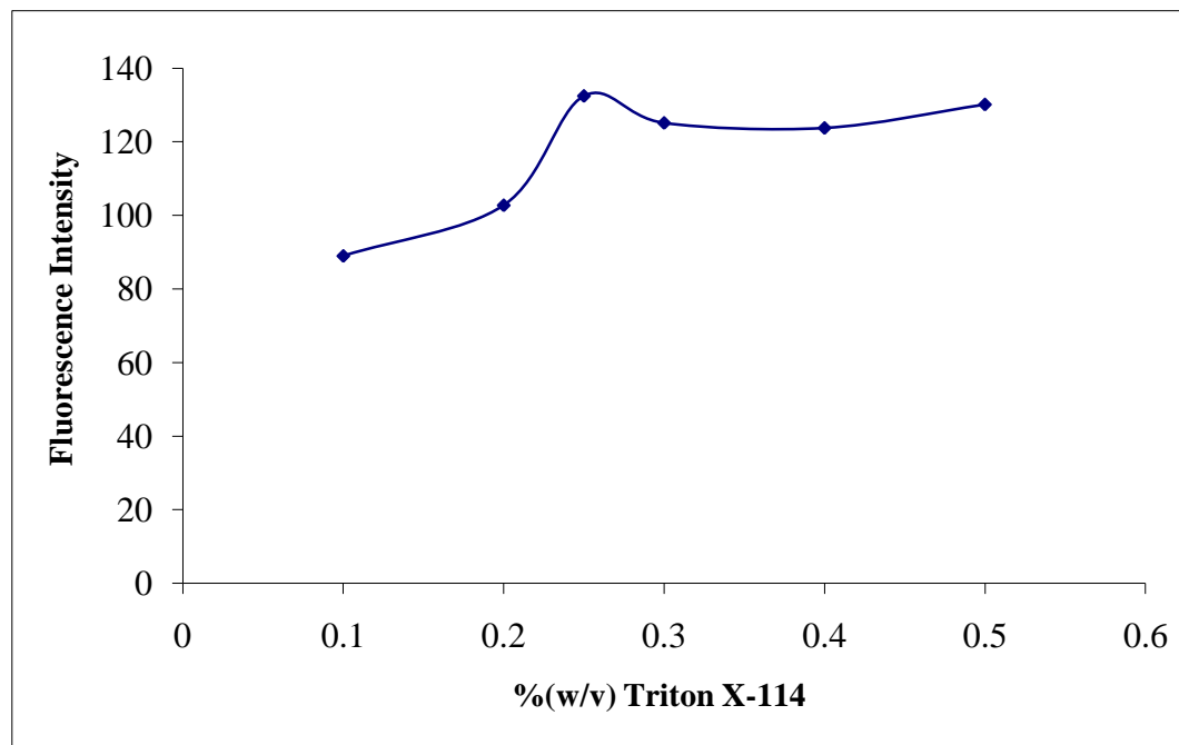
Figure 3.3 Effect of surfactant concentration on the fluorescence intensity of Se-DAN complex. ( \lambda_{em} = 570 nm for Se(IV)-DAN complex)
