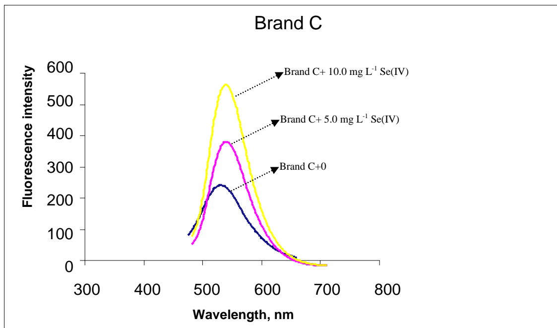
Figure 3.10 Fluorescence spectra of Se(IV)-DAN obtained from Brand C after cloud point extraction
