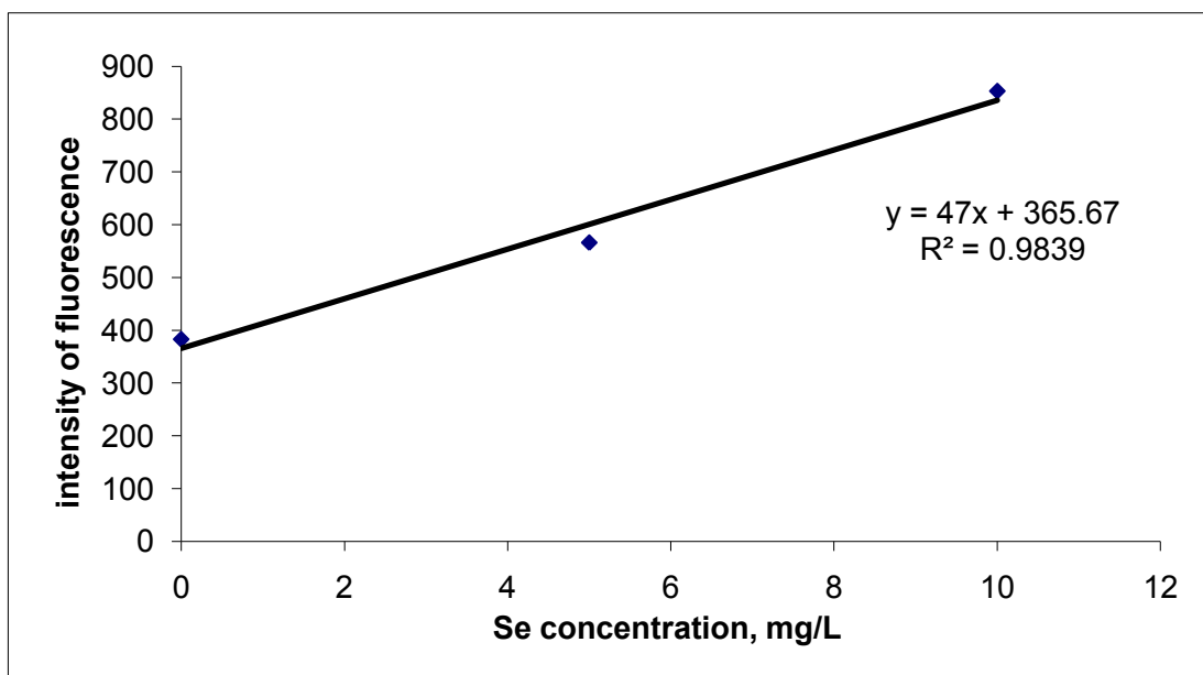
Figure 3.9 Calibration curve of Se(IV)-DAN obtained from Brand B after cloud point extraction
