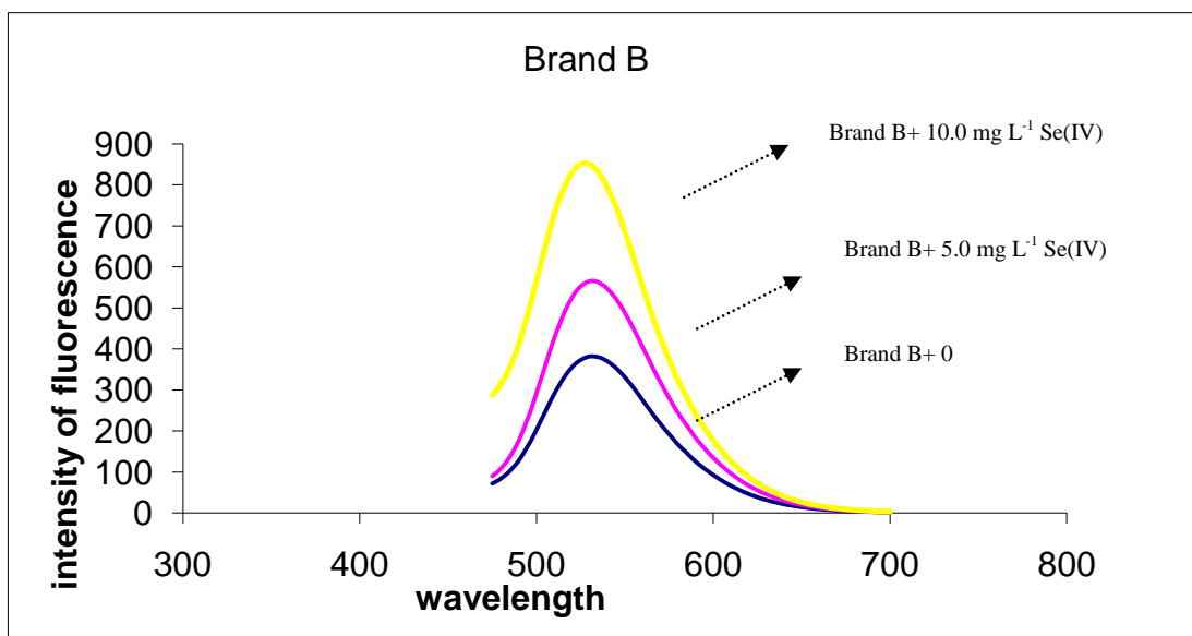
Figure 3.8 Fluorescence spectra of Se(IV)-DAN obtained from Brand B after cloud point extraction.
