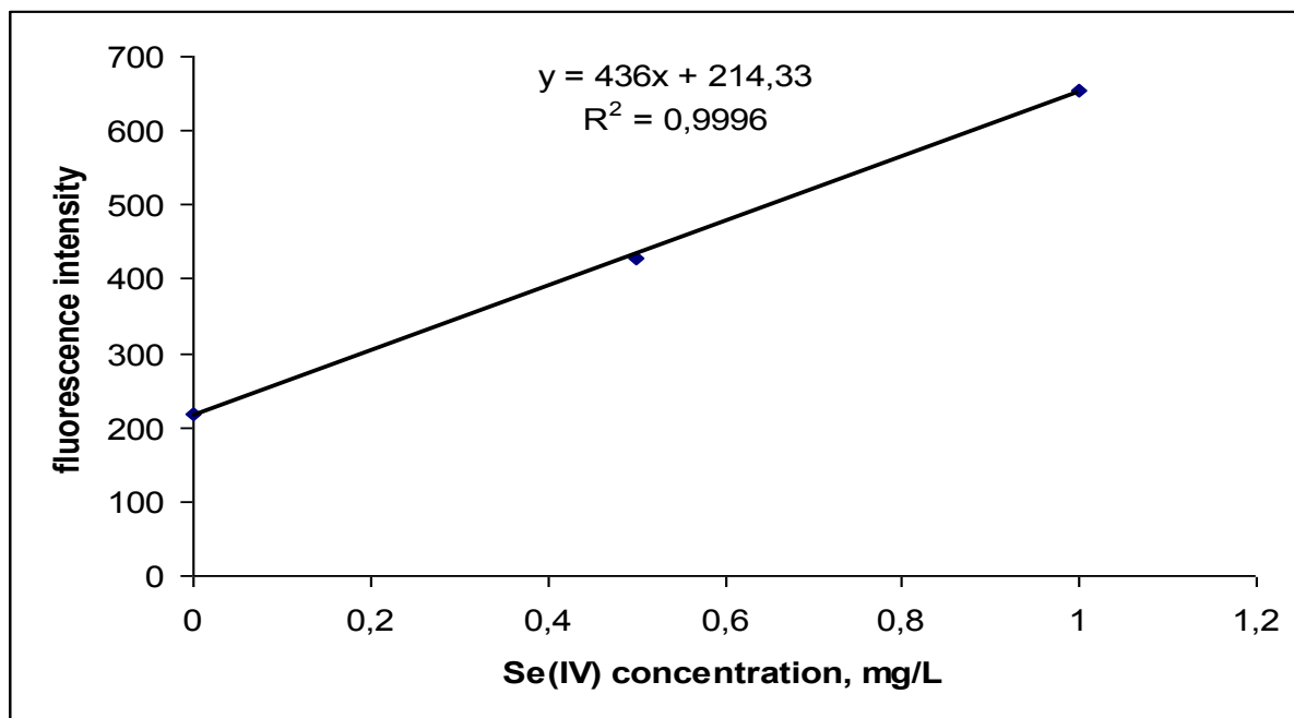
Figure 3.5 Calibration curve of Se(IV)-DAN obtained from SRM after cloud point extraction
