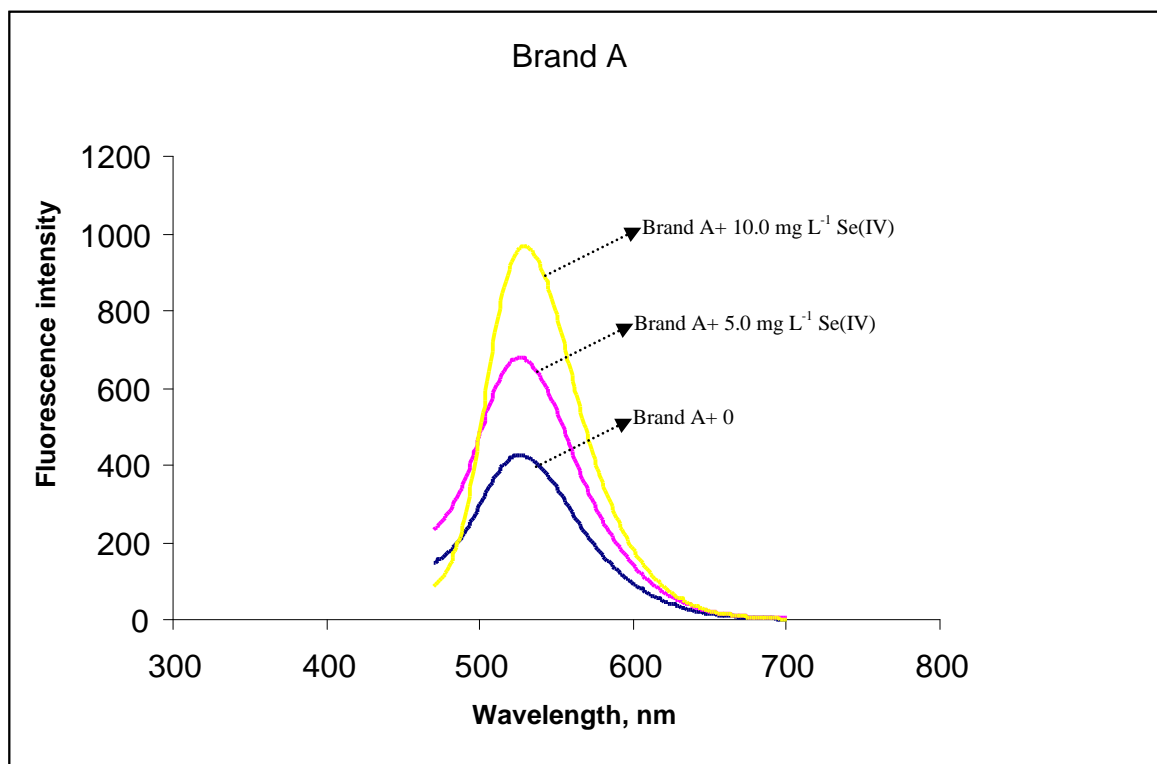
Figure 3.6 Fluorescence spectra of Se(IV)-DAN obtained from Brand A after cloud point extraction using the optimum parameters.
