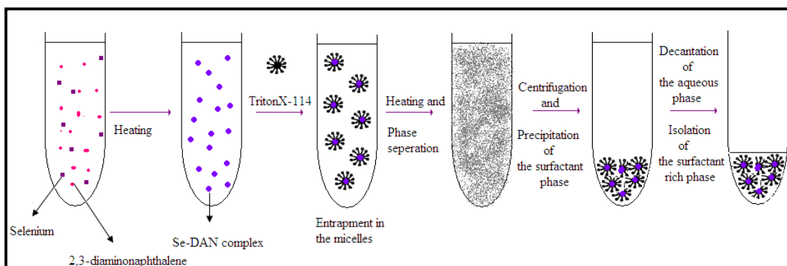
Figure 2.1 Procedure steps of complex formation and Preconcentration of complex by surfactant.
