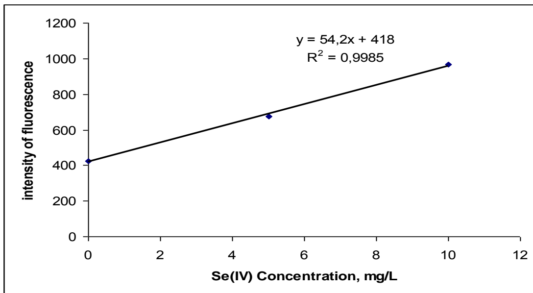
Figure 3.11 Calibration curve of Se(IV)-DAN obtained from Brand C after cloud point extraction.
