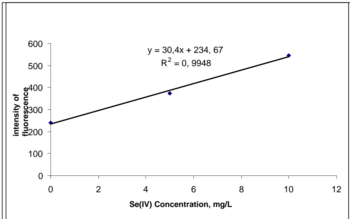
Figure 3.7 Calibration curve of Se(IV)-DAN obtained from Brand A after cloud point extraction.
