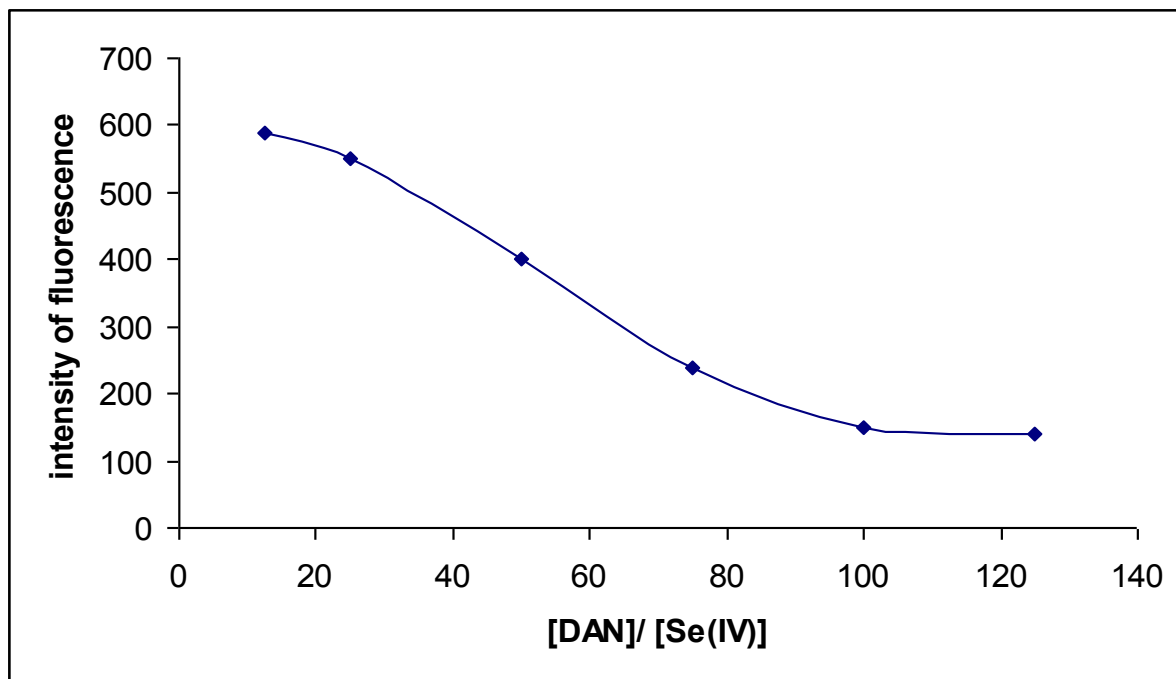
Figure 3.4 Effect of DAN / Se(IV) molar ratio on fluorescence intensity of Se(IV)-DAN complex. ( \lambda_{em} = 570 nm for Se(IV)-DAN complex)
