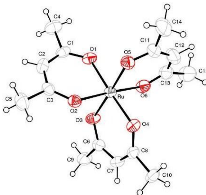
Figure 1.1 Crystal structure of \text{Ru}(\text{acac})_3 acting as homogeneous catalyst in the dehydrogenation of dimethylamine borane.
