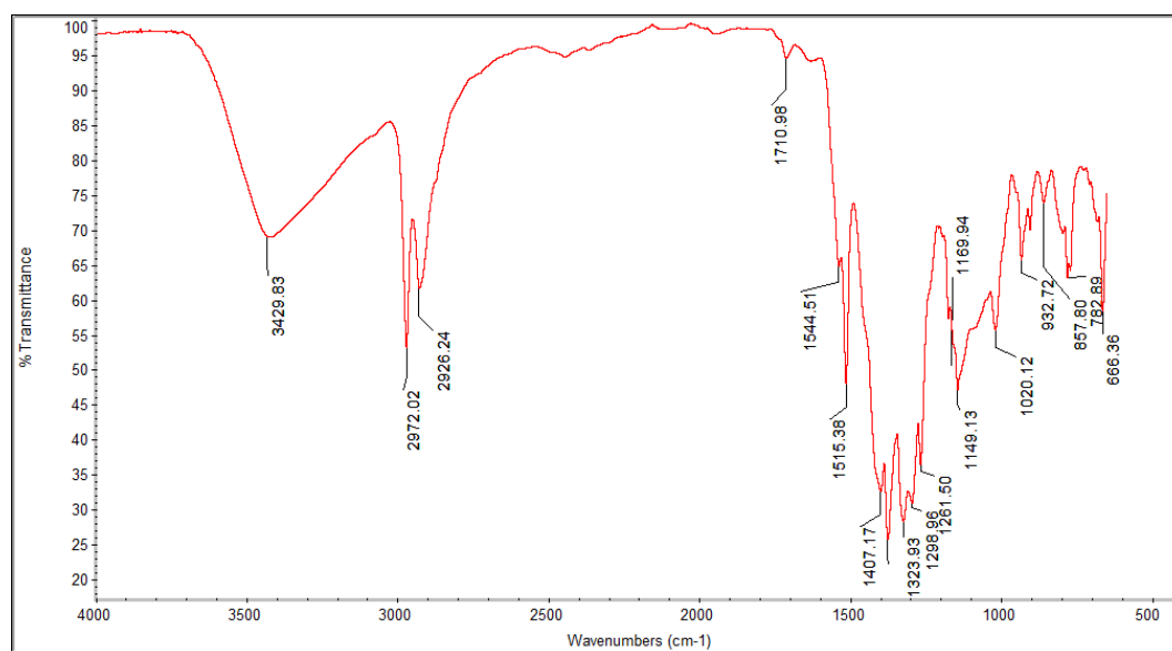
Figure 3.5 FTIR spectrum of the isolated ruthenium(II) species after catalytic dehydrogenation of dimethylamine borane (500mM) starting with \text{Ru}(\text{acac})_3 (5mM), taken from the ATR unit.
