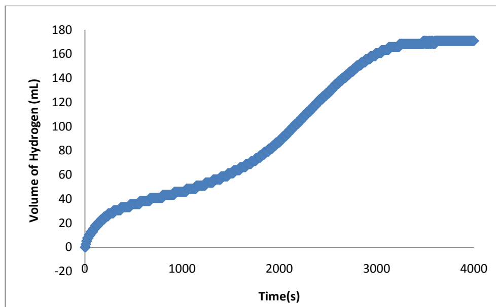
Figure 3.3 Plots of hydrogen volume versus time for the dehydrogenation of dimethylamine borane (500 mM) catalyzed by Ru(acac) 3 (5 mM) as pre-catalyst in 10 mL toluene at 60 °C.
