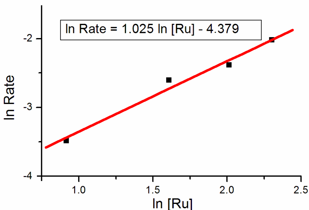
Figure 3.12 Plot of hydrogen generation rate versus the concentration of ruthenium (both in logarithmic scales) for the dehydrogenation of dimethylamine borane (500 mM) started with \text{Ru}(\text{acac})_3 at 60\text{ }^\circ\text{C} after the induction time.
