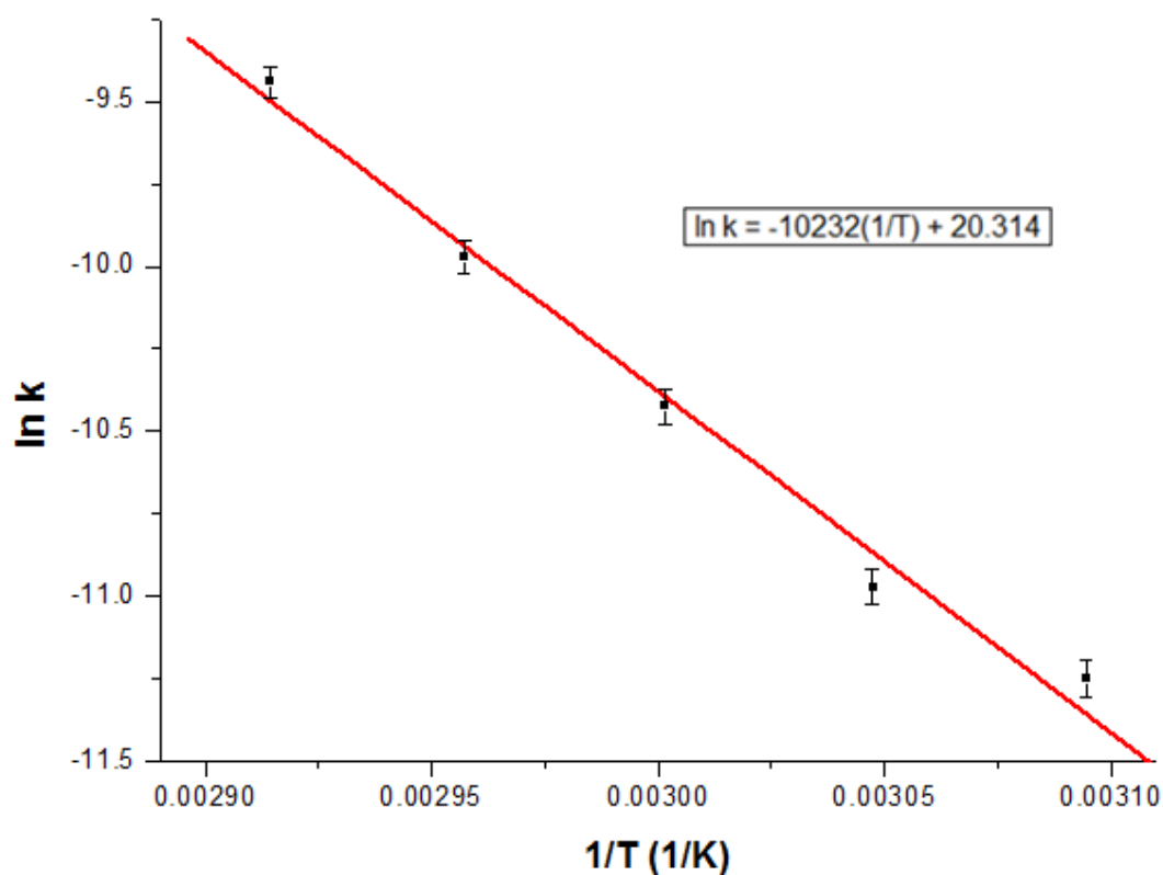
Figure 3.16 Arrhenius plot for dehydrogenation of dimethylamine borane starting with a solution containing 500 mM \text{NH}(\text{CH}_3)_2\text{BH}_3 and 5.0 mM \text{Ru}(\text{acac})_3 at different temperatures.
