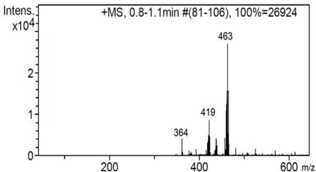
Figure 3.6 Mass spectrum of the ruthenium species, [\text{Ru}\{\text{N}_2\text{Me}_4\}_3(\text{acac})\text{H}] , isolated after catalytic dehydrogenation of dimethylamine borane starting with \text{Ru}(\text{acac})_3 .
