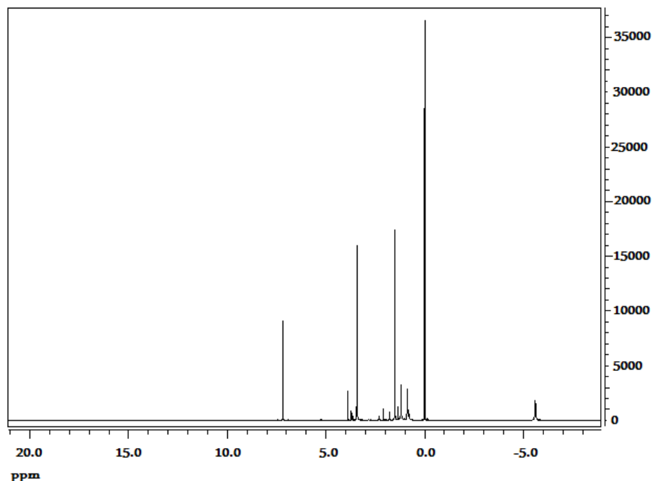
Figure 3.7 ^1\text{H} NMR spectrum of the ruthenium species, [\text{Ru}\{\text{N}_2\text{Me}_4\}_3(\text{acac})\text{H}] , isolated after catalytic dehydrogenation of dimethylamine borane (500 mM) starting with \text{Ru}(\text{acac})_3 (5mM). The peaks at 7 and 1.5 ppm belong to chloroform.
