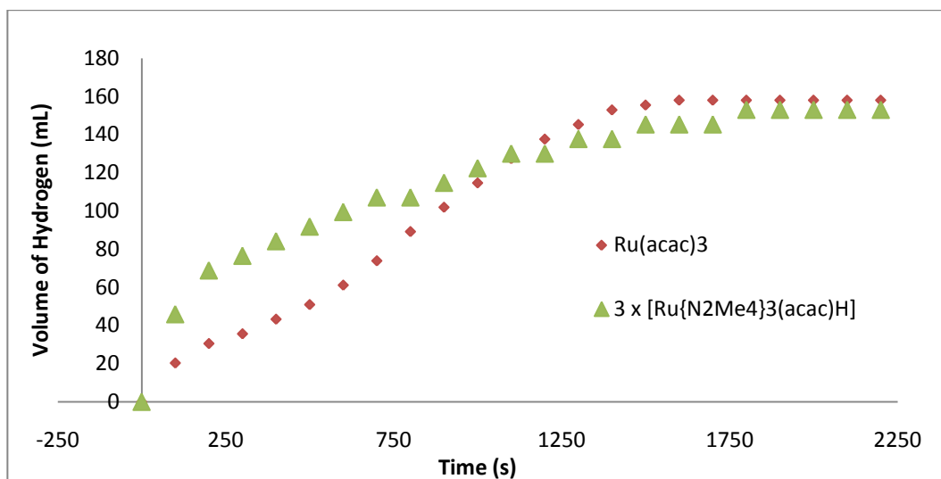
Figure 3.10 Comparison of dehydrogenation of dimethylamine borane (500 mM) catalyzed by Ru(acac) 3 (5 mM) and isolated ruthenium species, [Ru{N 2 Me 4 } 3 (acac)H] (1.65 mM) at 60.0 ± 0.1 °C. The data obtained for the latter complex was corrected by a factor of 3.
