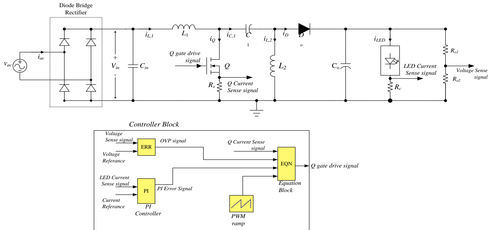
Figure 4.20 SEPIC converter simulation application circuit
