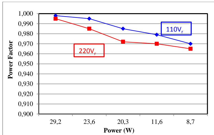
Figure 4.36 SEPIC converter power factor versus loading
