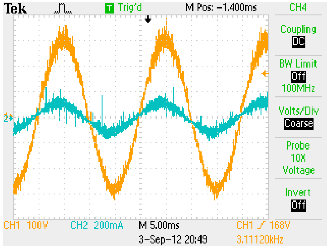
Figure 4.32 SEPIC converter V_{in} = 110 V; input line voltage (yellow) and input line current (blue) at 30W output power (Scales:100 V/div, 200 mA/div, Time: 5 ms/div)
