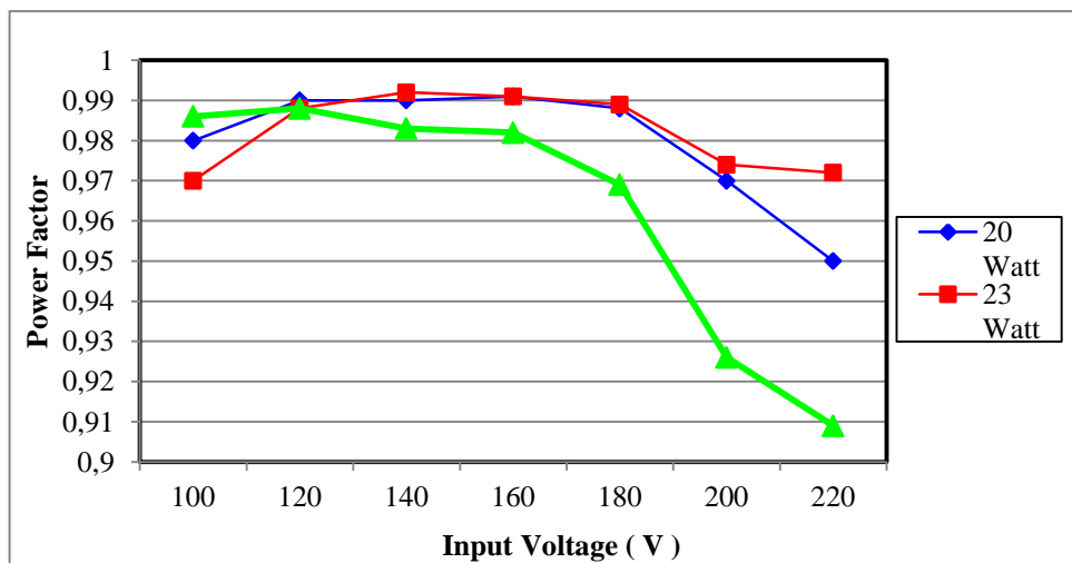
Figure 4.38 SEPIC converter power factor change due to input voltage for different power levels
