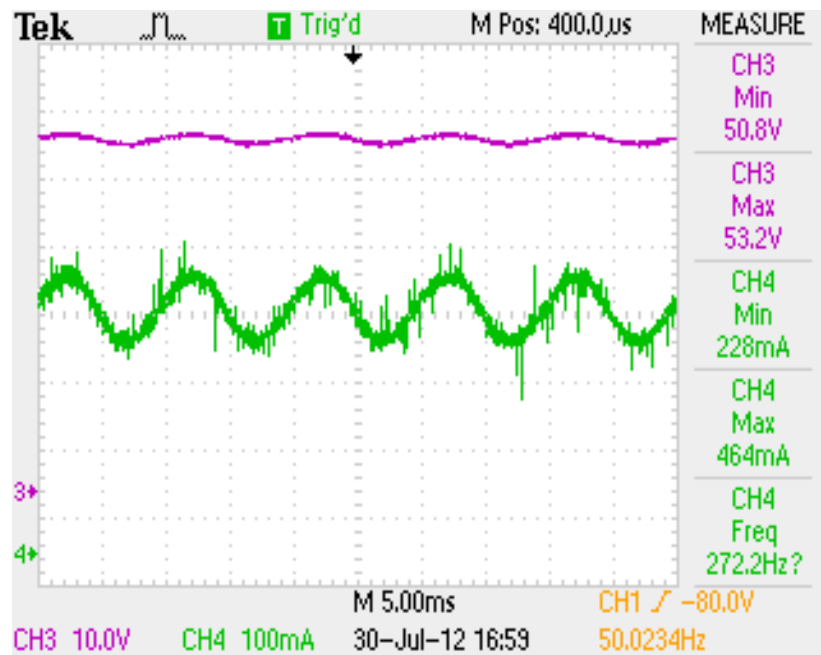
Figure 4.35 SEPIC converter output voltage (purple) and output current (green) at 20W output power (Scales: purple 10 V/div, green 100 mA/div, Time: 5 ms/div)
