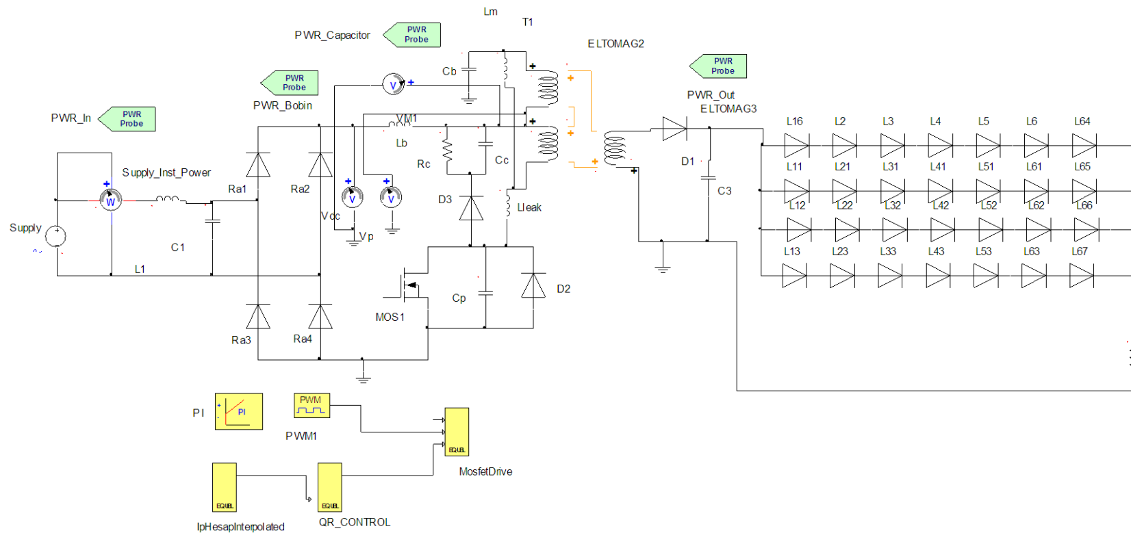
Figure 5.15 Flyback converter simulation application circuit layout
