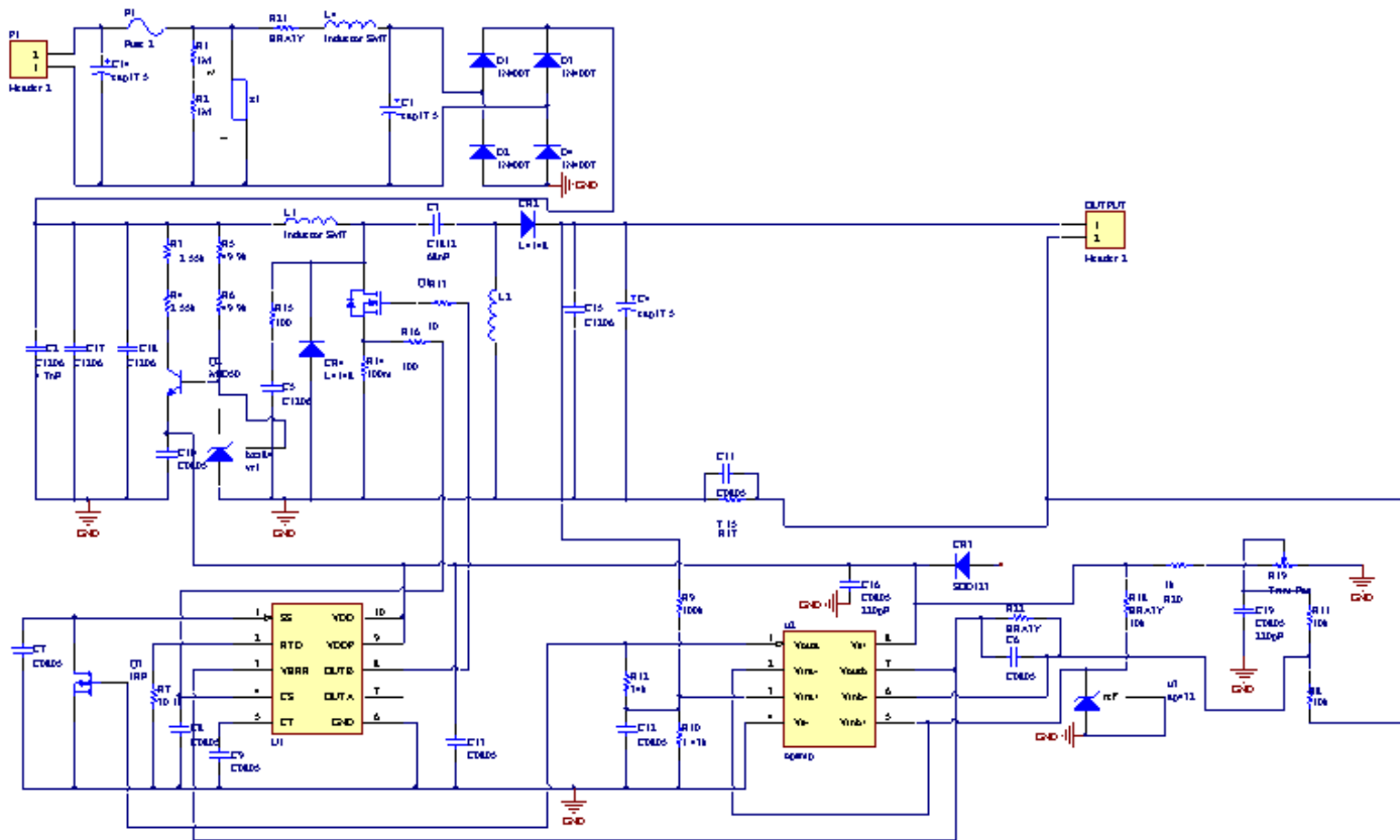
Figure 4.29 SEPIC converter schematic
