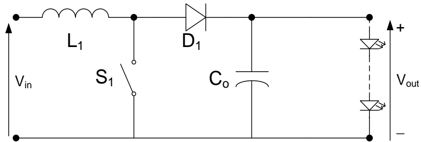
Figure 3.11 Boost converter basic schematic
