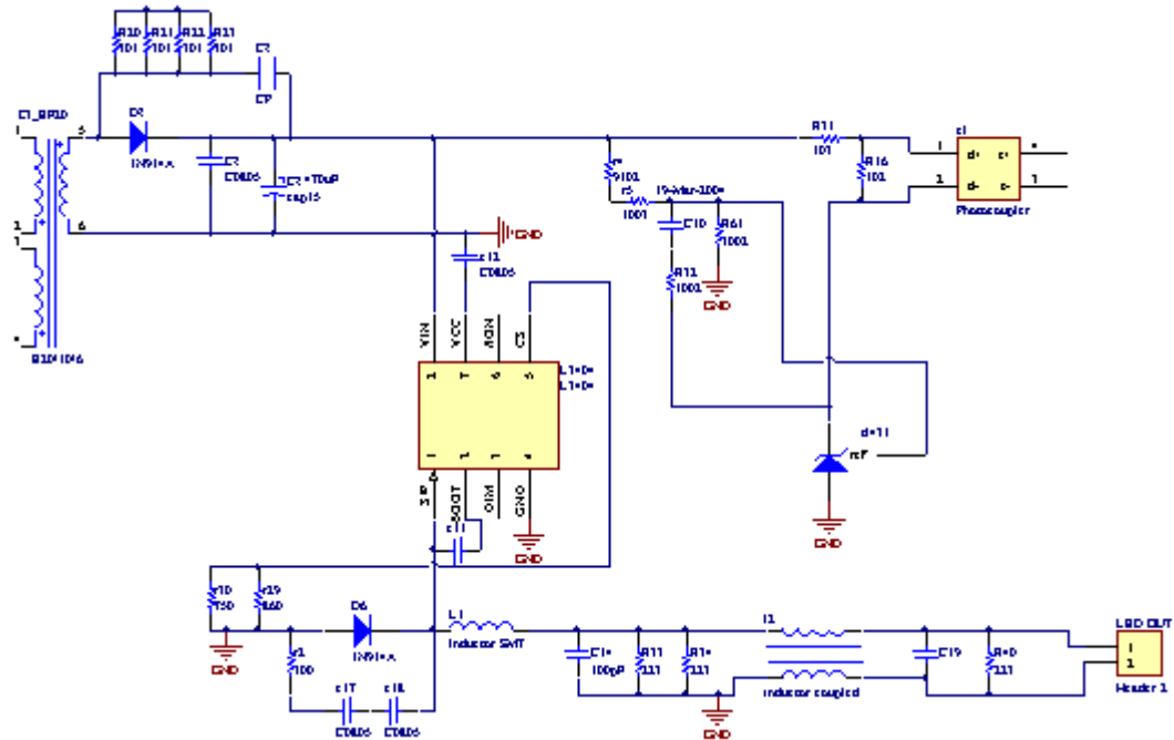
Figure 6.3 RECOM 30-700 converter schematic secondary side
