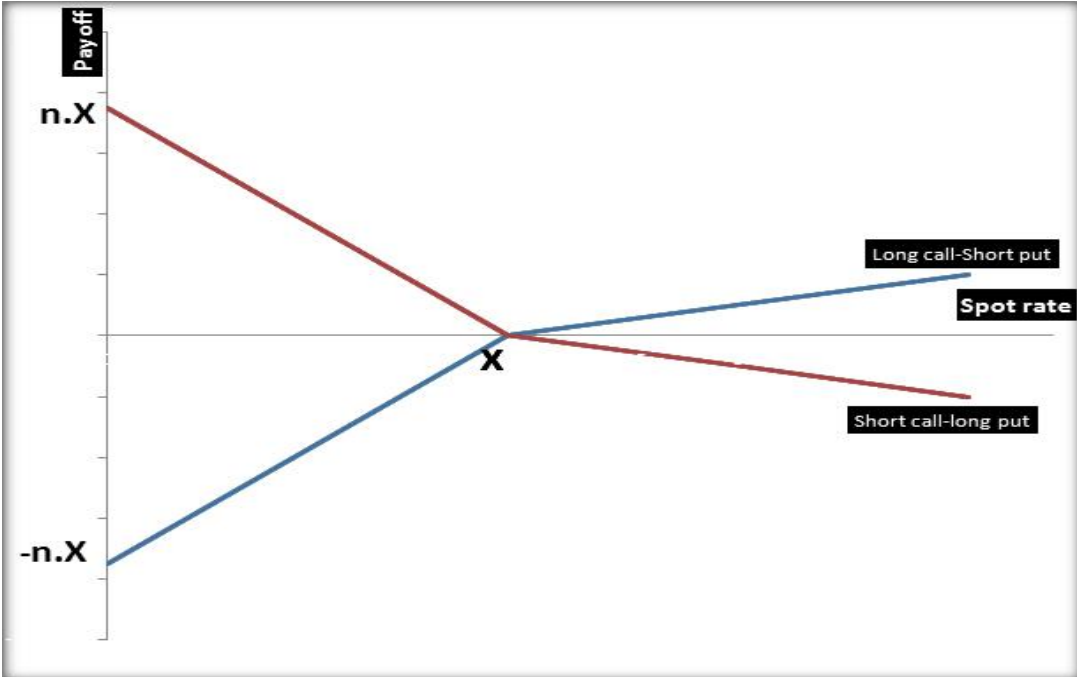
Figure 2.2: Contract payoff 2
