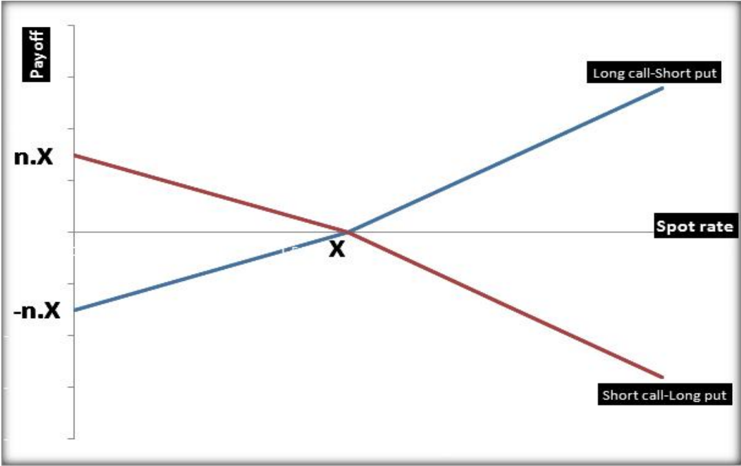
Figure 2.1: Contract payoff 1
