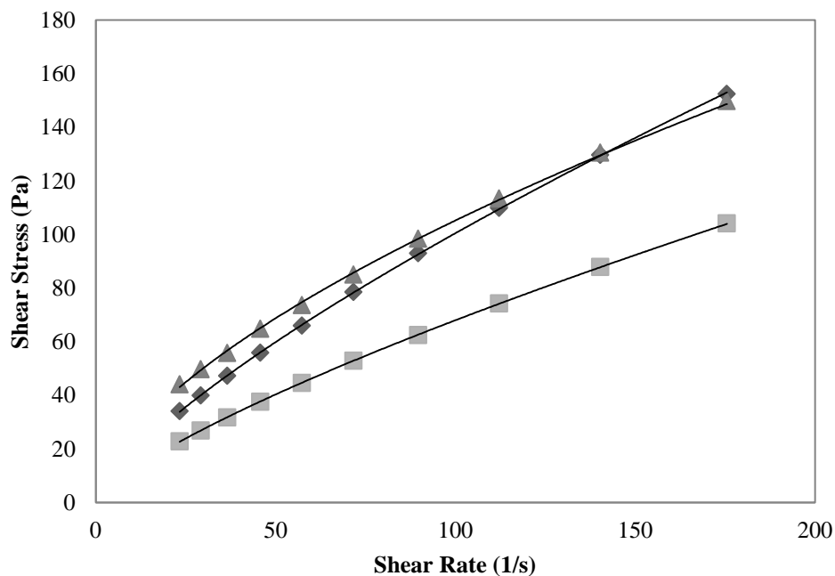
Figure 3.2 Flow curves for wafer batter samples containing RF and ChF in combination and control flours. (■): 100 WF, (◆): 100 RF, (▲): 80:20 RF:ChF, — : Power-law Model
