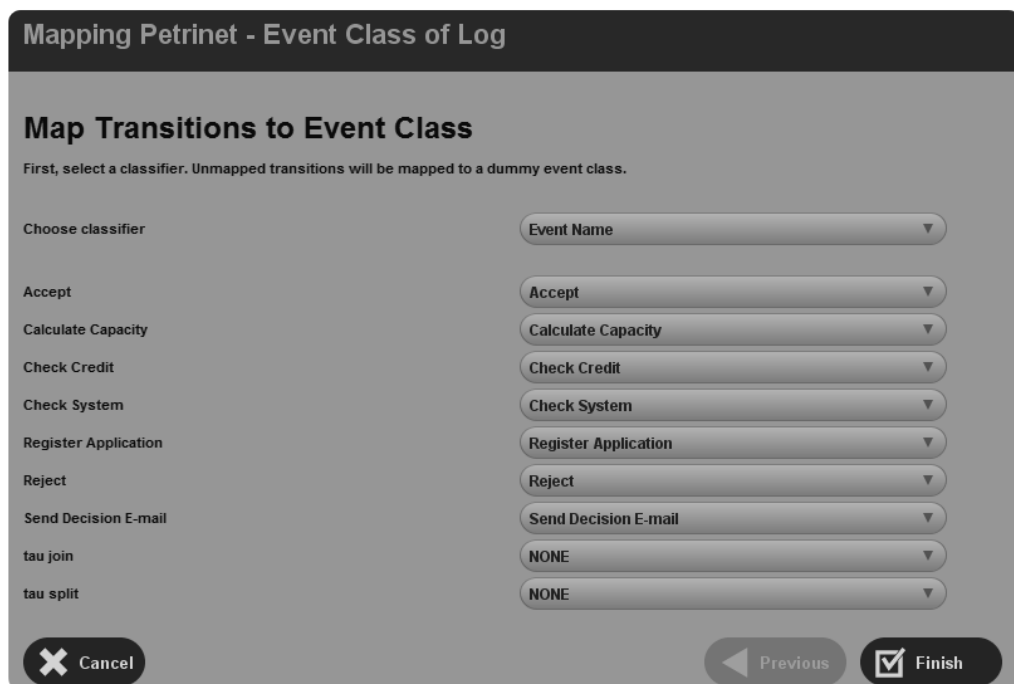
Figure A.4: Automated Replayer Screen of Cross-Organizational Process Miner Plugin
