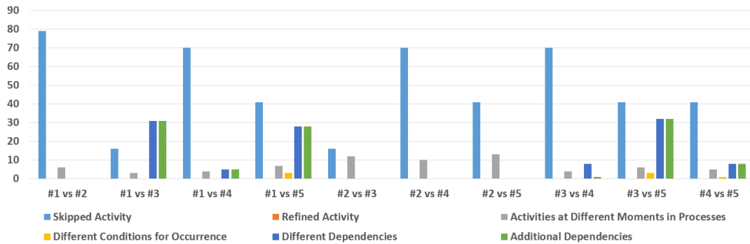
Figure 5.9: Mismatch pattern types for Environmental Permit Application Process dataset
