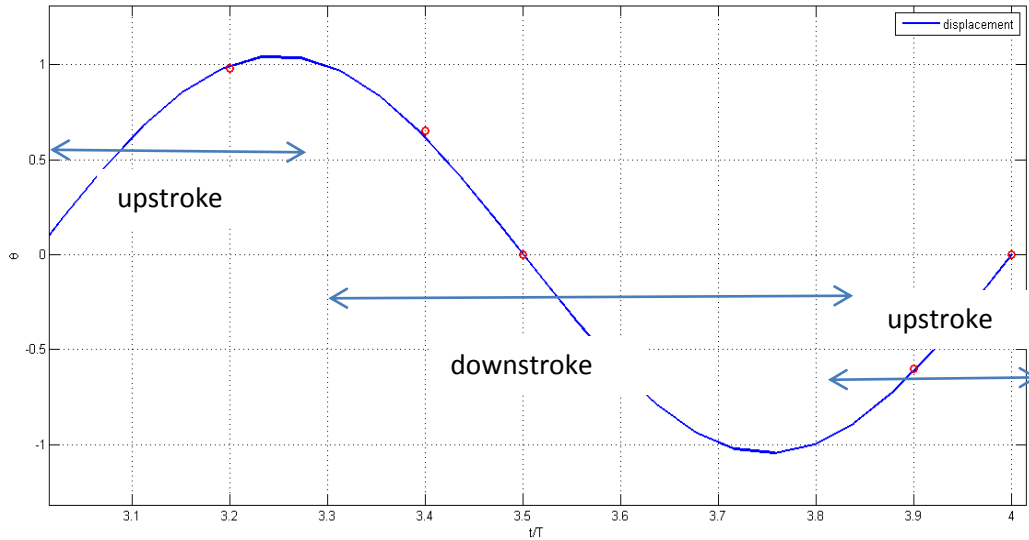
Figure 4.36: Sweeping position for 4th Period at case 6
