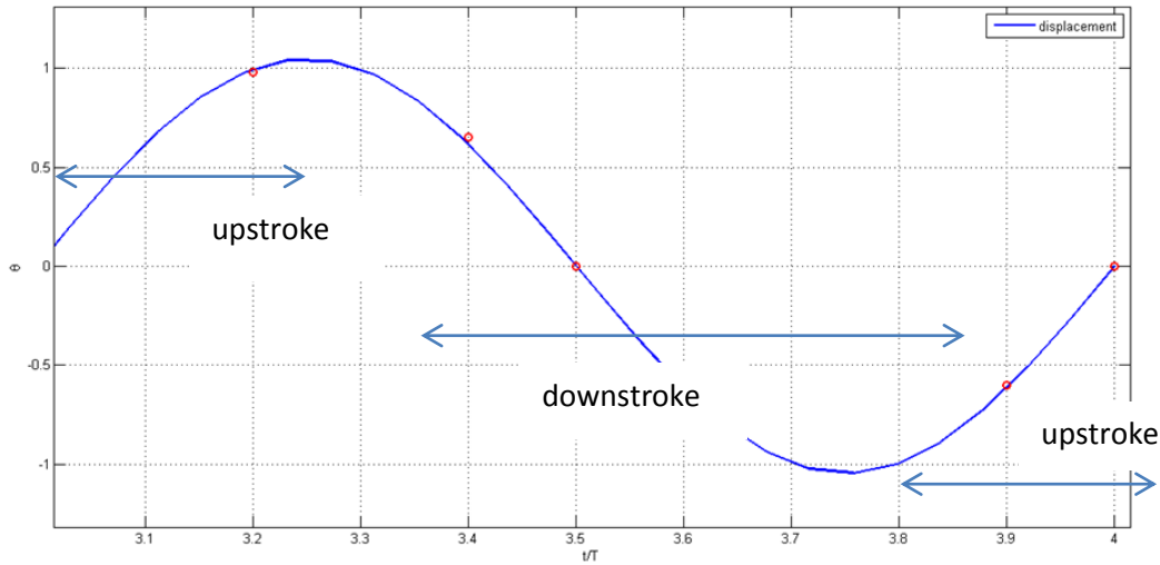
Figure 4.30: Sweeping position for 4th Period at case 5
