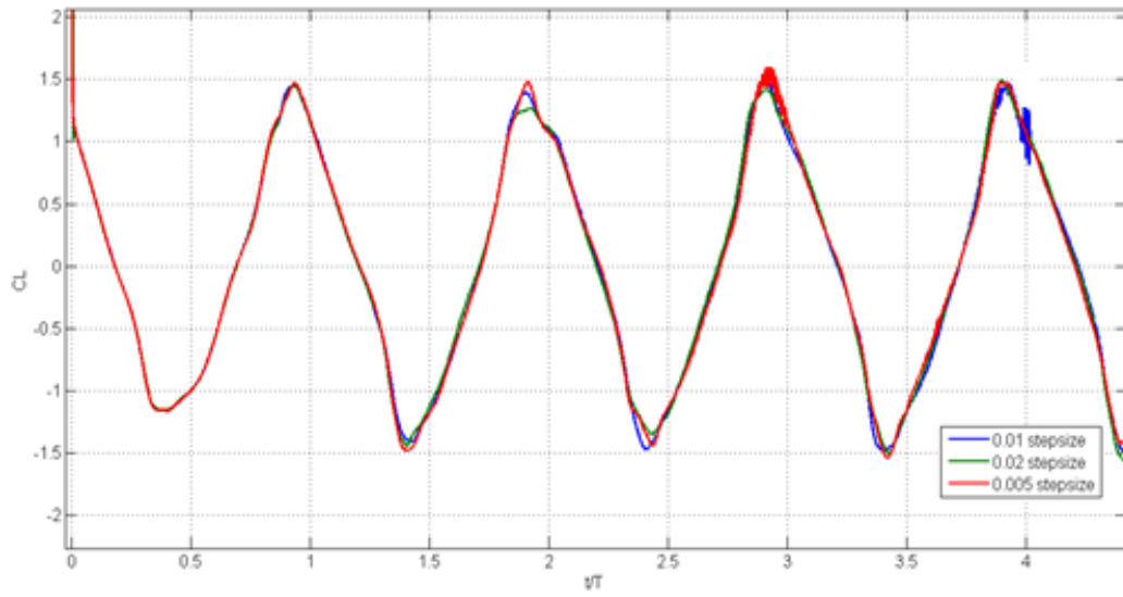
Figure 3. 14: Lift coefficient for time refinement studies
