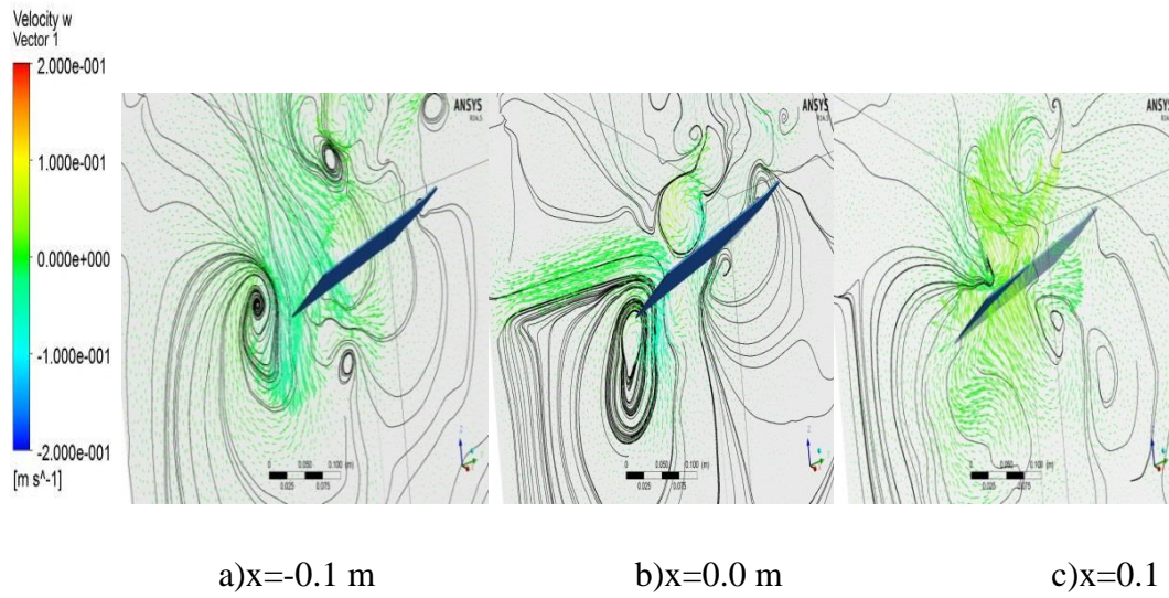
Figure 4.54 :Streamlines and velocity vectors at 30^\circ pitch angle and 30^\circ sweep angle ( t^*=3.3 )
