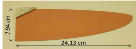
Figure 3. Flexible aluminum wing and support.
