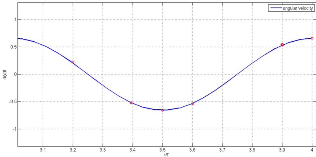
Figure 4.31: Sweeping velocity for 4th Period at case 5
