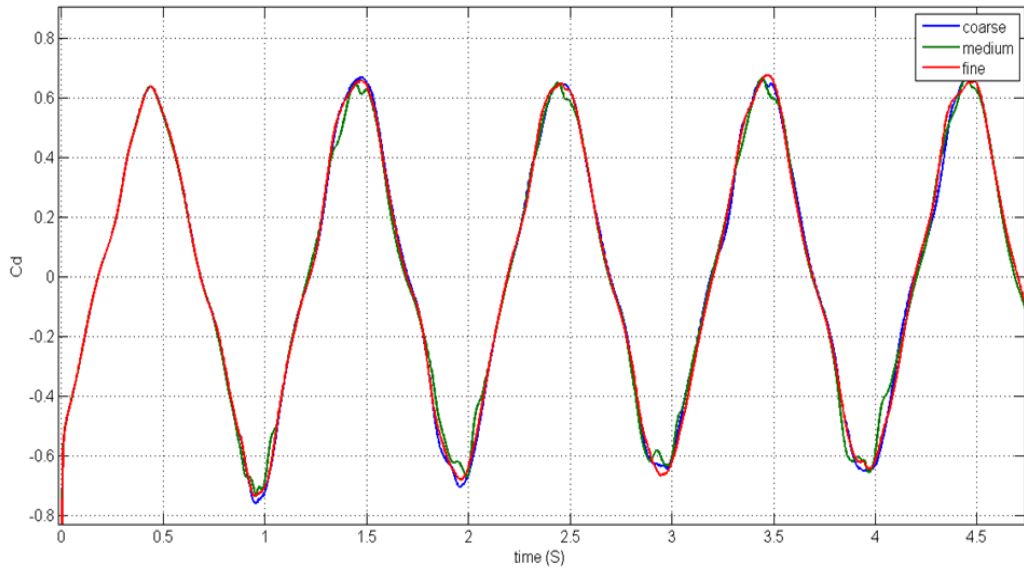
Figure 3.11 : Drag coefficient for coarse , medium and fine mesh studies
