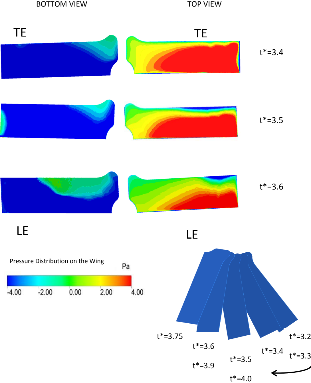
Figure 4.26: Top and bottom views at downstroke of 4th period for Case 5
