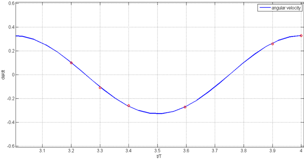
Figure 4.7 Angular velocity for 4th Period at case 1
