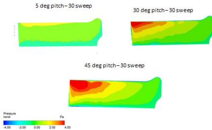
Figure 4.43 Pressure contours at t^*=3 (bottom surface)
