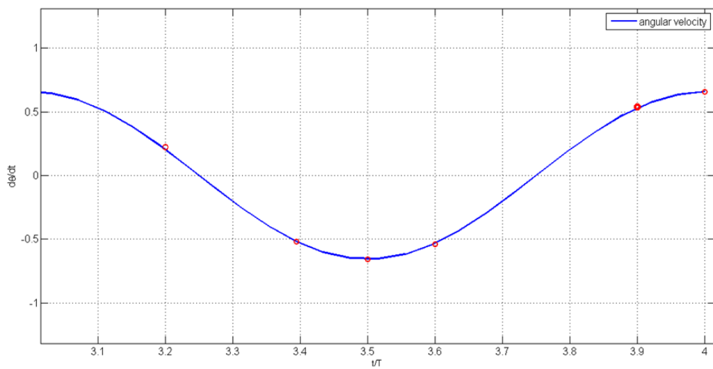
Figure 4.25: Sweeping velocity for 4th Period at case 4
