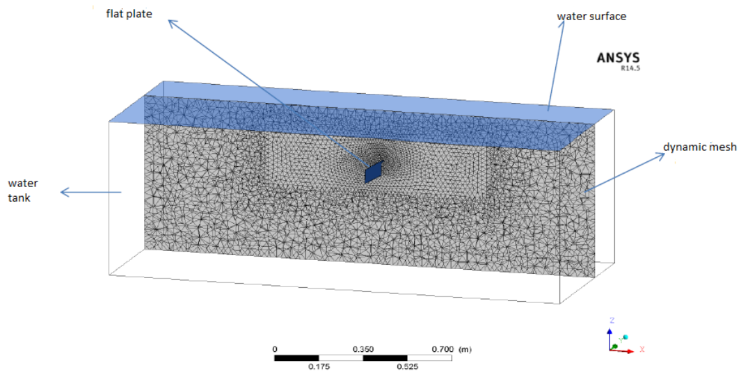
Figure 3.5 : Mesh view by using CFD post program
