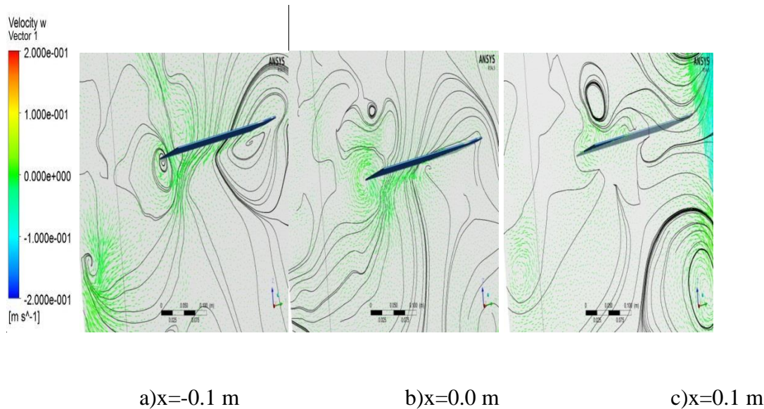
Figure 4.48 :Streamlines and velocity vectors at 5^\circ pitch angle and 30^\circ sweep angle ( t^*=3.3 )
