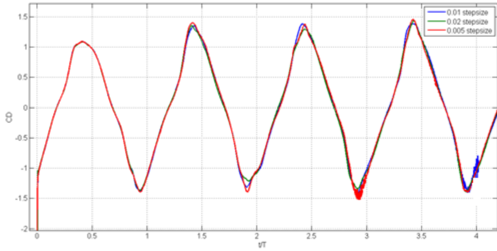
Figure 3. 13: Drag coefficient for time refinement studies
