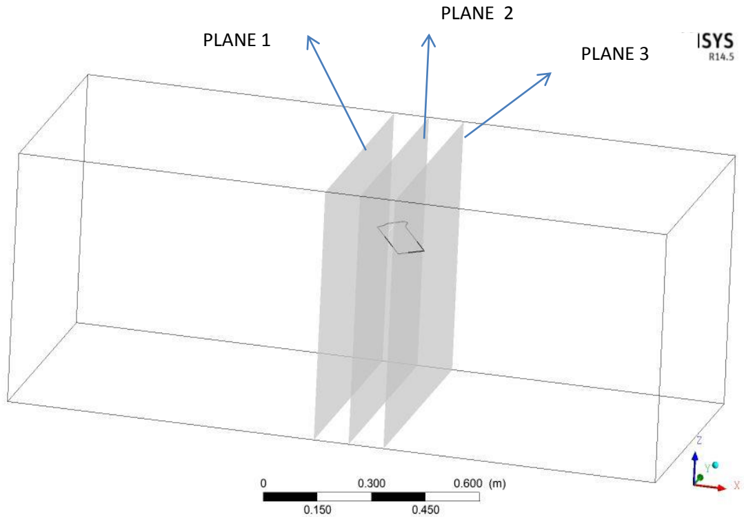
Figure 4.46: Three planes at different locations ( x=-0.1\text{ m}, 0\text{ m}, 0.1\text{ m} )
