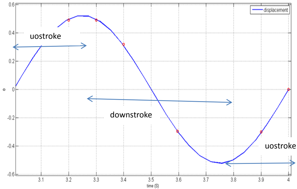
Figure 4.12: Sweeping position for 4th Period at case 2
