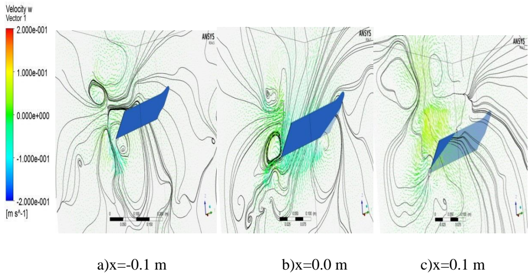
Figure 4.60 :Streamlines and velocity vectors at 45 0 pitch angle and 30 0 sweep angle ( t^*=3.3 )
