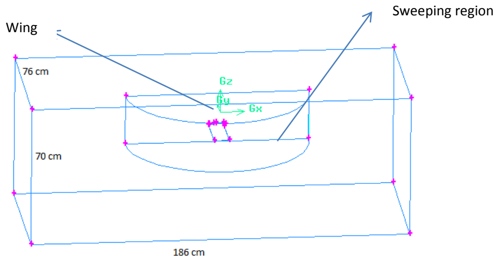
Figure 3.1 :Dimensions of water tank
