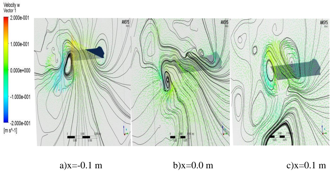
Figure 4.74 :Streamlines and velocity vectors at 30° pitch angle and 60° sweep angle ( t^*=3.6 )
