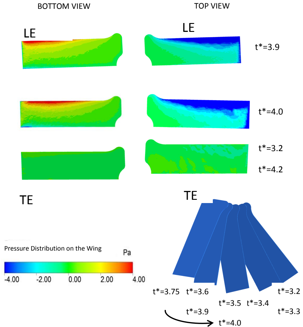
Figure 4.21: Top and bottom views at upstroke of 4th period for Case 4
