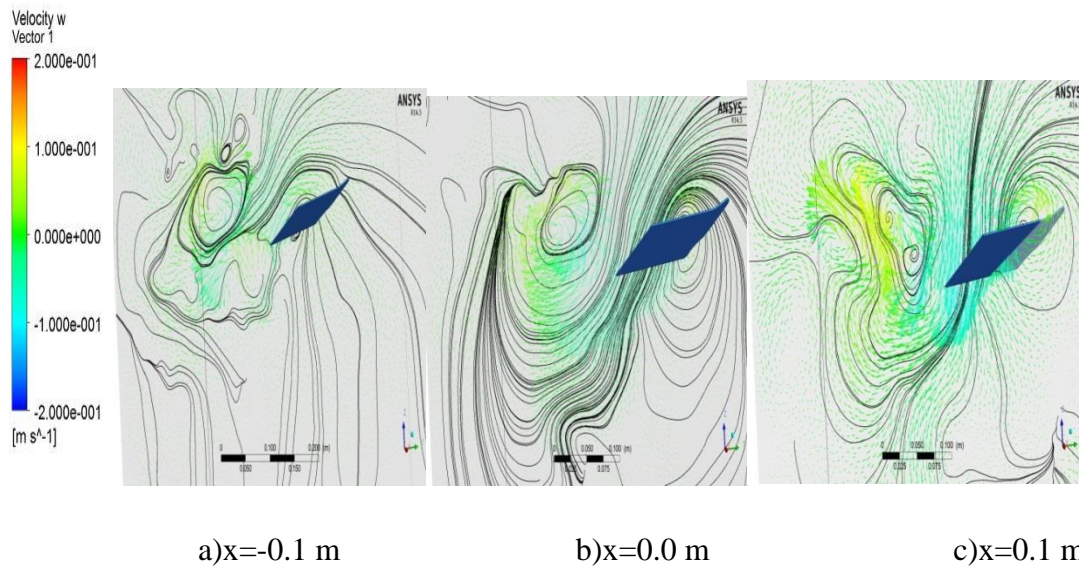
Figure 4.71 :Streamlines and velocity vectors at 30° pitch angle and 60° sweep angle ( t^*=3.2 )
