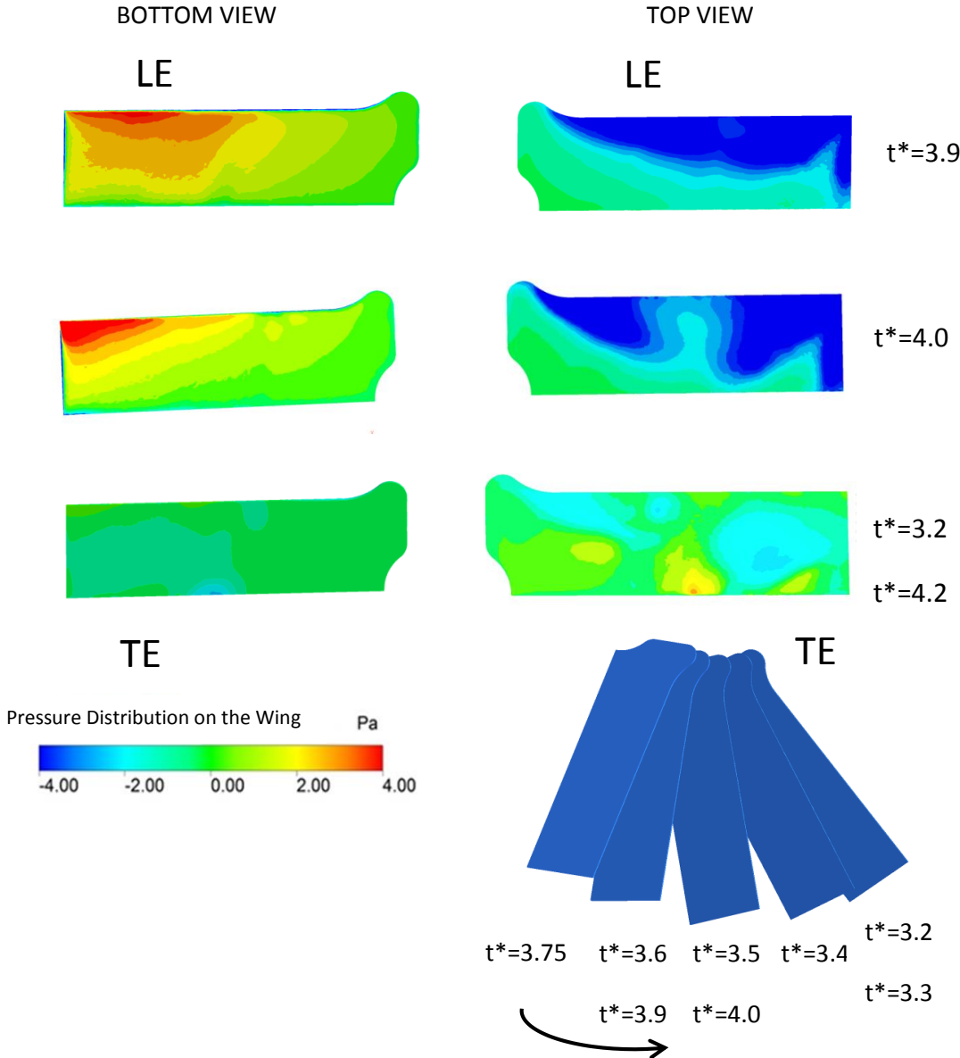
Figure 4.9 Top and bottom views at upstroke of 4th period for Case 2
