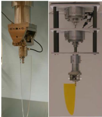
Figure 2. Flapping apparatus and load cell.
