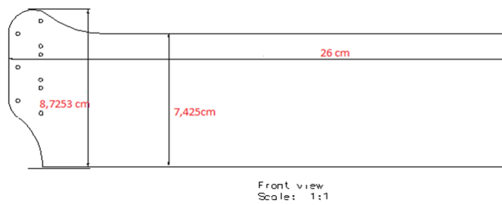
Figure 3.2 : Dimensions of flat plate
