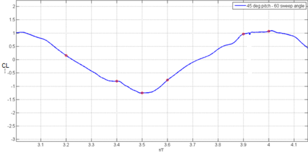
Figure 4.34:Lift coefficient for 4th Period at case 6
