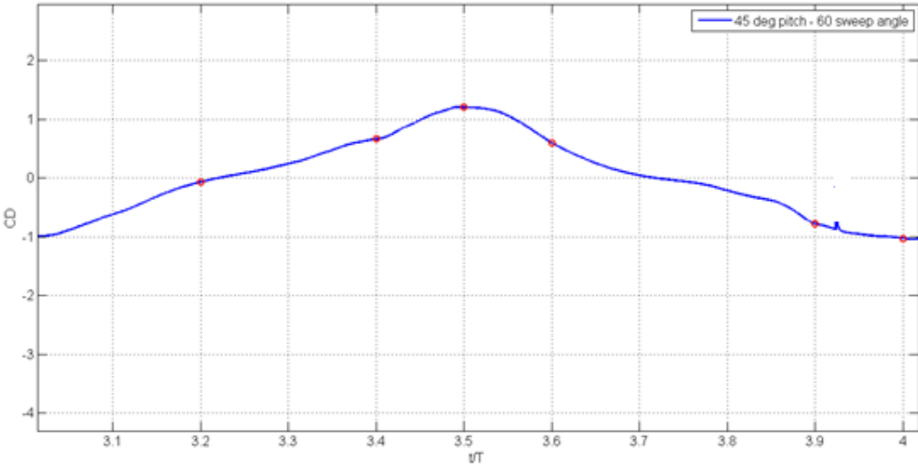
Figure 4.35: Drag coefficient for 4th Period at case 6
