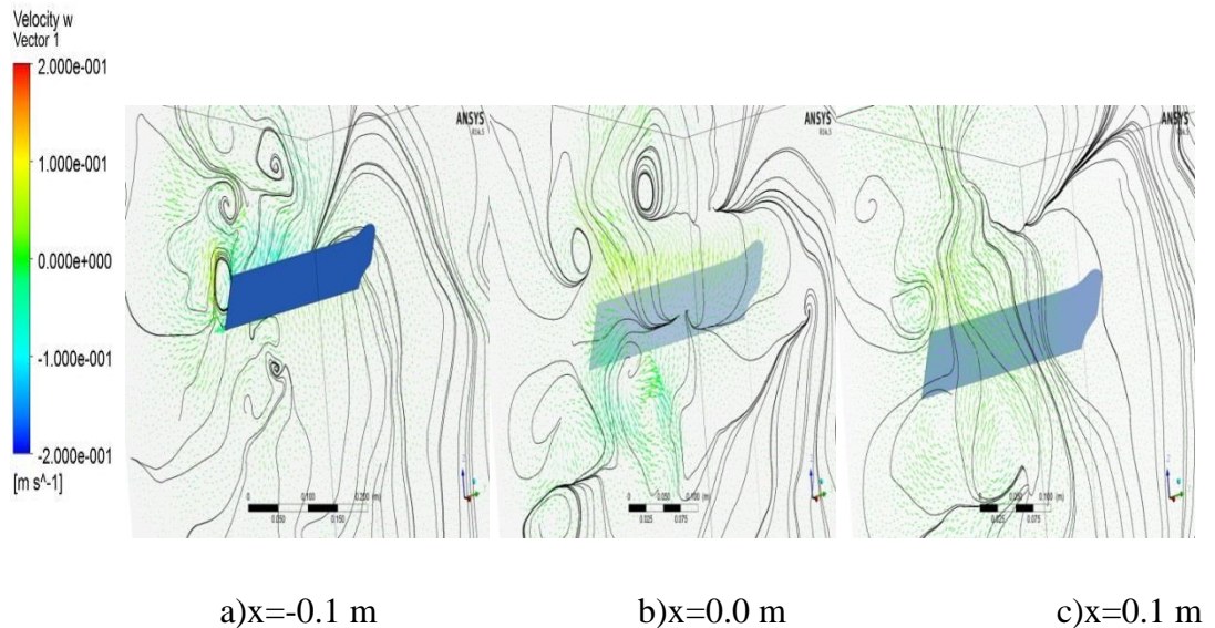
Figure 4.64 :Streamlines and velocity vectors at 45^\circ pitch angle and 30^\circ sweep angle ( t^*=4.0 )
