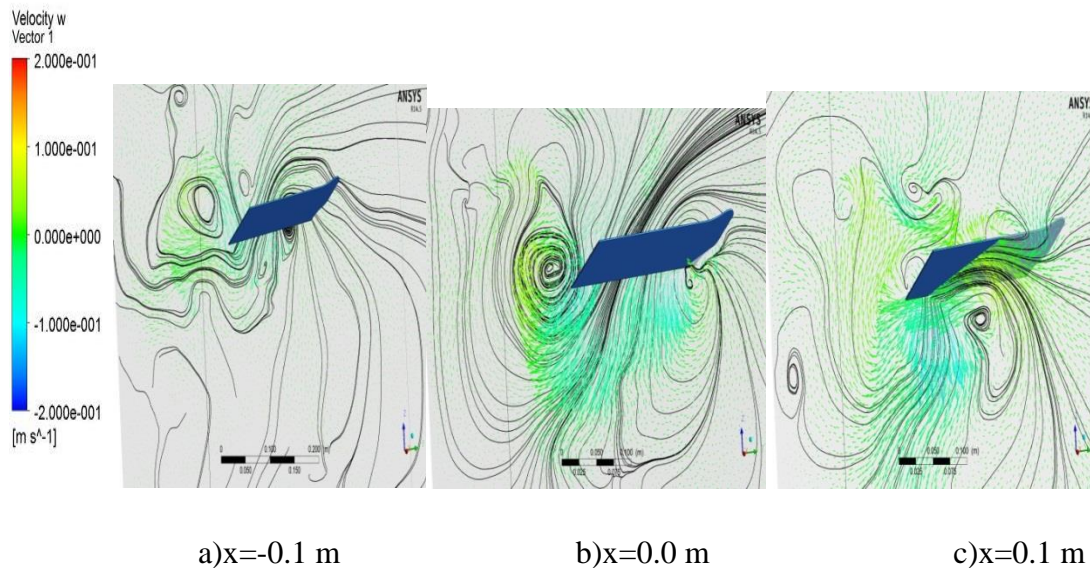
Figure 4.72 :Streamlines and velocity vectors at 30° pitch angle and 60° sweep angle ( t^*=3.4 )
