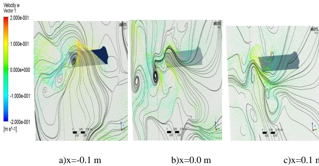
Figure 4.80 :Streamlines and velocity vectors at 45° pitch angle and 60° sweep angle ( t^*=3.6 )
