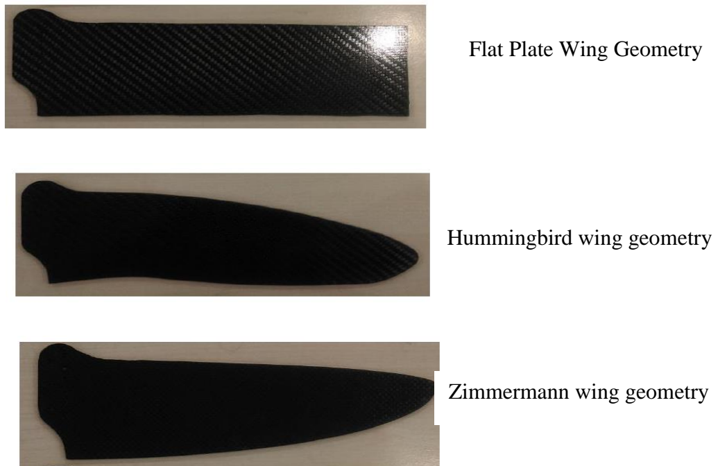
Figure 2.5: Different wing configurations used for experimental method [47]
