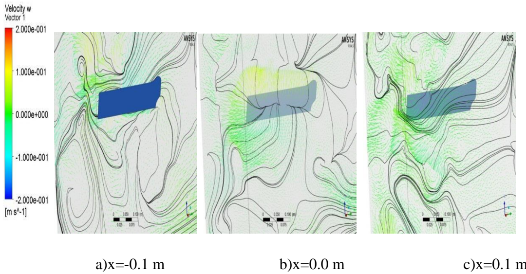
Figure 4.82 :Streamlines and velocity vectors at 45^\circ pitch angle and 60^\circ sweep angle ( t^*=4.0 )
