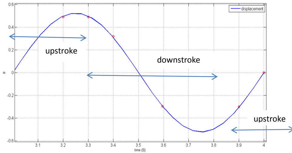
Figure 4.18: Sweeping position for 4th Period at case 3
