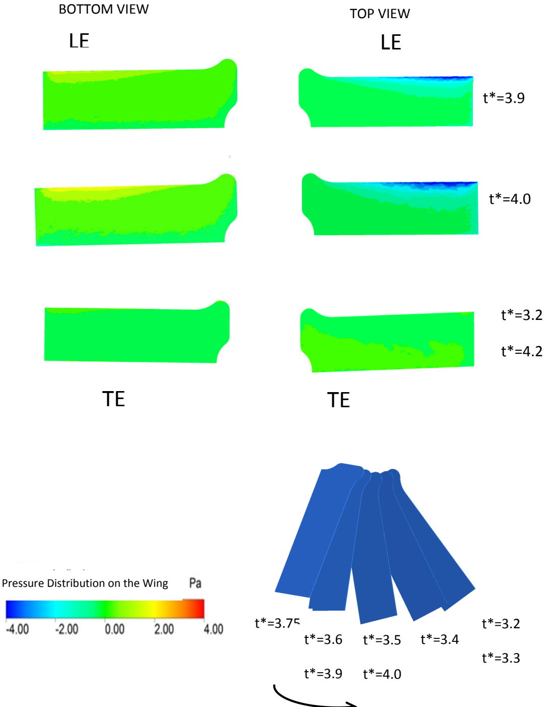
Figure 4.3 Top and bottom views at upstroke of 4th period for Case 1
