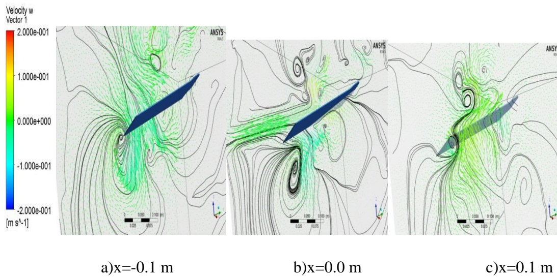
Figure 4.55:Streamlines and velocity vectors at 30^\circ pitch angle and 30^\circ sweep angle ( t^*=3.4 )
