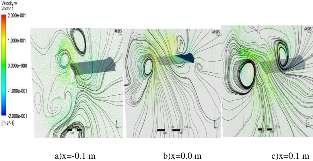
Figure 4.75 :Streamlines and velocity vectors at 30° pitch angle and 60° sweep ( t^*=3.9 )
