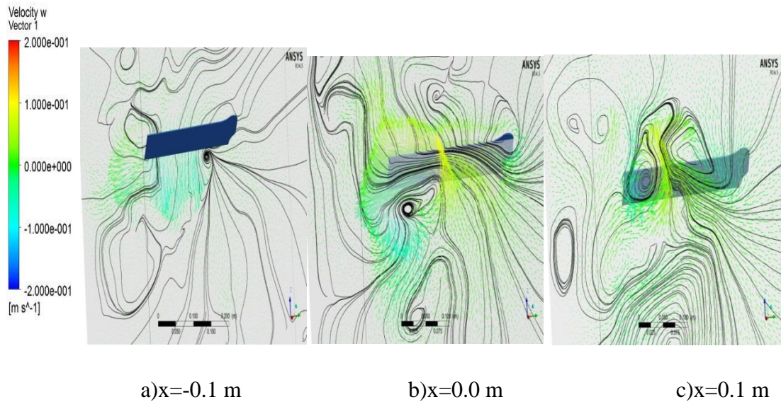
Figure 4.73 :Streamlines and velocity vectors at 30° pitch angle and 60° sweep angle ( t^*=3.5 )
