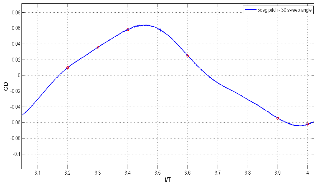
Figure 4.5 Drag coefficient for 4th Period at case 1
