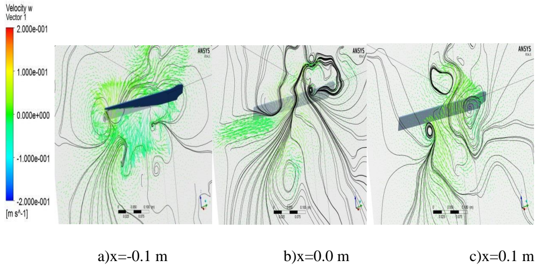
Figure 4.56 :Streamlines and velocity vectors at 30° pitch angle and 30° sweep angle ( t^*=3.6 )
