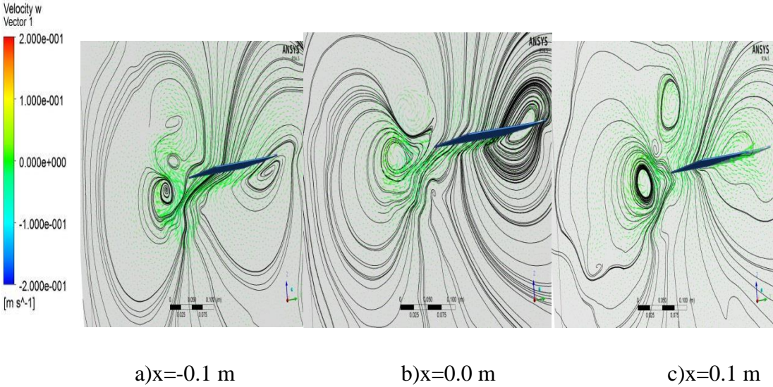
Figure 4.65 :Streamlines and velocity vectors at 5^\circ pitch angle and 60^\circ sweep angle ( t^*=3.2 )
