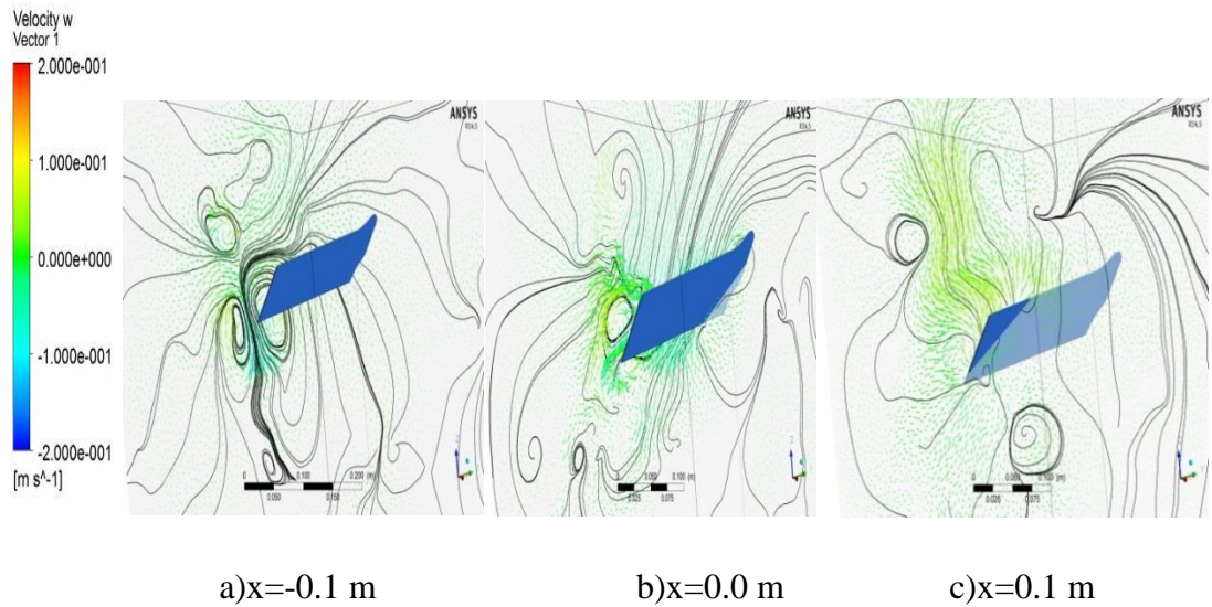
Figure 4.59 :Streamlines and velocity vectors at 45 0 pitch angle and 30 0 sweep angle ( t^*=3.2 )
