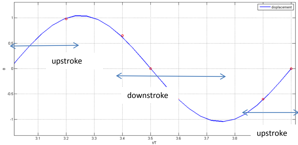
Figure 4.24: Sweeping position for 4th Period at case 4
