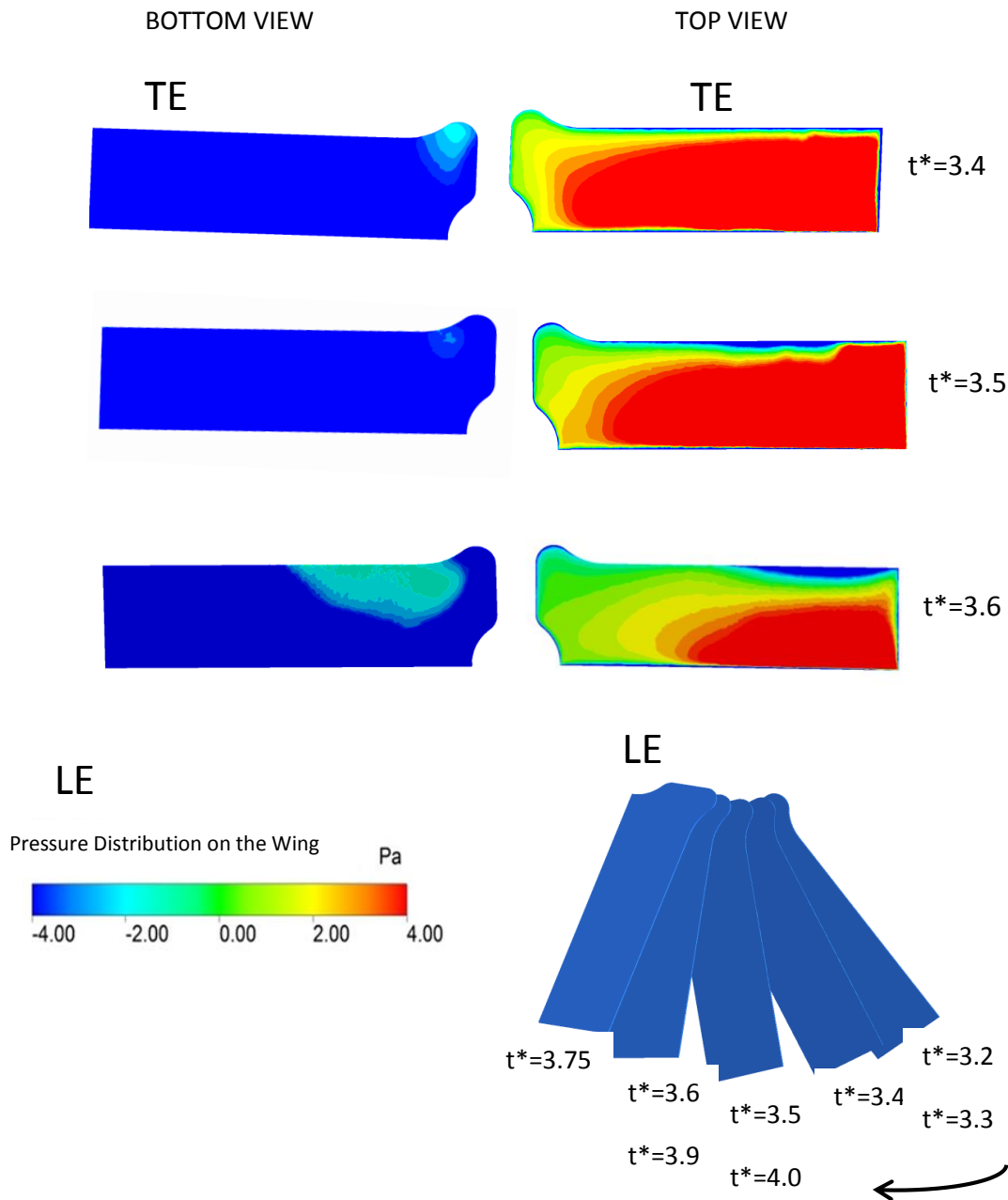
Figure 4.32: Top and bottom views at downstroke of 4th period for Case 6
