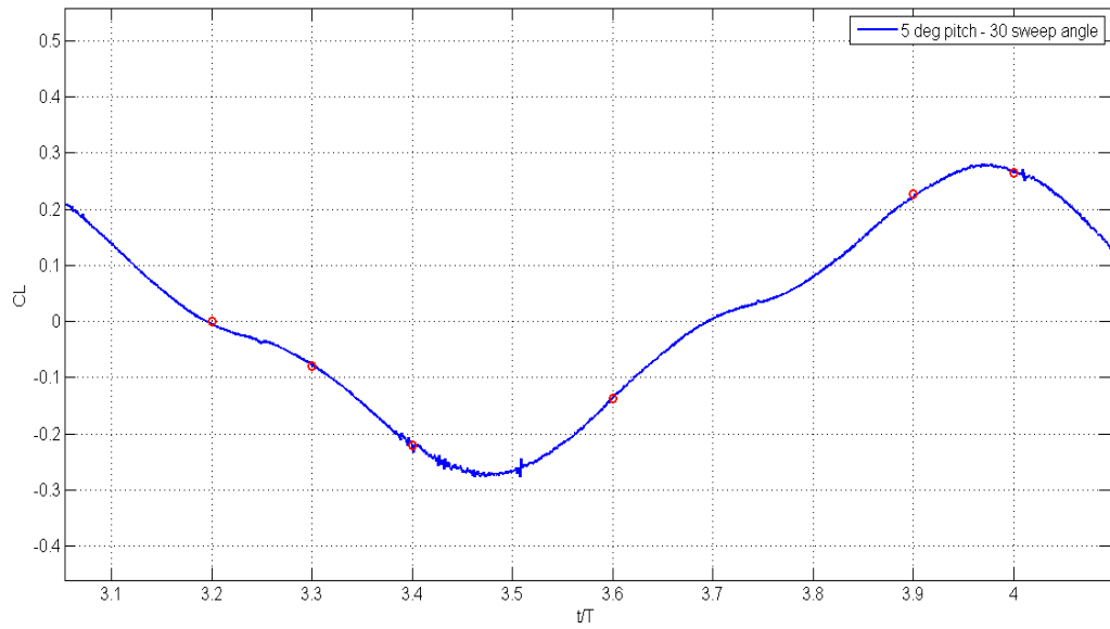
Figure 4.4 Lift coefficient for 4th Period at case 1
