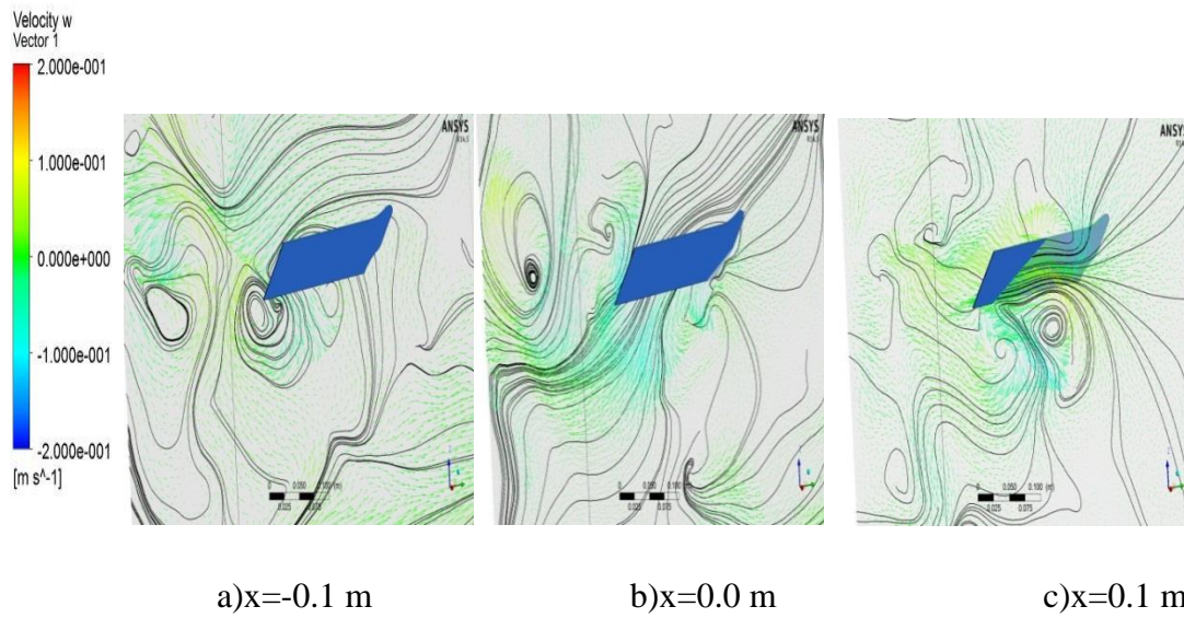
Figure 4.78 :Streamlines and velocity vectors at 45 0 pitch angle and 60 0 sweep angle ( t^*=3.4 )
