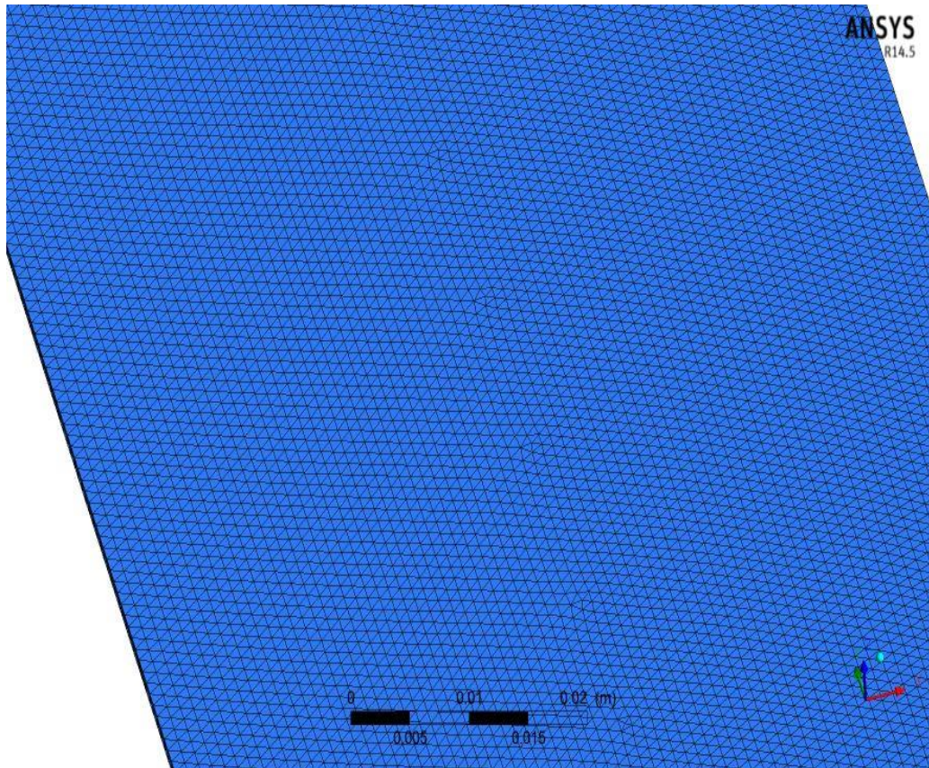
Figure 3.6: Zoom view of the mesh on the wing
