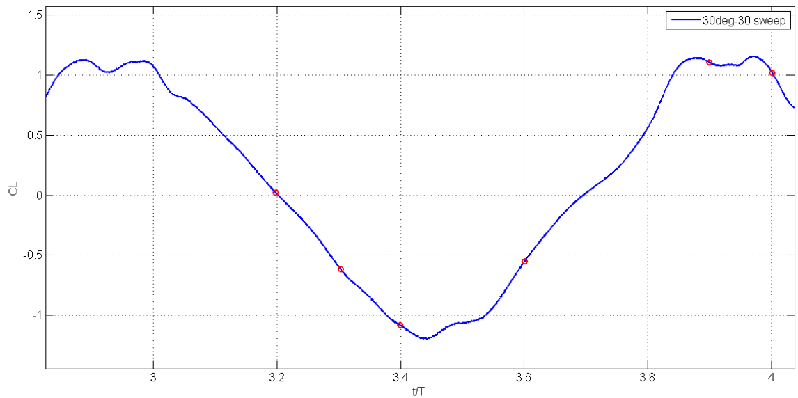
Figure 4.10: Lift coefficient for 4th Period at case 2
