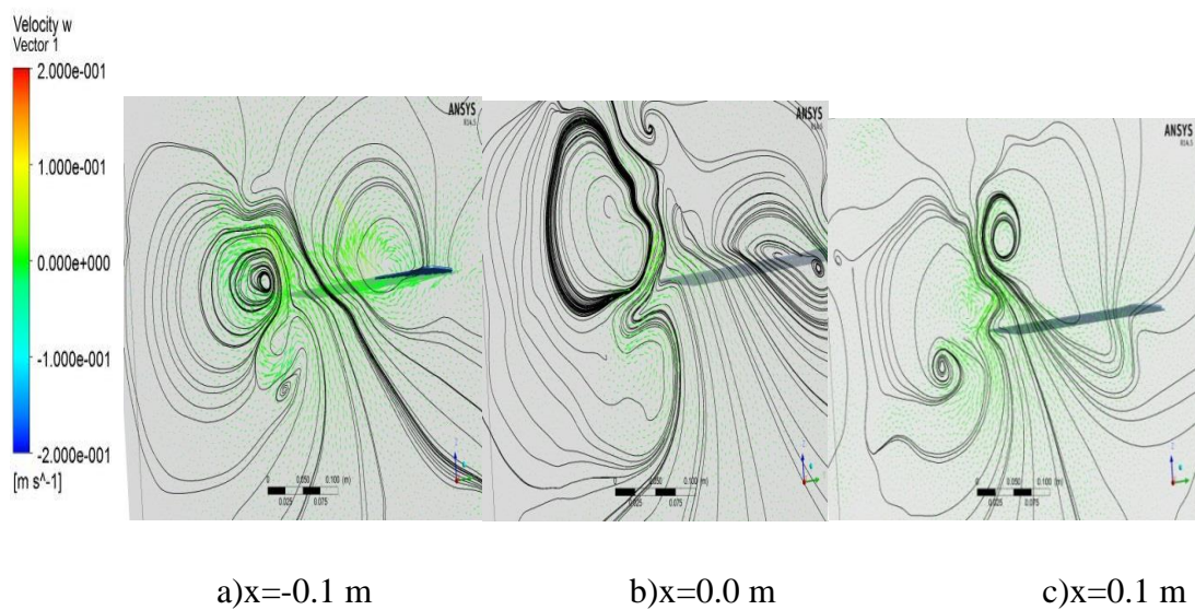
Figure 4.69 :Streamlines and velocity vectors at 5^\circ pitch angle and 60^\circ sweep angle ( t^*=3.9 )
