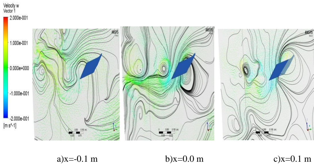
Figure 4.77 :Streamlines and velocity vectors at 45° pitch angle and 60° sweep angle ( t^*=3.2 )
