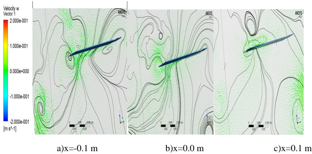
Figure 4.47 :Streamlines and velocity vectors at 5^\circ pitch angle and 30^\circ sweep angle ( t^*=3.2 )
