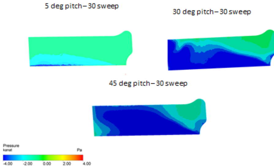
Figure 4.45 Pressure contours at t^*=3.5 (bottom surface)
