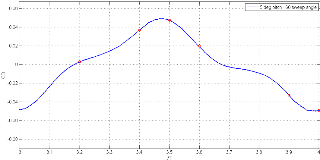
Figure 4.23: Drag coefficient for 4th Period at case 4
