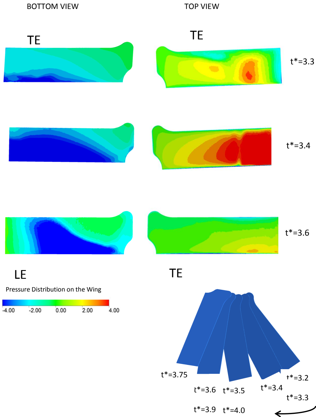
Figure 4.14: Top and bottom views at downstroke of 4th period for Case 3
