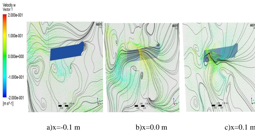
Figure 4.79 :Streamlines and velocity vectors at 45 0 pitch angle and 60 0 sweep angle ( t^*=3.5 )
