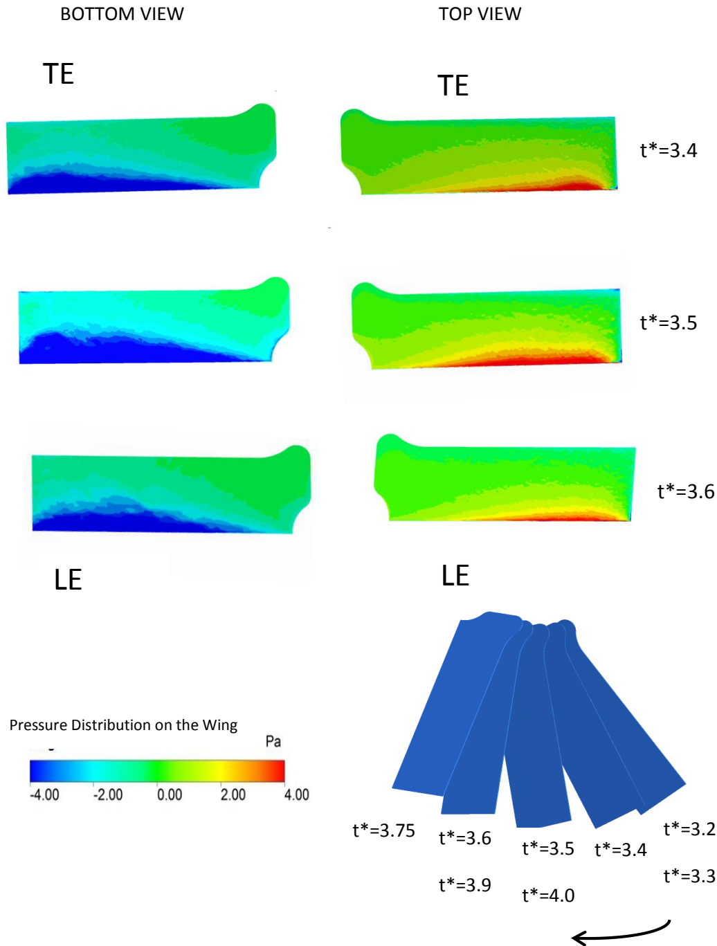
Figure 4.20: Top and bottom views at downstroke of 4th period for Case 4
