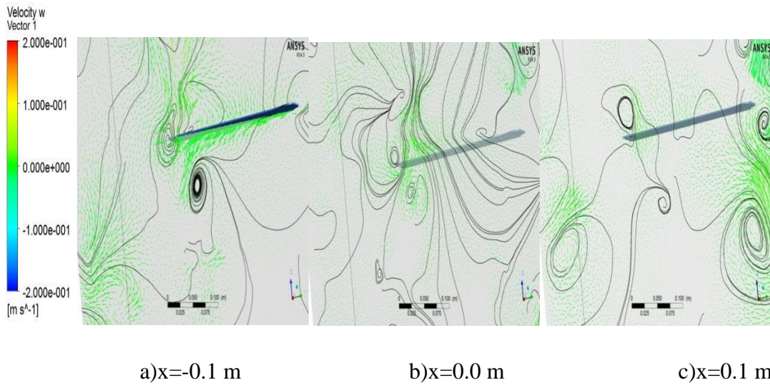
Figure 4.51 :Streamlines and velocity vectors at 5^\circ pitch angle and 30^\circ sweep angle ( t^*=3.9 )
