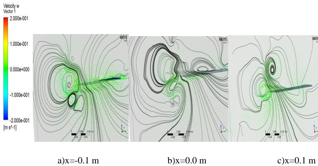
Figure 4.68 :Streamlines and velocity vectors at 5^\circ pitch angle and 60^\circ sweep angle ( t^*=3.6 )
