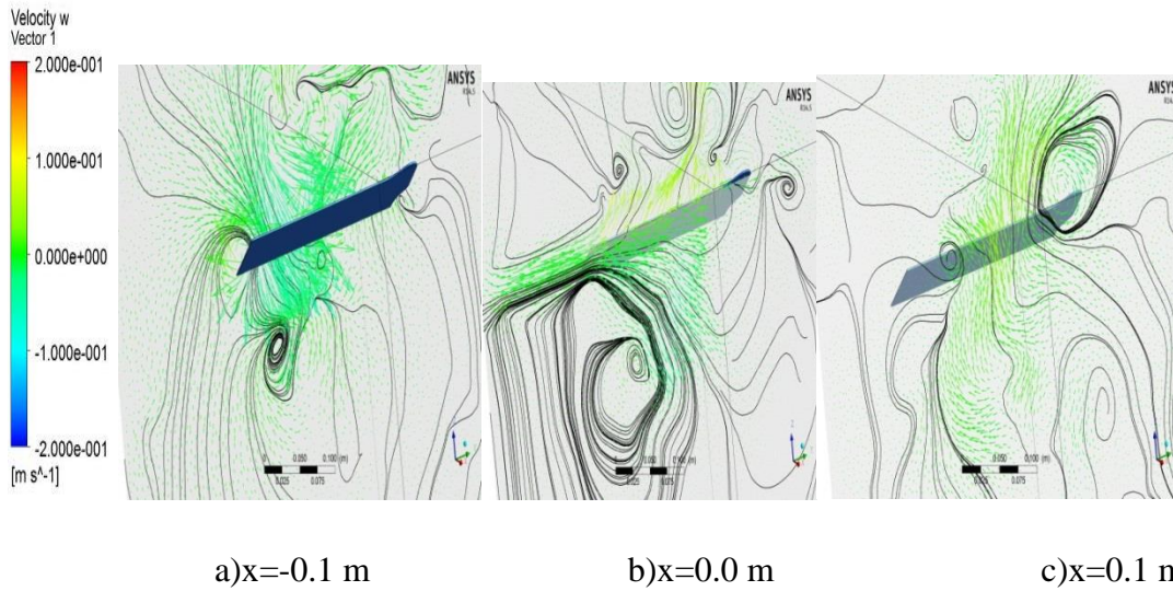
Figure 4.58 :Streamlines and velocity vectors at 30^\circ pitch angle and 30^\circ sweep angle ( t^*=4.0 )
