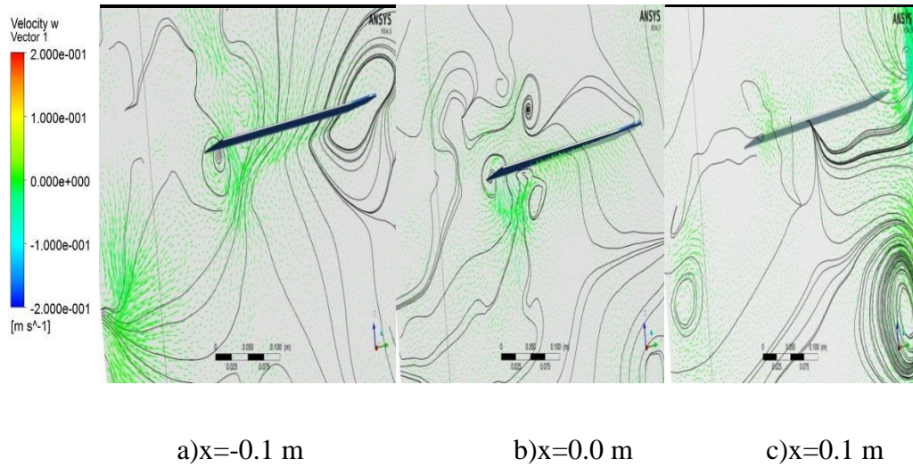
Figure 4.49 :Streamlines and velocity vectors at 5^\circ pitch angle and 30^\circ sweep angle ( t^* = 3.4 )
