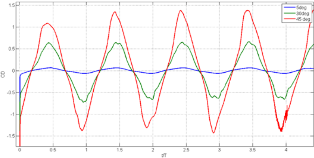
Figure 4.38: Drag coefficients at 30 deg sweep angle (blue:5deg,green:30deg,red:45deg)
