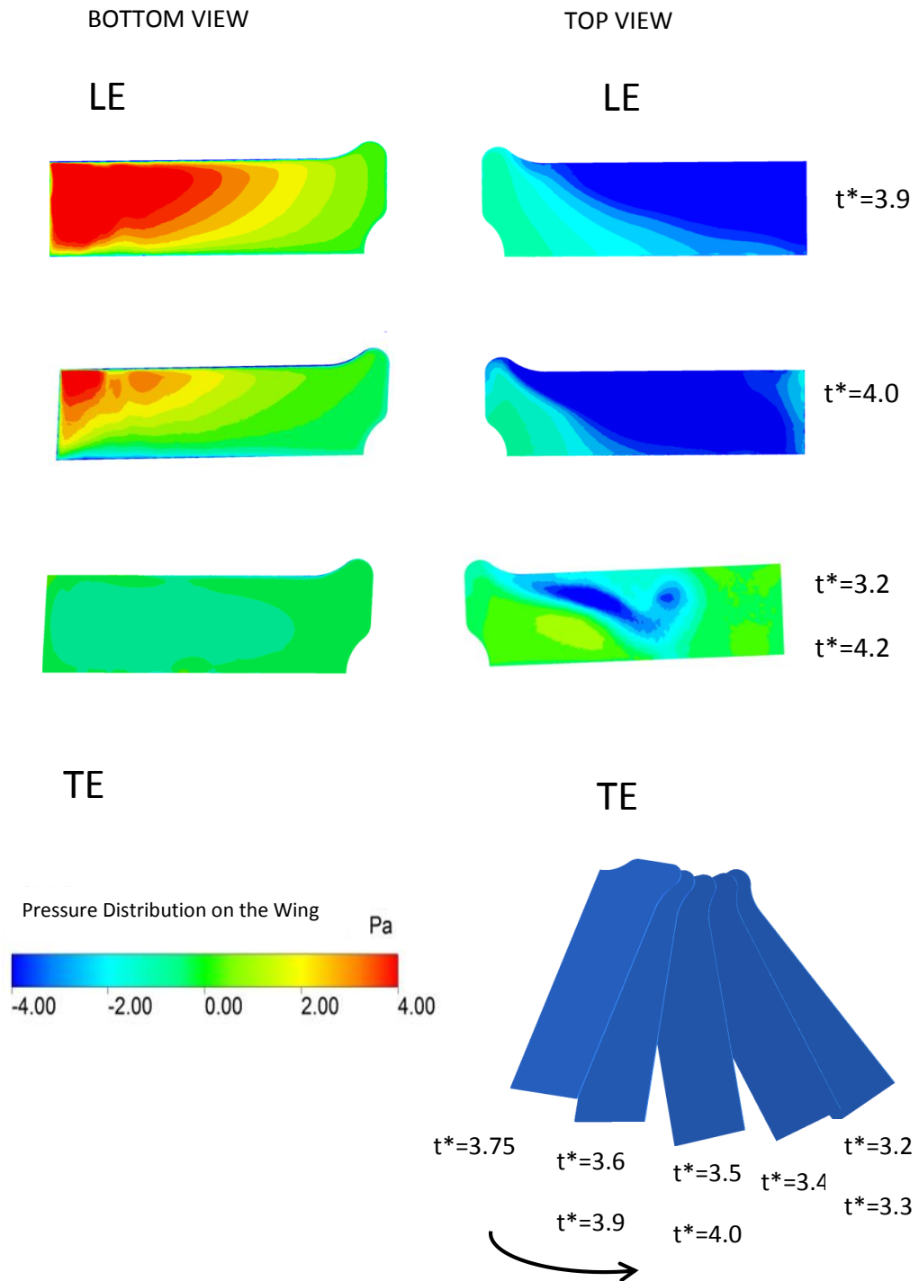
Figure 4.15: Top and bottom views at upstroke of 4th period for Case 3
