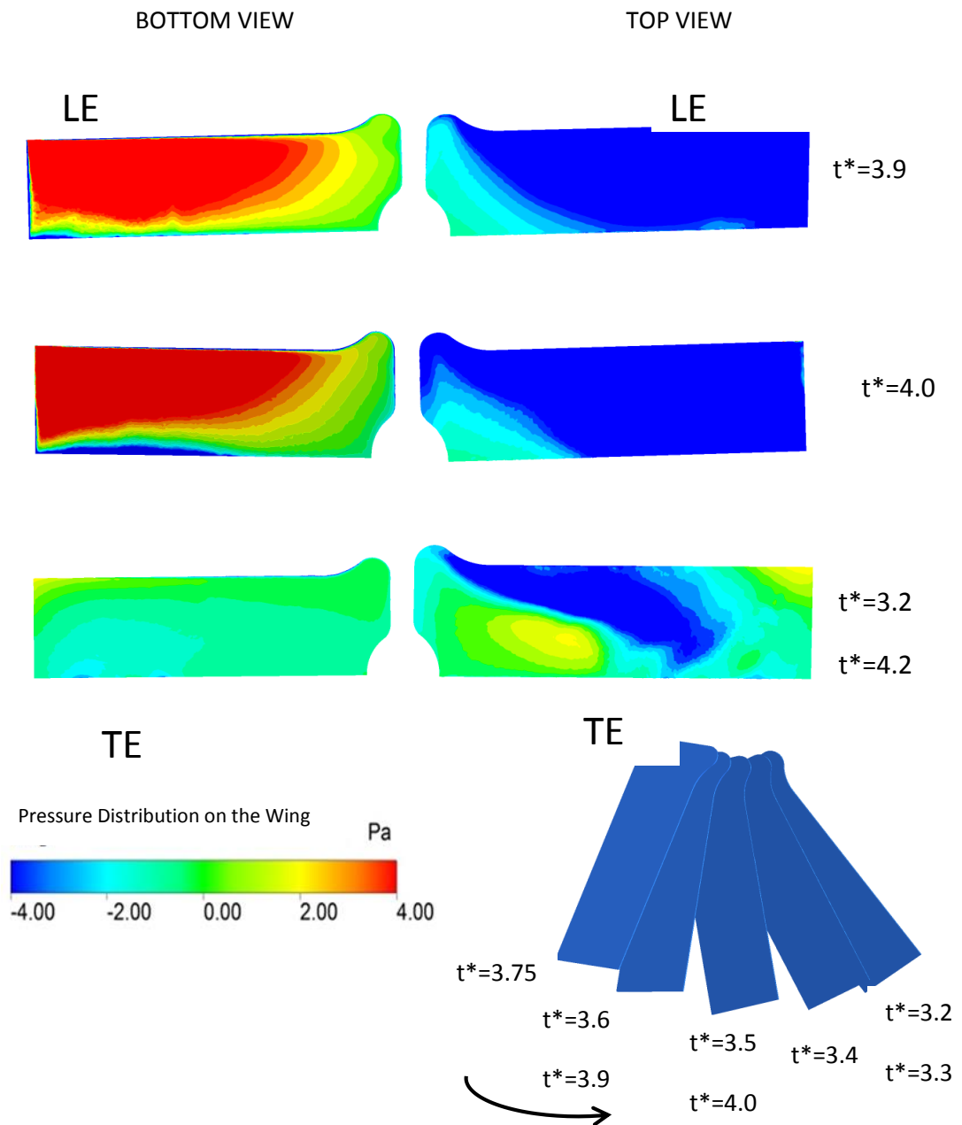
Figure 4.27: Top and bottom views at upstroke of 4th period for Case 5
