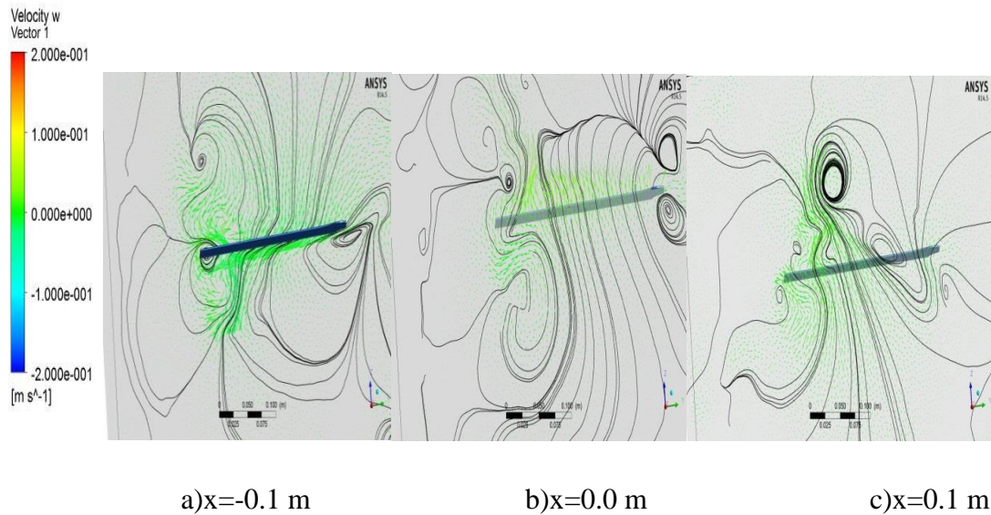
Figure 4.70 :Streamlines and velocity vectors at 5^\circ pitch angle and 60^\circ sweep angle ( t^*=4.0 )
