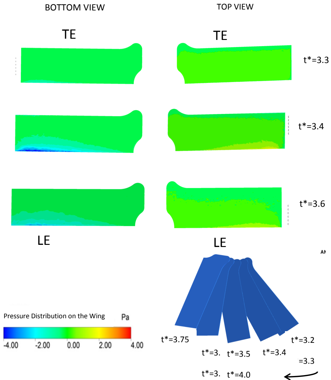
Figure 4.2: Top and bottom views at downstroke of 4th period for Case 1
