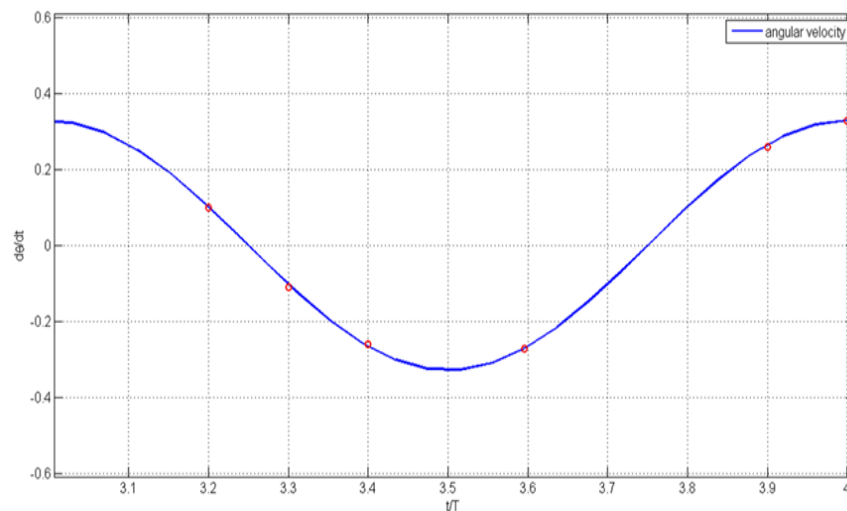
Figure 4.19: Sweeping velocity for 4th Period at case 3
