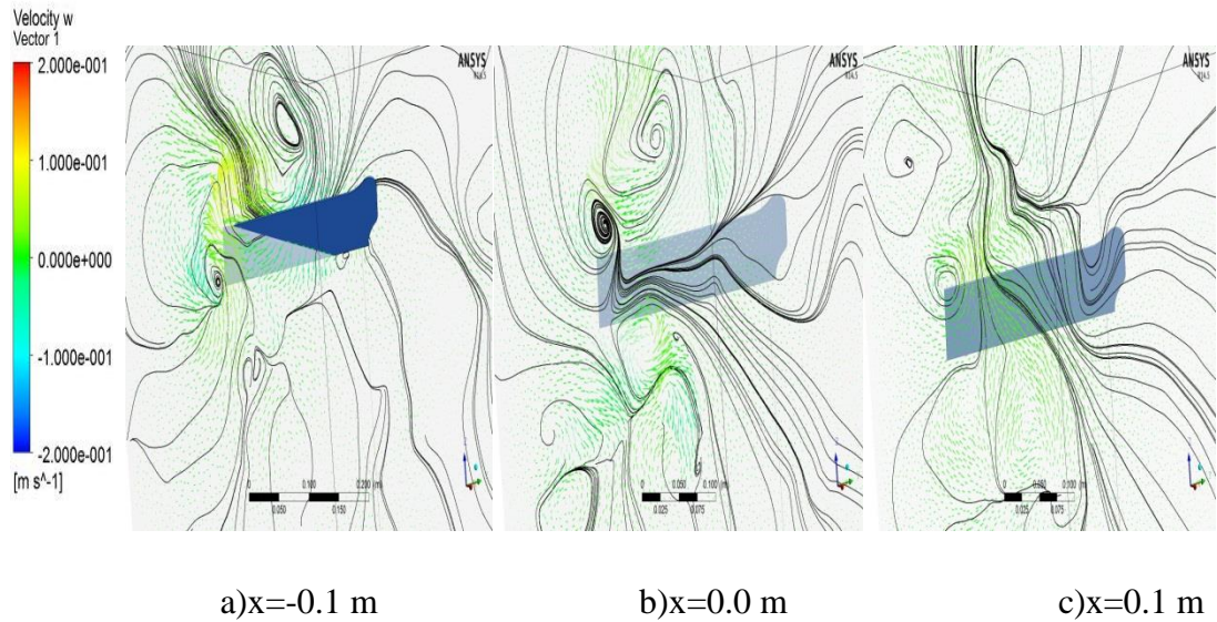
Figure 4.63 :Streamlines and velocity vectors at 45^\circ pitch angle and 30^\circ sweep angle ( t^*=3.9 )
