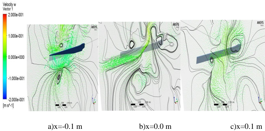
Figure 4.57 :Streamlines and velocity vectors at 30° pitch angle and 30° sweep angle ( t^*=3.9 )
