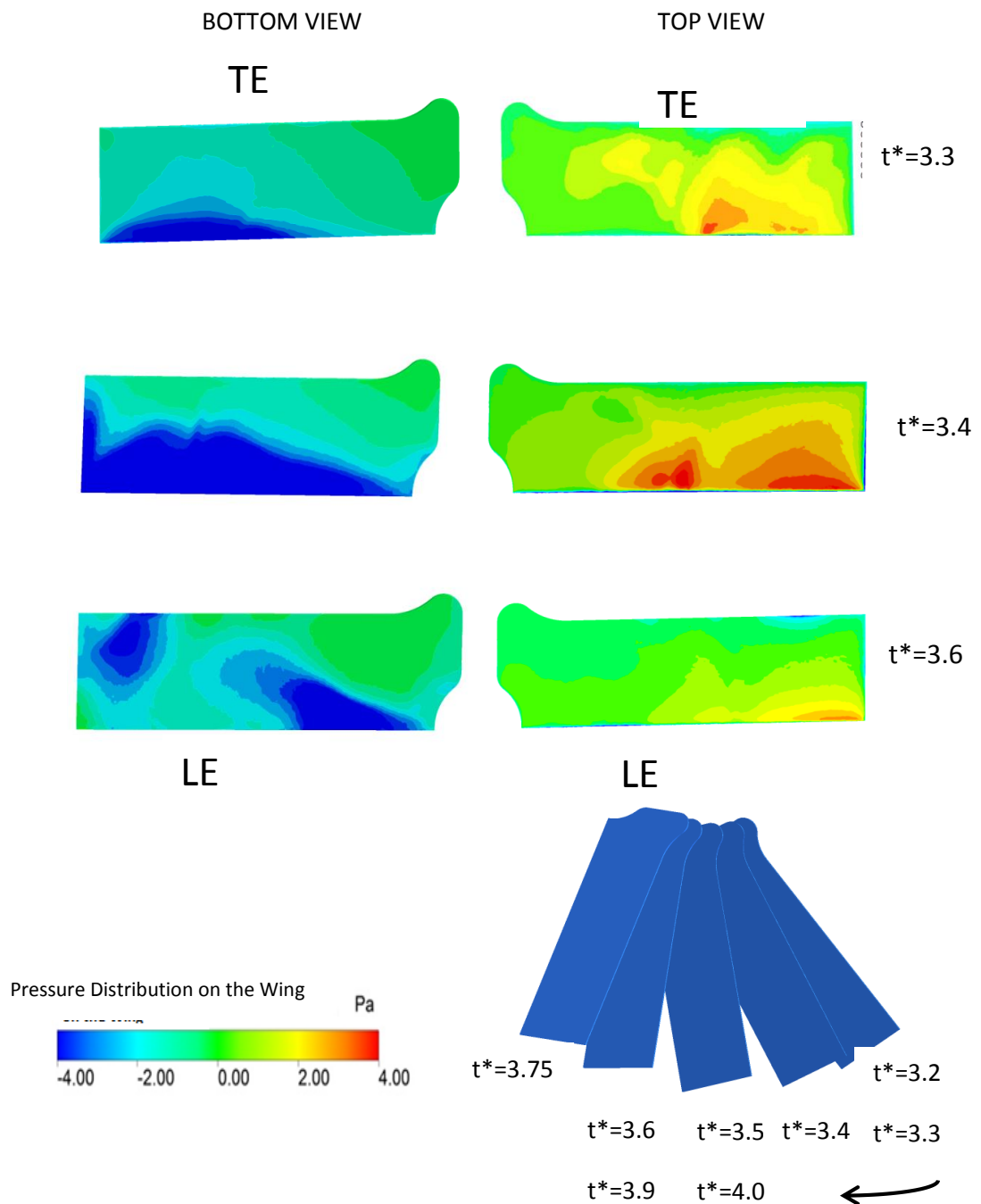
Figure 4.8 Top and bottom views at downstroke of 4th period for Case 2
