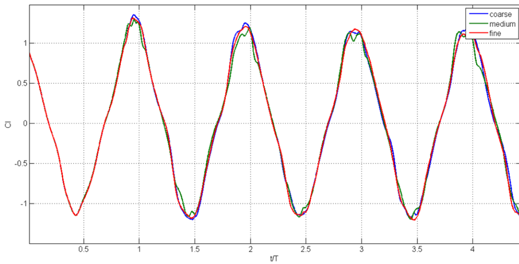
Figure 3.12 : Lift coefficient for coarse . medium and fine mesh studies
