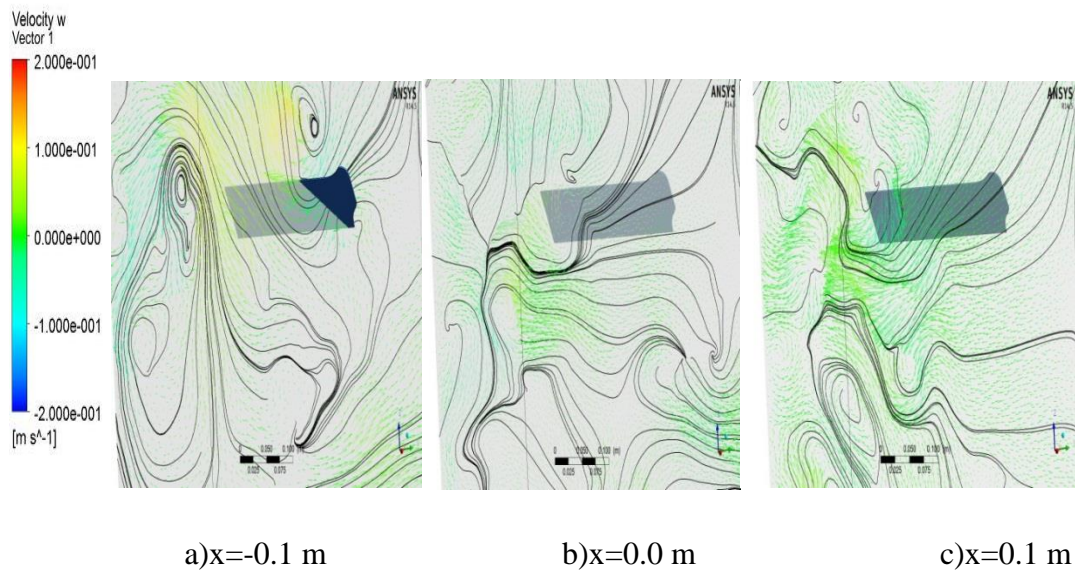
Figure 4.81 :Streamlines and velocity vectors at 45° pitch angle and 60° sweep angle ( t^*=3.9 )
