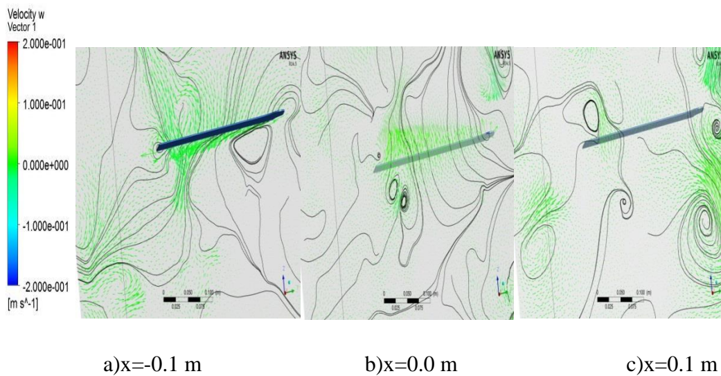
Figure 4.52:Streamlines and velocity vectors at 5^\circ pitch angle and 30^\circ sweep angle ( t^*=4.0 )
