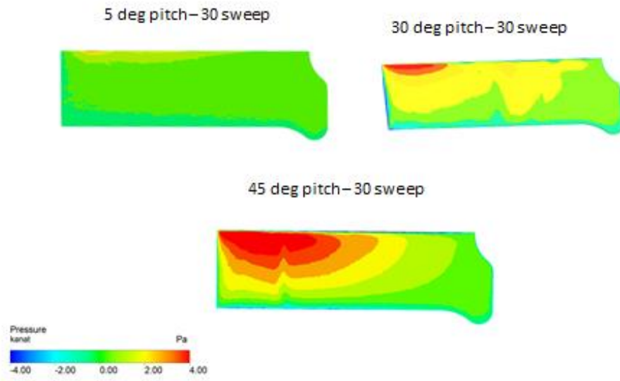
Figure 4.44 Pressure contours at t^*=3.5 (top surface)
