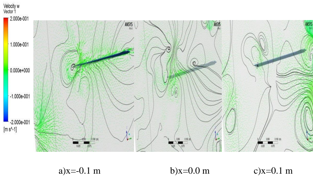
Figure 4.50 :Streamlines and velocity vectors at 5^\circ pitch angle and 30^\circ sweep angle ( t^* = 3.6 )
