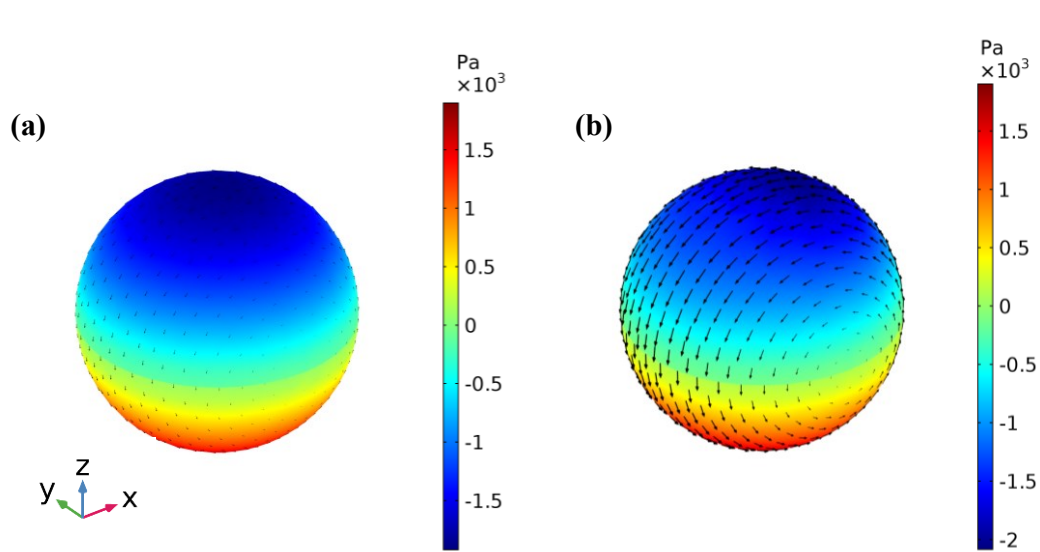
Figure 4.15. z-components of stress distribution on the spherical particle travelling at different lateral positions in a circular channel. (a) The stress distribution at a position (0,0.1h). (b) The stress distribution at (0,0.7h).
