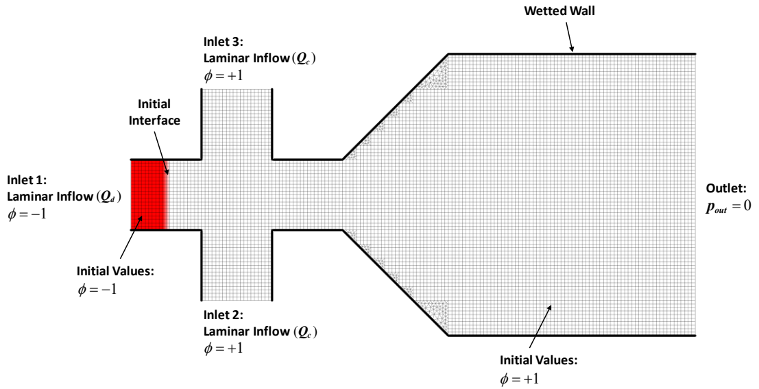
Figure 3.4. Mesh details and boundary conditions used in 2D COMSOL model.
