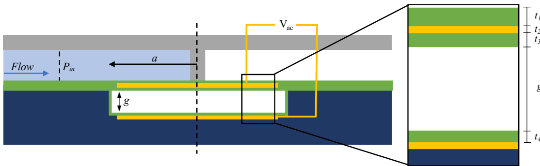
Figure 6.4. Geometric parameters involved in the design of the microvalves.
