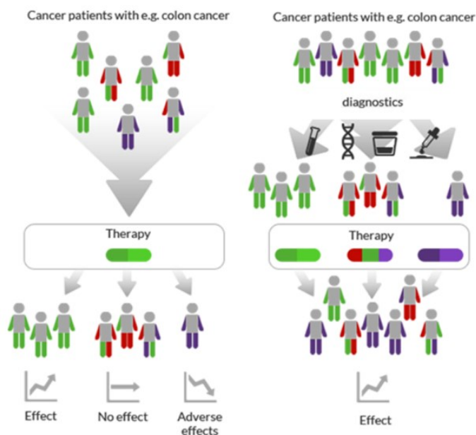
Figure 1.3. Personalized chemotherapy [27].
