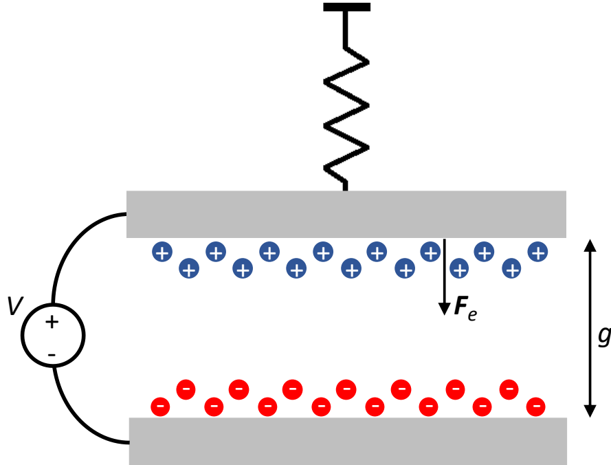
Figure 6.5. Schematic illustration of the parallel-plate approach.
