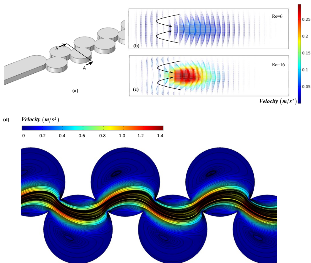
Figure 2.9. Formation of Dean vortices in the proposed CEA micromixer. (a) Cross-section. (b) and (c) Simulation results which are illustrated for Re=6 ( 45 \mu\text{l}/\text{min} ) and Re=16 ( 120 \mu\text{l}/\text{min} ). (d) Formation of expansion vortices at Re=20 . The formation of these vortices facilitates mixing of species at respectively high Reynolds numbers.
