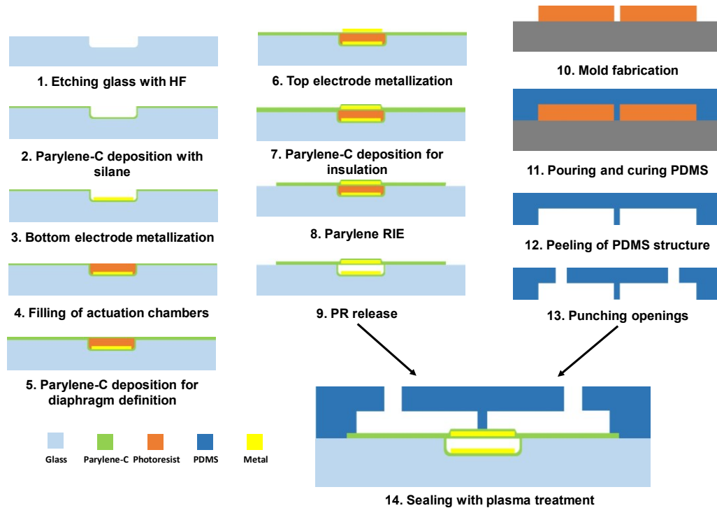
Figure 7.2. Fabrication flow schematic cross-section diagram. The structures are not drawn actual layout dimensions.
