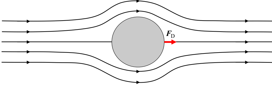
Figure 4.3. Schematic illustration of viscous drag force.
