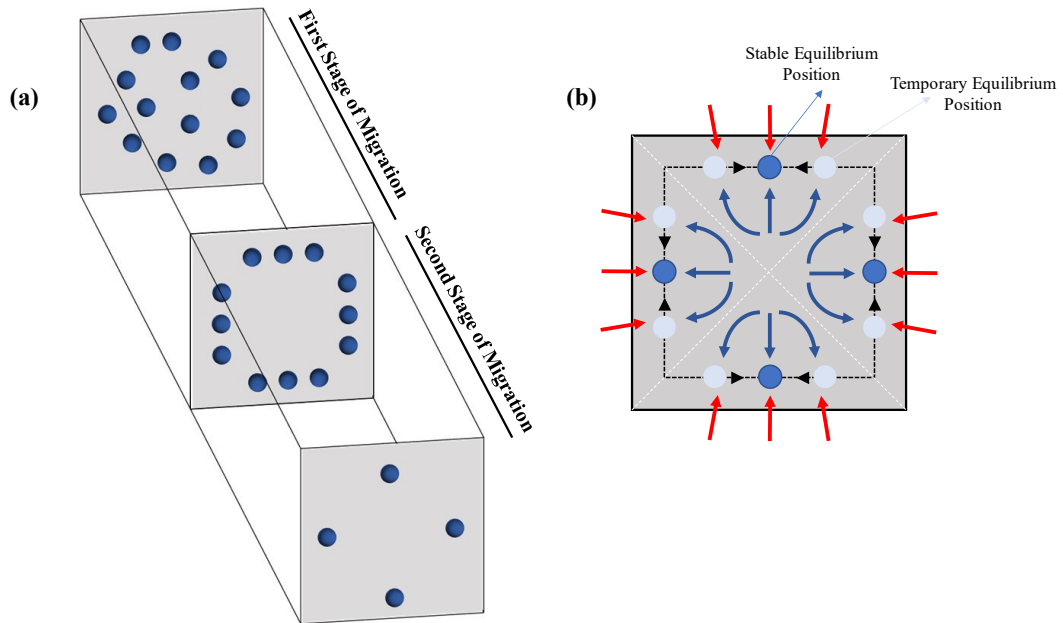
Figure 4.10. Inertial focusing in a square microchannel. (a) Two stages of lateral migration. (b) Stable and temporary equilibrium locations obtained under the effect of lift forces.
