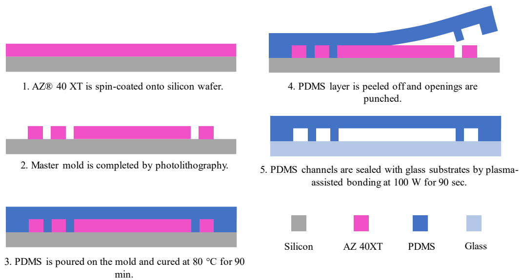
Figure 5.2. Schematic showing fabrication steps of PDMS devices actualized by soft lithography.
