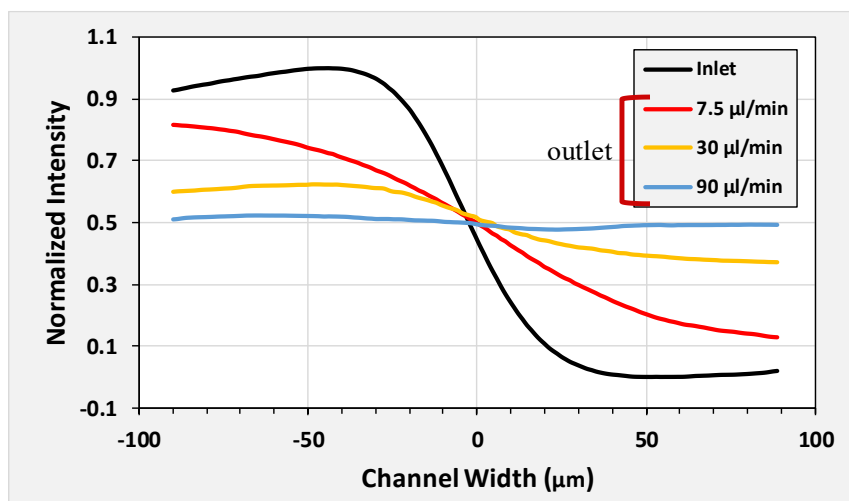
Figure 5.5. Normalized intensity values indicating species concentration at the entrance and the exit of the micromixer based on the fluidic experiments.
