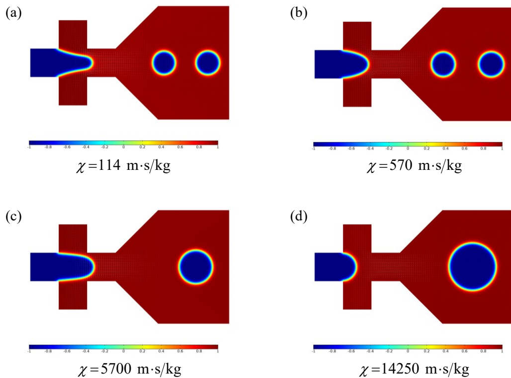
Figure 3.7. The 2D schematics of droplet break-up numerically calculated for four different values of mobility (a-d). The interfacial parameter is fixed to 0.05L . The flow rates of dispersed and continuous phases are 5 \mu\text{l}/\text{min} and 30 \mu\text{l}/\text{min} , respectively. The white arrows indicate the direction of the flow.
