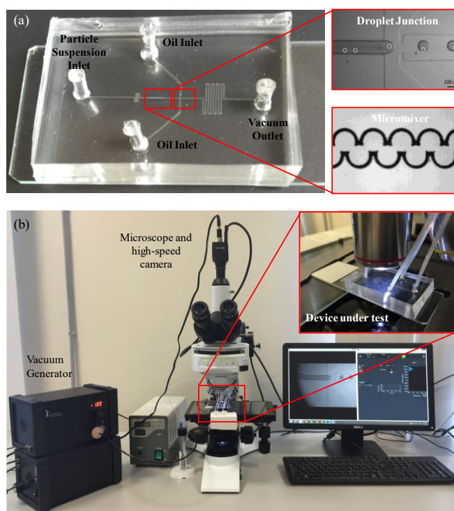
Figure 5.15. Single cell encapsulation experiments. (a) PDMS test device. (b) Experimental setup.
