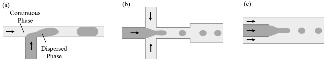
Figure 3.1. Typical passive droplet generation strategies. (a) T-junction microchannel. (b) Flow-focusing microchannel. (c) Co-flow type microchannel.
