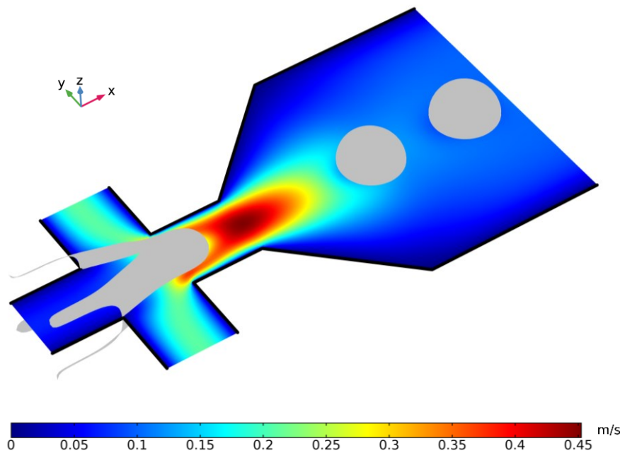
Figure 3.5. COMSOL Simulation of droplet generation in a 3D flow-focusing junction. The flow rates of dispersed and continuous phases are 5 \mu\text{l}/\text{min} and 30 \mu\text{l}/\text{min} , respectively. Surface plot represents the velocity field and the contour plot depicts the interfacial film.
