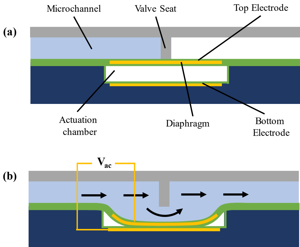
Figure 6.3. The structure of electrostatic microvalve and operation states. (a) Closed state. (b) Open State.
