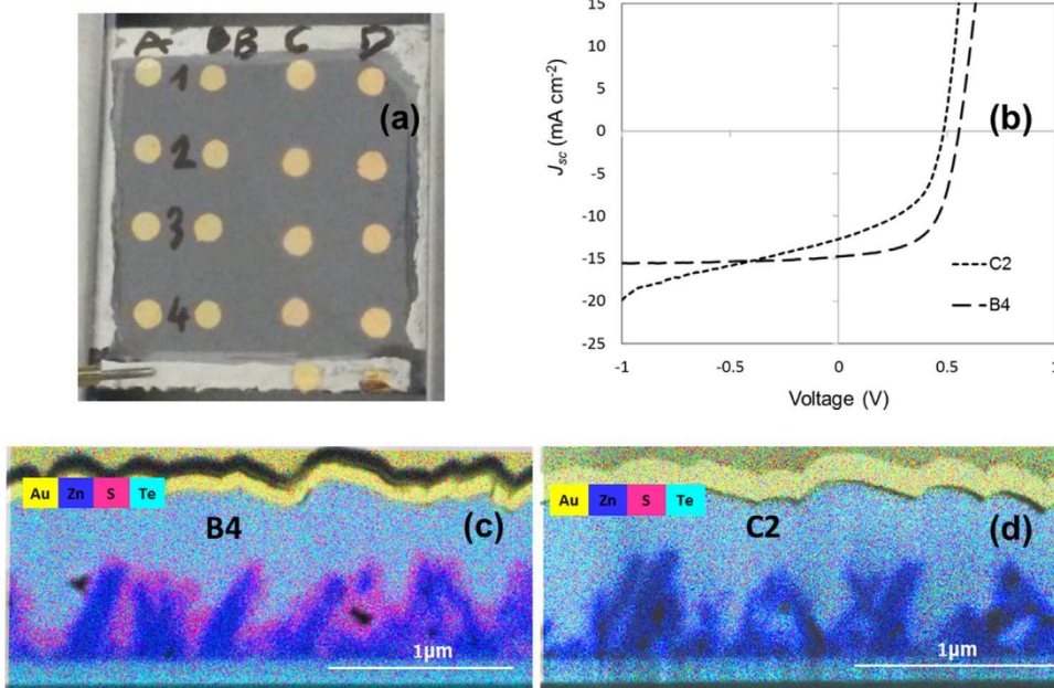
Fig. 7. A typical 2.5 \times 2.5 \text{ cm}^2 CdTe/CdS/ZnO NRs device with 2 mm diameter dot contacts (a), light J - V curves (b) and cross-sectional EDS elemental (Au, Zn, S, and Te) maps (c, d) for selected cells (B4, C2). ZnO NRs in cell B4 have a CdS coating whereas those in C2 has little/or no CdS coverage. The ZnO NRs are embedded in a relatively thick CdTe layer electrically separating the Au contact.
