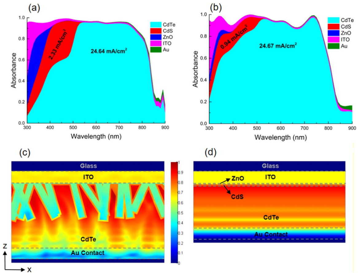
Fig. 6. The absorption spectra in each layer for (a) NR-based and (b) planar cells. The corresponding solar spectrum weighed normalized absorption profiles are given for (c) NR-based cells and (d) planar cells.
