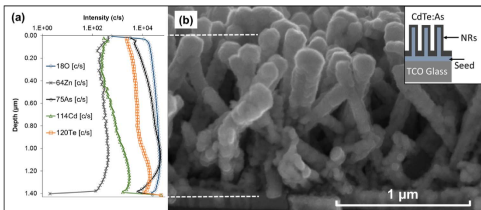
Fig. 5. SIMS depth profiles of the Zn^{64} , O^{18} , Cd^{114} , Te^{120} , and As^{75} isotopes (a) and a cross-sectional SEM image (b) for a CdTe:As coated ZnO NR array with rod length of \sim 1.4 \mu\text{m} .
