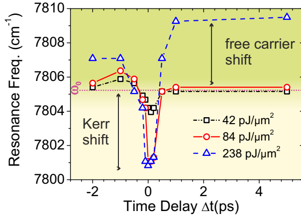
FIG. 4: (color online) Resonance frequency versus time delay ( \Delta t ) between pump and probe at different pump pulse energies. The resonance frequency red-shifts due to the instantaneous electronic Kerr effect only at temporal overlap ( \Delta t = 0 \pm 15 \text{ fs} ) of pump-probe (shaded with bright color). The blue shift of the cavity resonance due to free carriers is observed when the pump pulse energy is increased (shaded with dark color). The dotted horizontal line shows the unswitched resonance frequency at \omega_0 = 7805.6 \text{ cm}^{-1}
