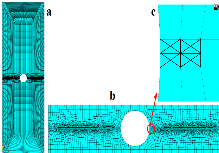
Figure 4. a) Meshed model using Mesh#2 b) Enrichment field c) Initial crack definition in XFEM
