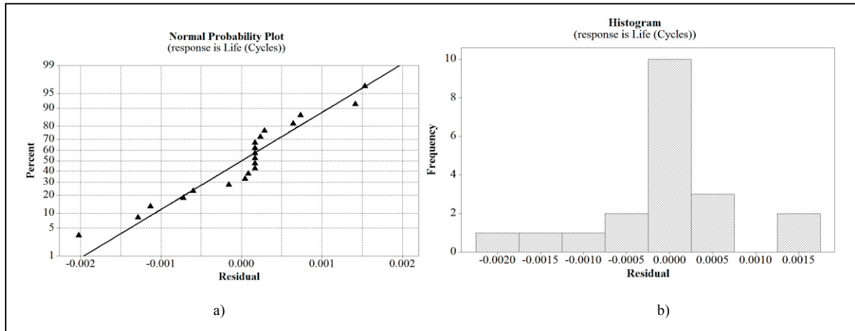
Figure 6. a) Normal Probability Plot. b) Residuals Histogram
