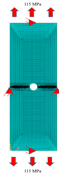
Figure 3. Modelled geometry for the XFEM analysis
