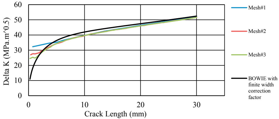
Figure 5. Comparison of XFEM mesh sensitivity
