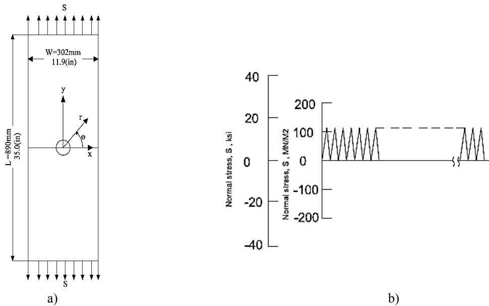
Figure 1. a) Experimental Specimen b) Loading Condition in the experimental tests [1]
