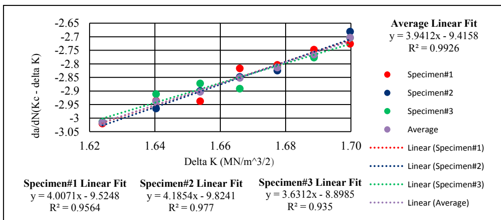
Figure 2. Linear Fit of the Experimental Data on LOG-LOG Scale
