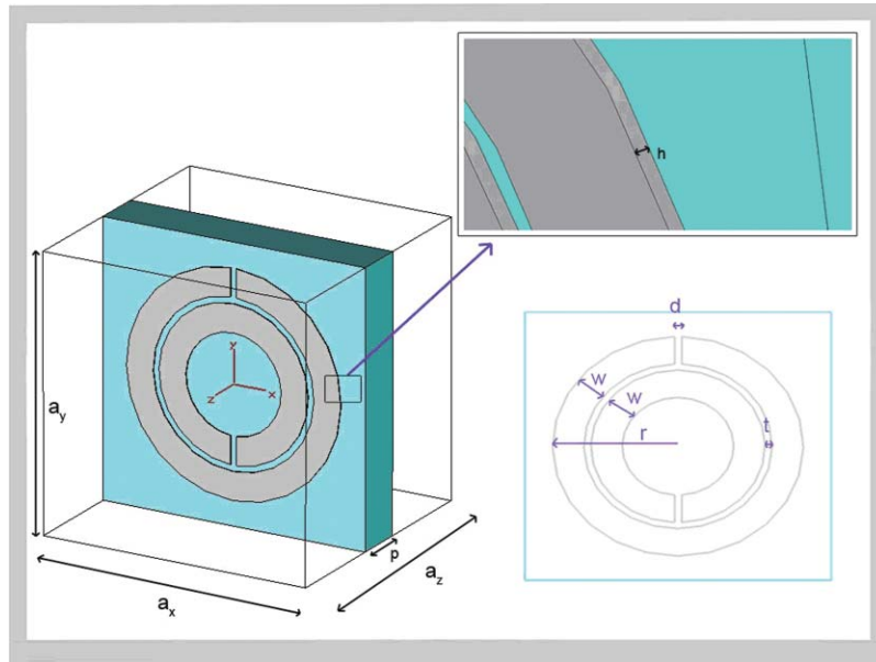
Fig. 1 Unit cell of the SRR structure.
