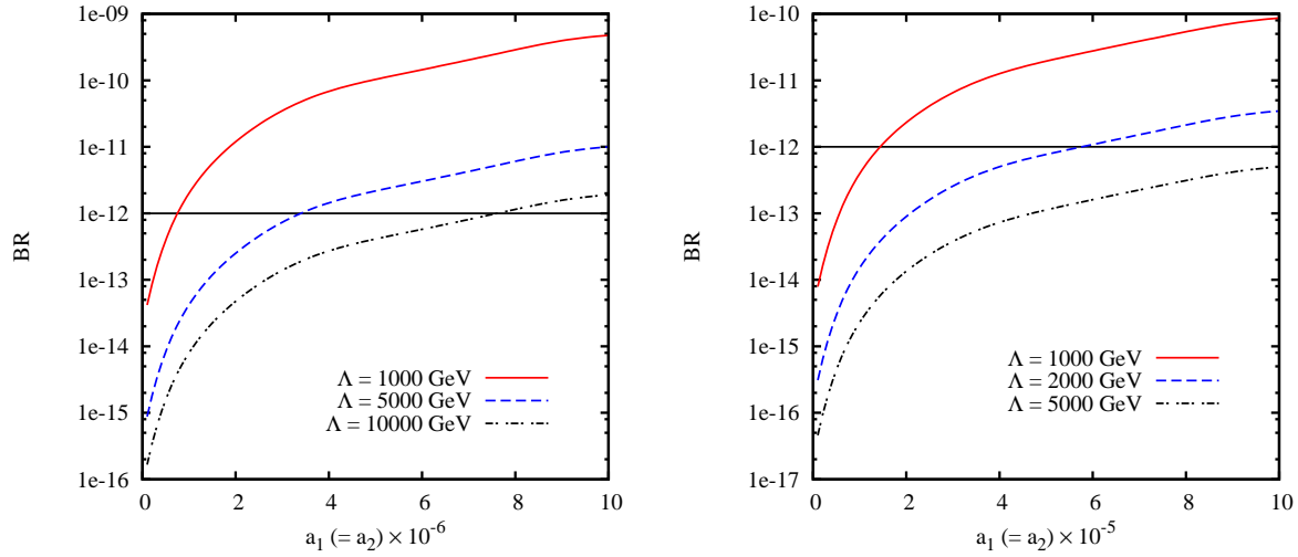
Figure 3: Variation of the branching ratio with a_1(= a_2) for various values of \Lambda_{\mathcal{U}} . The other parameters are (a) Left panel: a_3 = a_4 = 0.001 and d_{\mathcal{U}} = 1.6 , (b) Right panel: a_3 = a_4 = 0.01 and d_{\mathcal{U}} = 1.8 .
