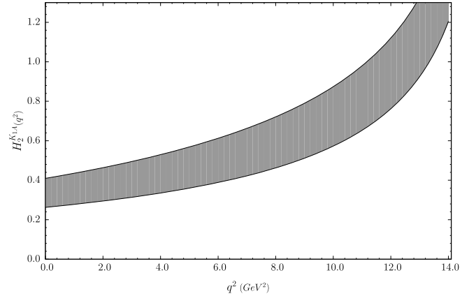
Fig. 3. The same as in Fig. 1, but for the helicity amplitude H_2(q^2) .
