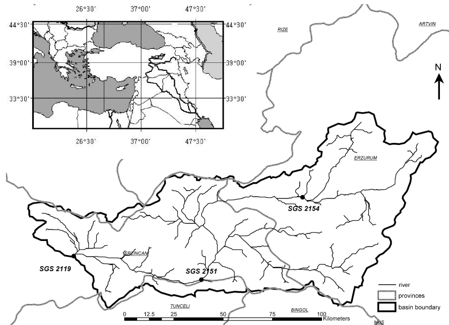
Fig. 1. Location of Karasu Basin (upper Euphrates River) in Turkey and stream gauging stations (SGS) in the basin.
