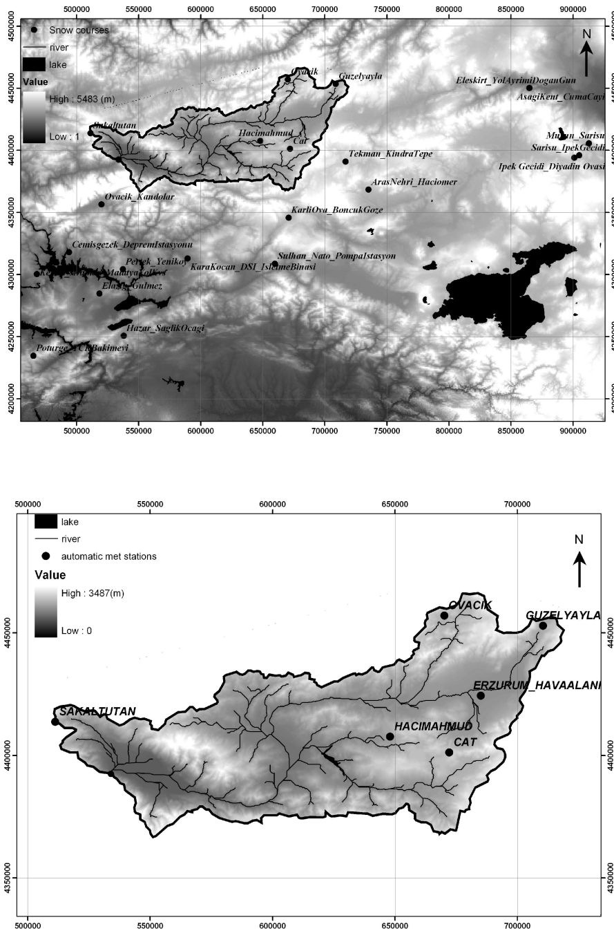
Fig. 2. (a) Snow courses on the topographic map of Karasu Basin and the surrounding area, (b) AWOS locations on the DEM of Karasu Basin.
