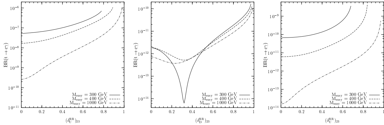
FIG. 8: The gluino, chargino and neutralino contributions to the \text{BR}(t \rightarrow c\gamma) as function of (\delta_{U(D)}^{RR})_{23} for the case where the flavor changing effects come from the mixing in the RR sector only. The graph on the left(right) denotes the gluino(neutralino) contribution for the up RR mixing. The one in the middle is for the chargino as a function of (\delta_D^{RR})_{23} . Three representative M_{\text{susy}} values (300,400,1000) GeV are chosen, with m_{\tilde{g}} = 300 GeV, \tan\beta = 10 , A = M_{\text{susy}} and \mu = 200 GeV.
