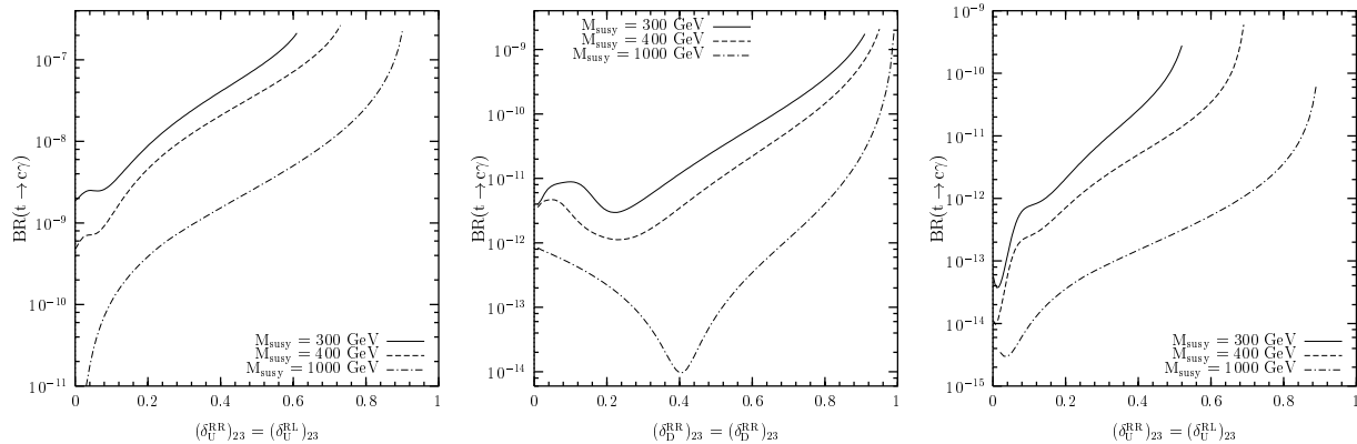
FIG. 9: The same as Fig.8 but for the case where both (\delta_{U(D)}^{RR})_{23} and (\delta_{U(D)}^{RL})_{23} contribute, with the assumption (\delta_{U(D)}^{RR})_{23} = (\delta_{U(D)}^{RL})_{23} .
