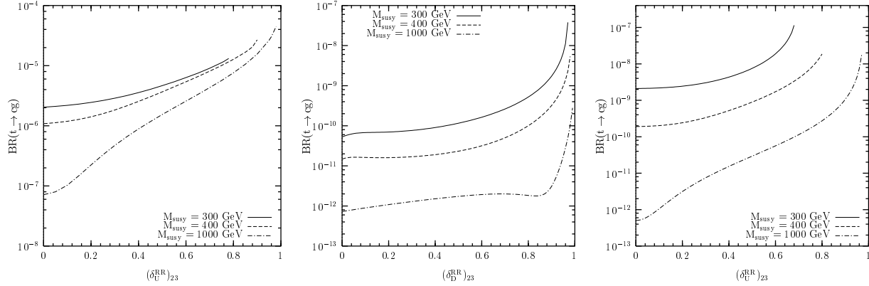
FIG. 5: The gluino, chargino and neutralino contributions to the \text{BR}(t \rightarrow cg) as function of (\delta_{U(D)}^{RR})_{23} for the case where the flavor changing effects come from the mixing in the RR sector only. The graph on the left(right) denotes the gluino(neutralino) contribution for the up RR mixing. The one in the middle is for the chargino as a function of (\delta_D^{RR})_{23} . Three representative M_{\text{susy}} values (300,400,1000) GeV are chosen with m_{\tilde{g}} = 300 GeV, \tan\beta = 10 , A = M_{\text{susy}} and \mu = 200 GeV.
