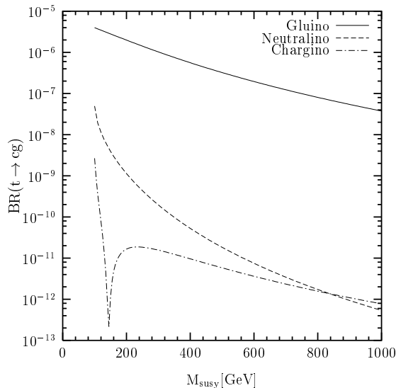
FIG. 2: The gluino, chargino and neutralino contributions to the \text{BR}(t \rightarrow cg) as a function of M_{\text{susy}} in the flavor diagonal scenario for m_{\tilde{g}} = 300 GeV, \tan \beta = 10 together with the parameter values defined at the beginning of section V. The solid, dashed, dotted-dashed curves as coded represent gluino, neutralino and chargino contributions, respectively.
