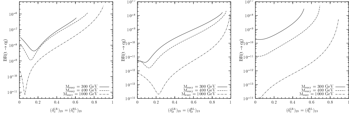
FIG. 7: The same as Fig.5 but for the case where both (\delta_{U(D)}^{LR})_{23} and (\delta_{U(D)}^{RL})_{23} contribute, with the assumption (\delta_{U(D)}^{LR})_{23} = (\delta_{U(D)}^{RL})_{23} .
