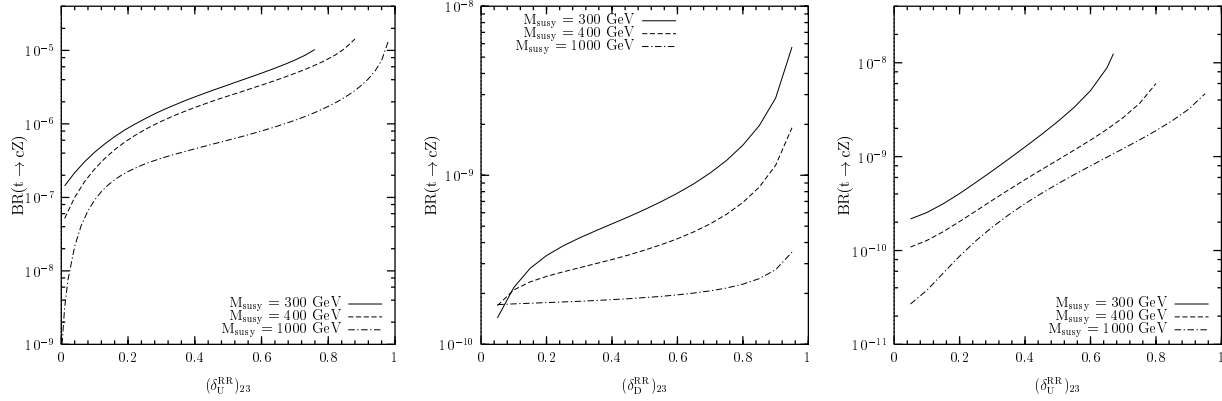
FIG. 10: The gluino, chargino and neutralino contributions to the BR(t \rightarrow cZ) as function of (\delta_{U(D)}^{RR})_{23} for the case where the flavor changing effects come from the mixing in the RR sector only. The graph on the left(right) denotes the gluino(neutralino) contribution for the up RR mixing. The one in the middle is for the chargino as a function of (\delta_D^{RR})_{23} . Three representative M_{\text{susy}} values (300,400,1000) GeV are chosen with m_{\tilde{g}} = 300 GeV, \tan \beta = 10 , A = M_{\text{susy}} and \mu = 200 GeV.
