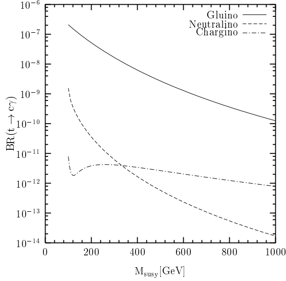
FIG. 3: The same as Fig. 2 but for the t \rightarrow c\gamma decay mode.
