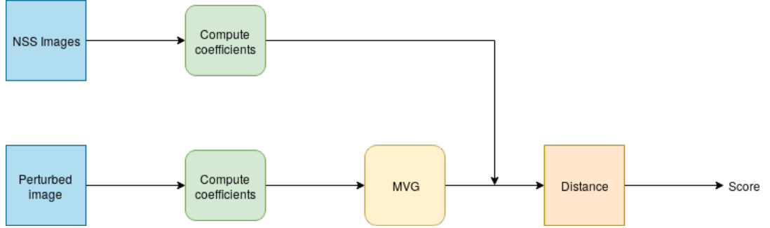
Figure 3.3: NIQE Algorithm
