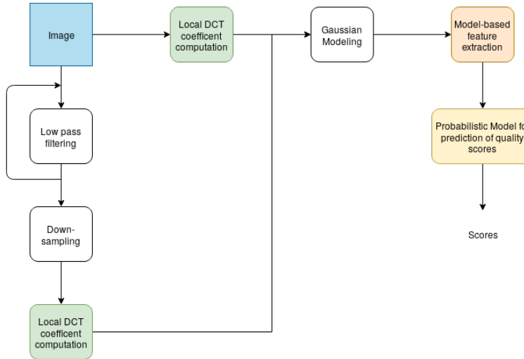
Figure 3.2: BLIINDS-2 Algorithm
