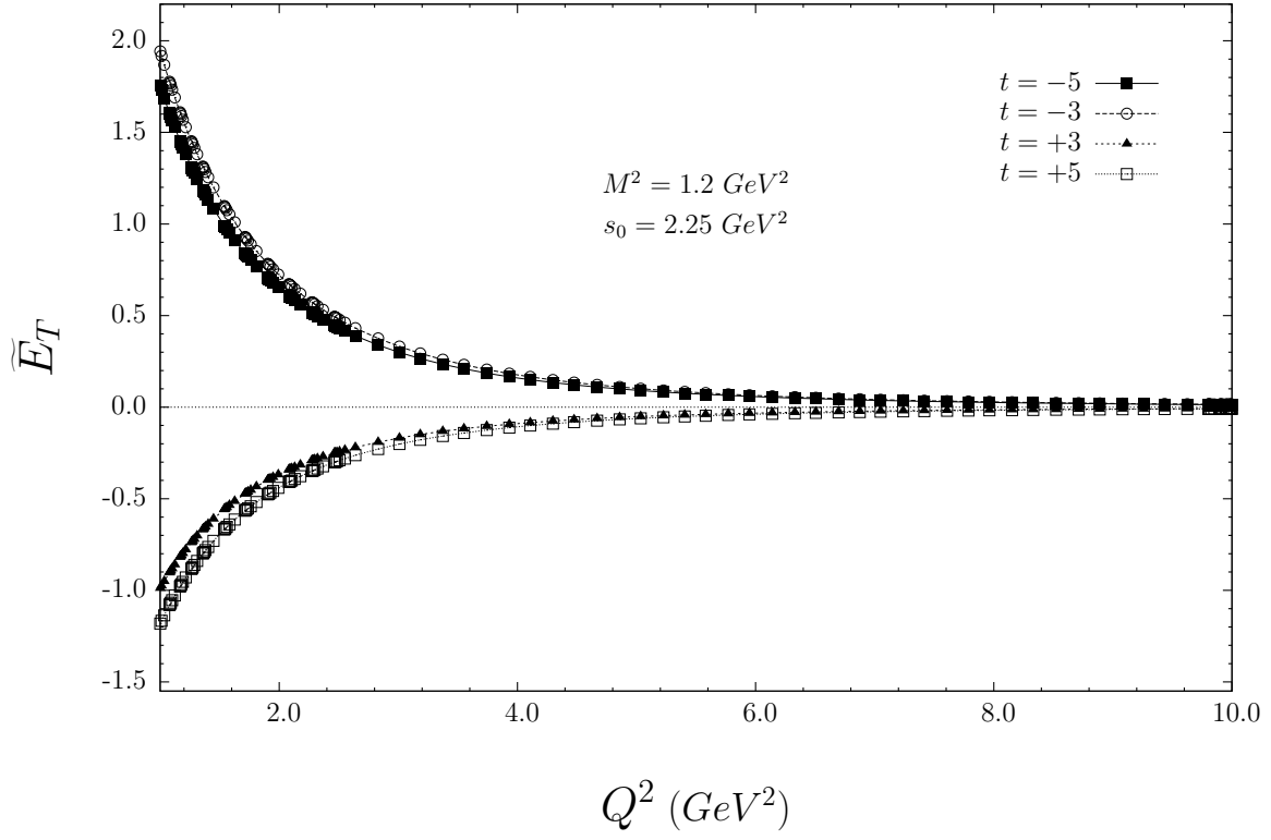
Figure 7: The same as in Fig. (4), but for the isovector current.
