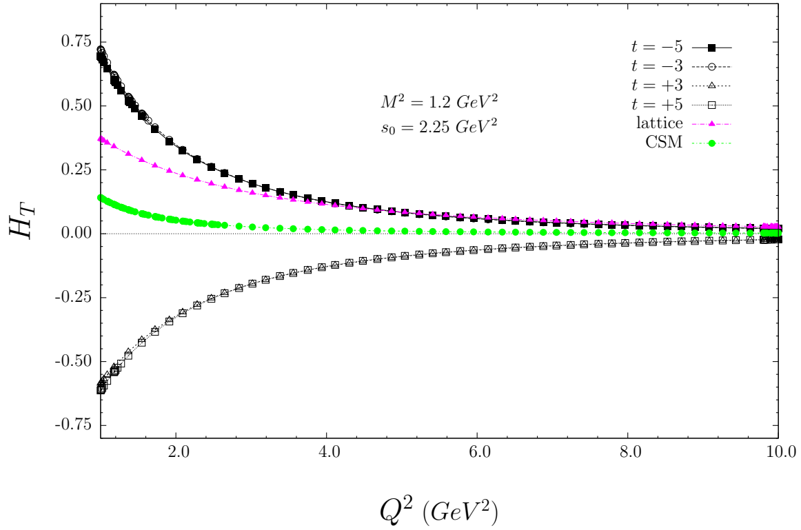
Figure 3: The dependence of H_T on Q^2 at M^2 = 1.2 \text{ GeV}^2 and s_0 = 2.25 \text{ GeV}^2 and four fixed values of t : t = -5; -3; 3; 5 , for the isoscalar current.
