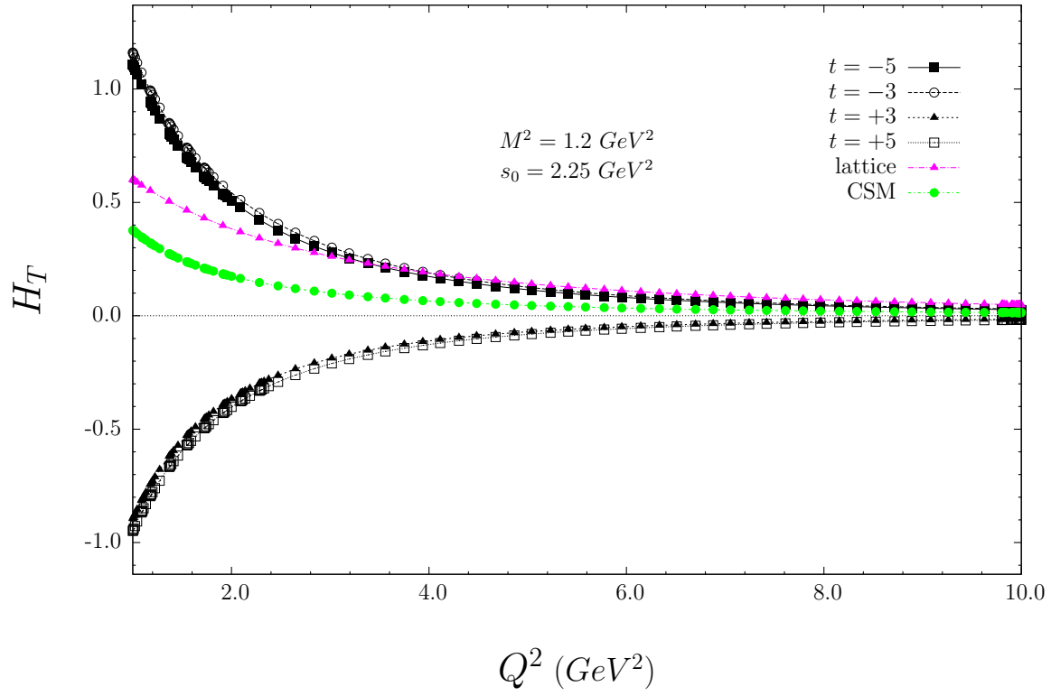
Figure 6: The same as in Fig. (3), but for the isovector current.
