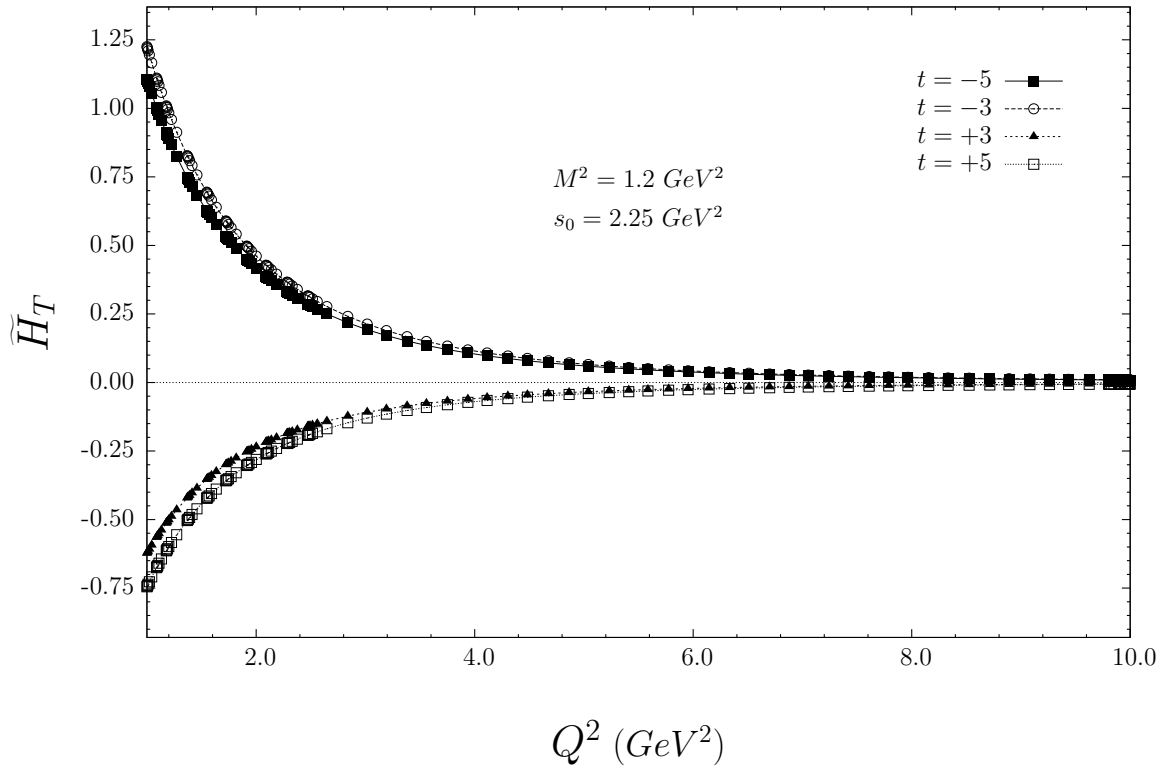
Figure 5: The same as in Fig. (3), but for the form factor \tilde{H}_T(Q^2) .
