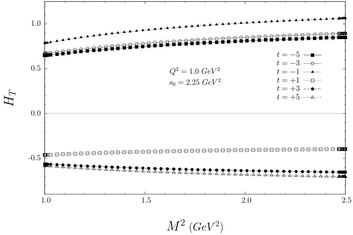
Figure 1: The dependence of the form factor H_T of nucleon on M^2 at Q^2 = 1 \text{ GeV}^2 and s_0 = 2.25 \text{ GeV}^2 , at six different values of t : t = -5; -3; -1; 1; 3; 5 , using the first set of DAs for the isoscalar current.
