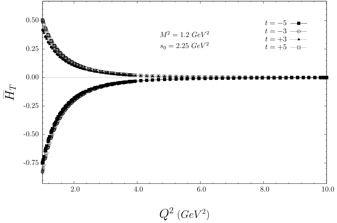
Figure 8: The same as in Fig. (5), but for the isovector current.
