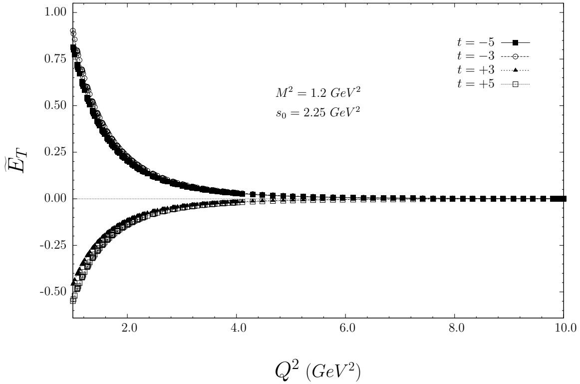
Figure 4: The same as in Fig. (3), but for the form factor \tilde{E}_T(Q^2) .
