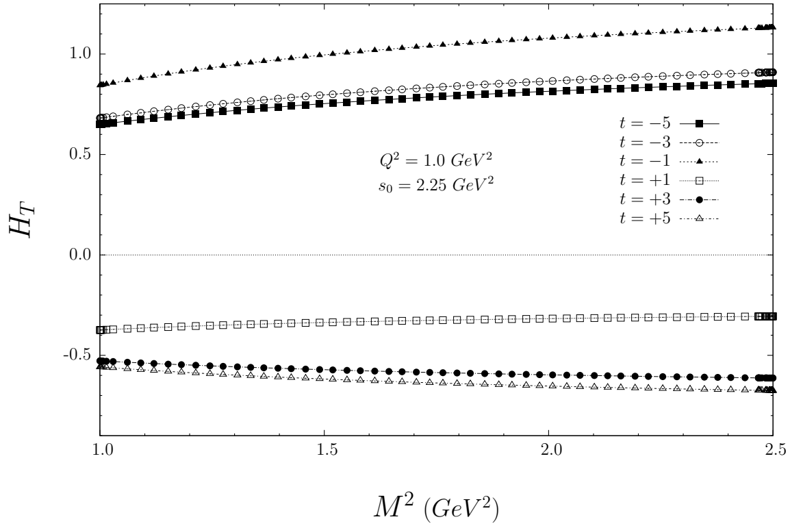
Figure 2: The same as in Fig. (1), but at s_0 = 2.5 \text{ GeV}^2 and using the second set of DAs.
