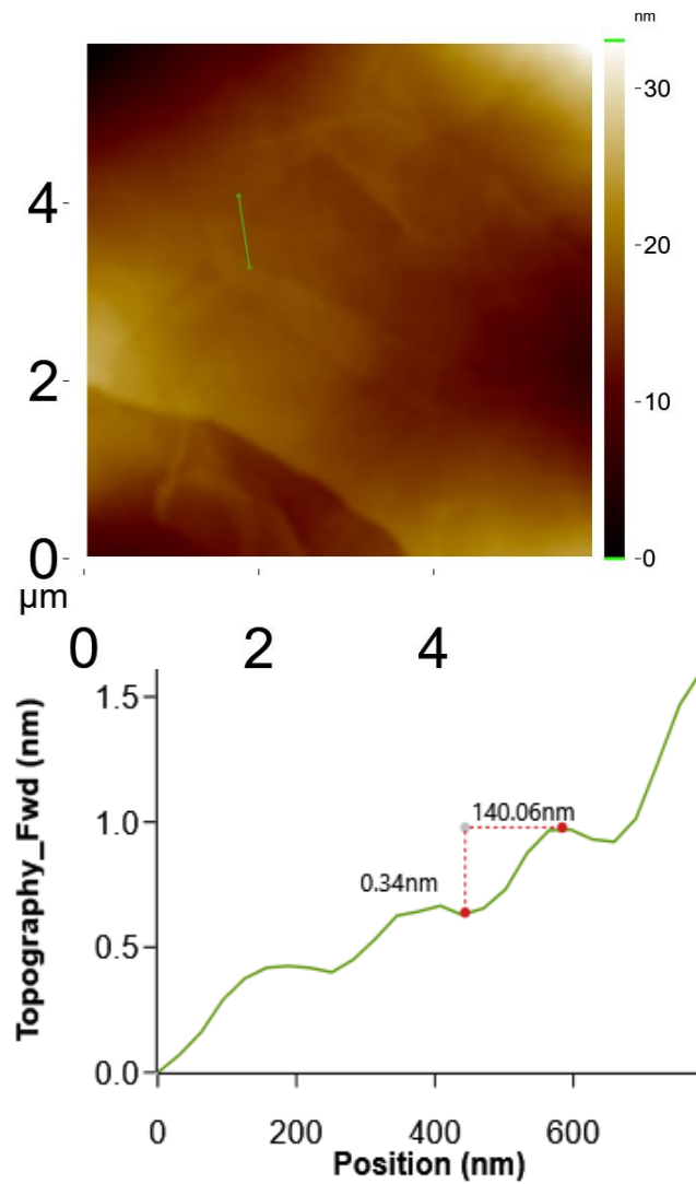
Figure 5. 15 Single-layer Graphene.
