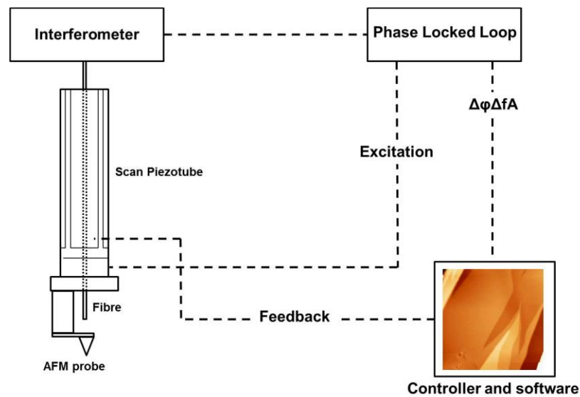
Figure 3. 20 LT-AFM control scheme.[51]
