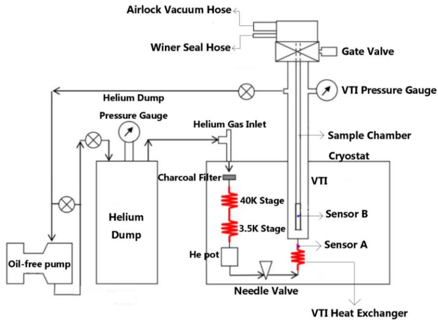
Figure 5. 2 The cryostat and gas handling system schematic design. [65]
