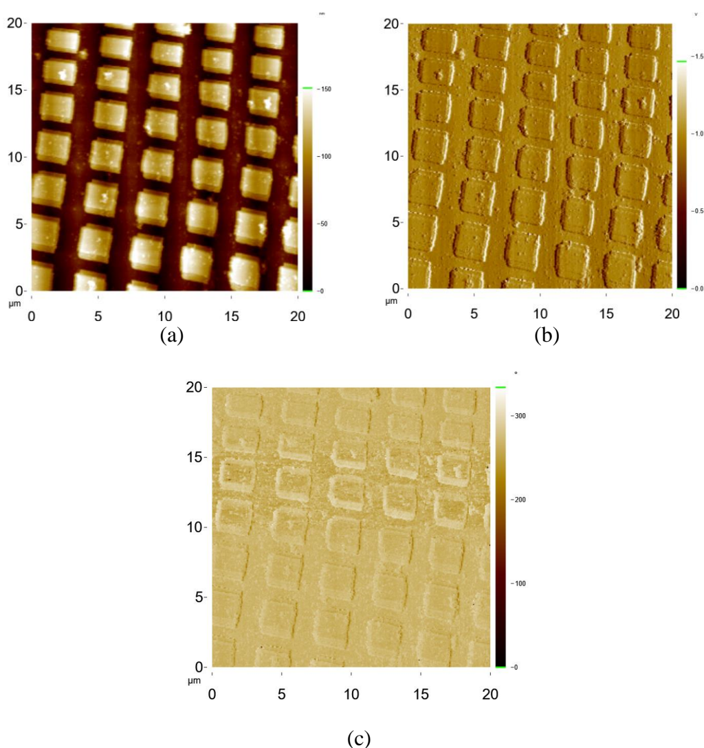
Figure 6. 14 AFM image of the grating sample in Tapping mode at 300 K. (a) Sample Topography, (b) Amplitude (Feedback) and, (c) Phase images.
