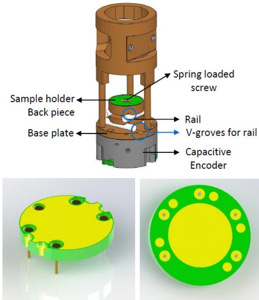
Figure 3. 11 Sample positioner and holders. [49]
