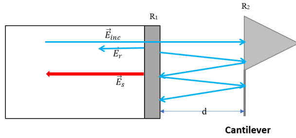
Figure 6. 10 schematic design of the fiber-cantilever reflectivity. \vec{E}_{inc} , \vec{E}_r , \vec{E}_s are respectively the incident beam, the fiber surface reflected beam, the summation of the cantilever and fiber reflected beam, R_1 fiber surface reflectivity, R_2 cantilever Reflectivity.
