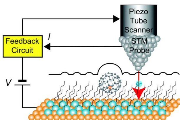
Figure 1. 2 schematic of scanning tunneling microscopy. [12]
