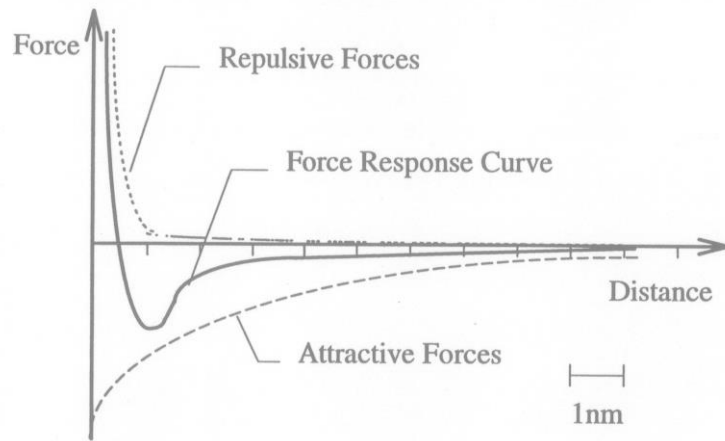
Figure 2. 9 The graph represents the attractive and repulsive regime in Lennard-Jones potential [50]
