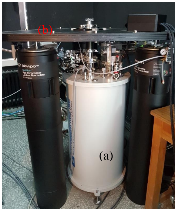
Figure 5. 6 (a) The cryostat, and (b) Isolation Vibration Platform.
