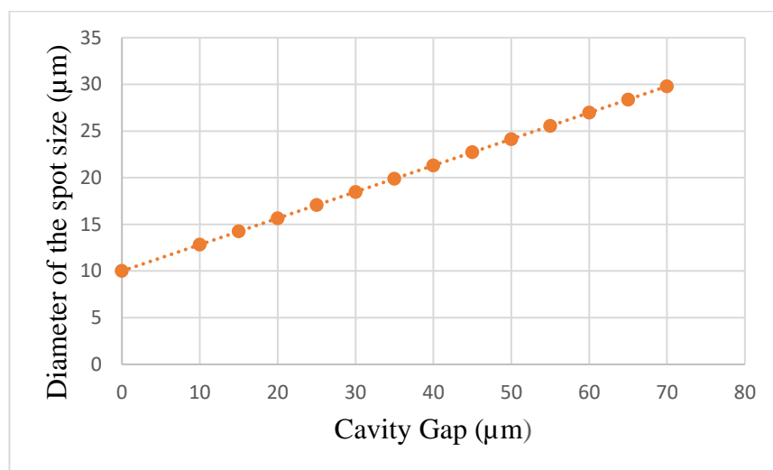
Figure 4. 2 Cavity gap vs spot size diameter.
