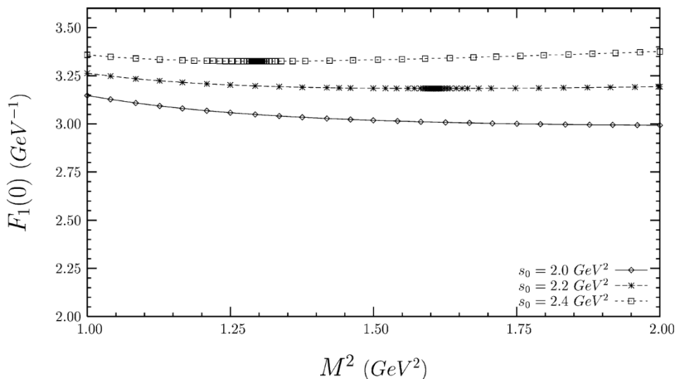
Fig. 1. The dependence of the transition form factor F_1(0) for the radiative \phi \rightarrow f_0 \gamma decay on M^2 at three different values of the continuum threshold s_0 = 2.0 \text{ GeV}^2 , 2.2 \text{ GeV}^2 and 2.4 \text{ GeV}^2 .
