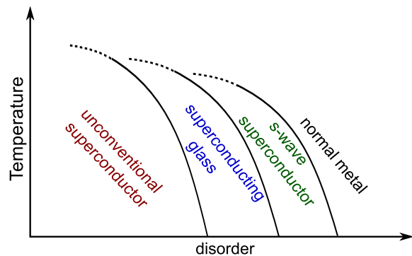
FIG. 2: Schematic picture of the phase diagram of an unconventional superconductor as a function of temperature and disorder
