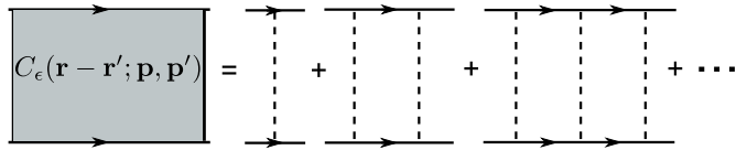
FIG. 1: Diagrammatic representation of the Cooperon ladder. Solid lines are electron Green's functions whereas dashed lines are impurities. \hat{C}(\mathbf{r} - \mathbf{r}'; \mathbf{p}, \mathbf{p}') in Eq. (9) is obtained by integration of this ladder over energy.
