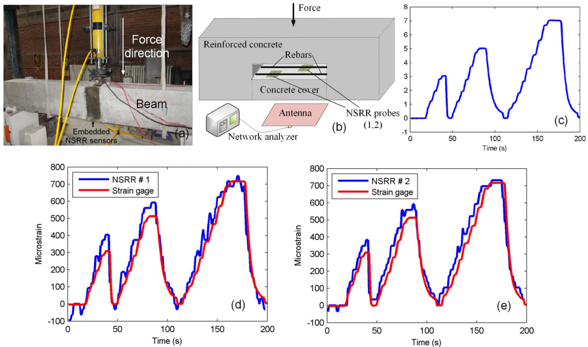
Fig. 9. Simultaneous multi-point sensing by two different sensors in a simply supported beam experiment: (a) Experiment setup. (b) Diagram showing the placement of NSRR probes on the reinforcing bars within the beam. (c) Applied force plotted versus time (load cell value). (d) NSRR # 1 strain versus time compared with strain gage data. (e) NSRR # 2 strain versus time compared with strain gage data.
