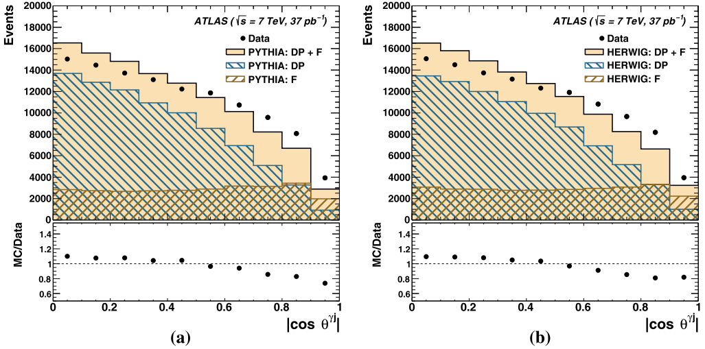
Fig. 5. The estimated signal yield in data (dots) using the signal leakage fractions from (a) PYTHIA or (b) HERWIG as functions of |\cos \theta^{\gamma}| . These distributions do not include requirements on m^{\gamma j} or |\eta^{\gamma} + y^{\text{jet}}| . Other details as in the caption to Fig. 3.
