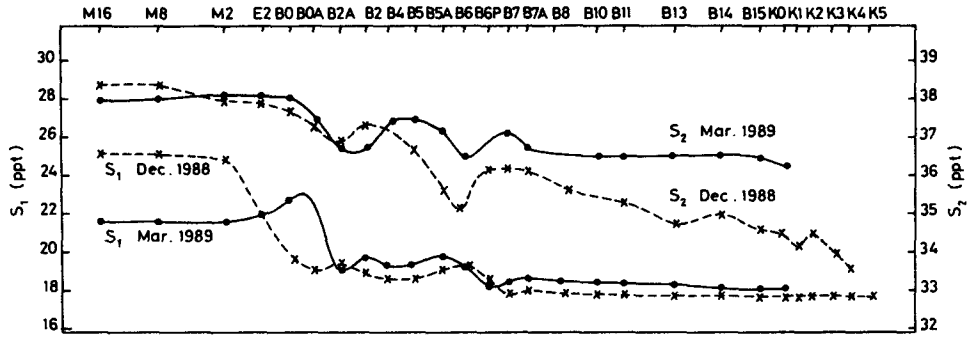
FIG. 8. Average salinities in the upper layer ( S_1 ) and in the lower layer ( S_2 ) in the Bosphorus Strait for December 1988 (×) and March 1989 (●).
