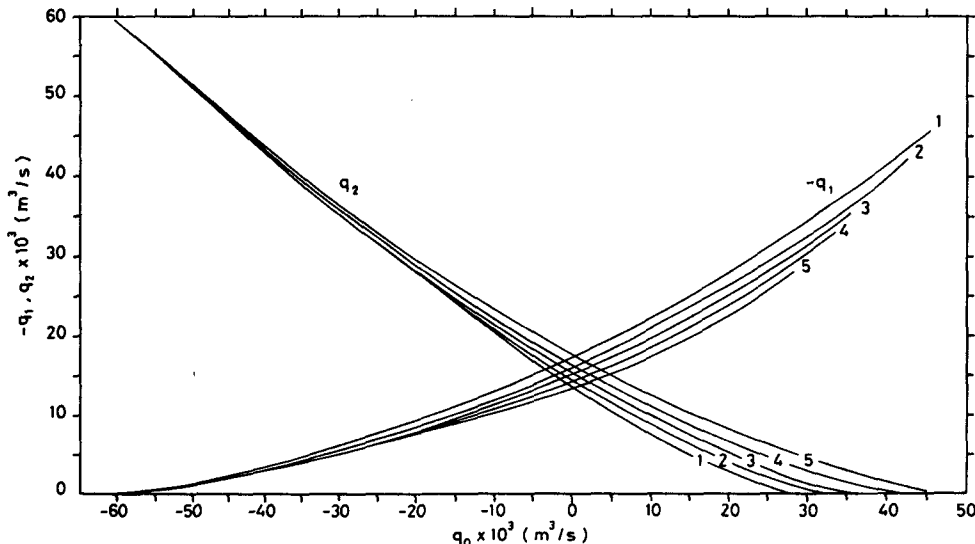
FIG. 10. Upper and lower layer transports ( -q_1, q_2 ) versus q_0 obtained by the analytic model.
