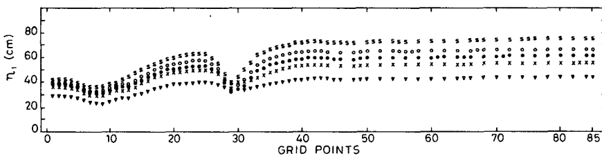
FIG. 5c. Computed variations of the free surface elevation for various values of q_0 : 4380 \text{ m}^3 \text{ s}^{-1} ( \nabla ), 10500 \text{ m}^3 \text{ s}^{-1} ( \times ), 12350 \text{ m}^3 \text{ s}^{-1} ( \bullet ), 16600 \text{ m}^3 \text{ s}^{-1} ( \circ ) and 21765 \text{ m}^3 \text{ s}^{-1} ( \blacksquare ).
