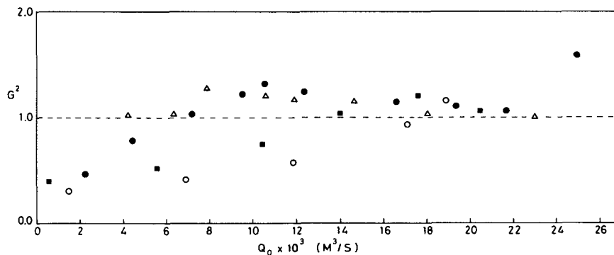
FIG. 6. Composite Froude number versus the net barotropic flow at grid point 32 for different values of friction coefficients with C_b = 0.0023 and (a): C_i = 0.0005 ( \circ ), (b): C_i = 0.0003 ( \blacksquare ), (c): C_i = 0.0001 ( \bullet ) and with (d): C_b = 0.0010 , C_i = 0.0001 ( \nabla ).
