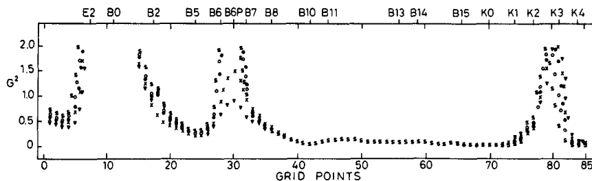
FIG. 5a. Computed variations of the composite Froude number for various values of q_0 : 4380 \text{ m}^3 \text{ s}^{-1} ( \nabla ), 10500 \text{ m}^3 \text{ s}^{-1} ( \times ), 12350 \text{ m}^3 \text{ s}^{-1} ( \bullet ), 16600 \text{ m}^3 \text{ s}^{-1} ( \circ ) and 21765 \text{ m}^3 \text{ s}^{-1} ( \blacksquare ).
