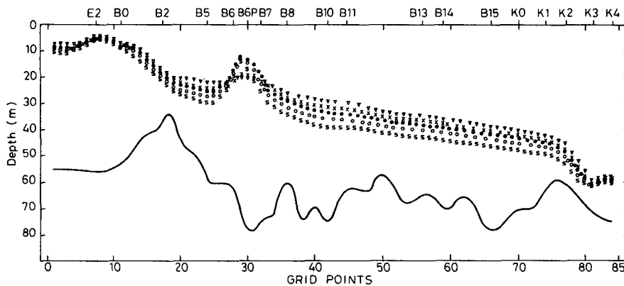
FIG. 5b. Computed variations of the interface depth for various values of q_0 : 4380 \text{ m}^3 \text{ s}^{-1} ( \nabla ), 10500 \text{ m}^3 \text{ s}^{-1} ( \times ), 12350 \text{ m}^3 \text{ s}^{-1} ( \bullet ), 16600 \text{ m}^3 \text{ s}^{-1} ( \circ ) and 21765 \text{ m}^3 \text{ s}^{-1} ( \blacksquare ).
