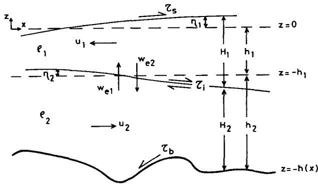
FIG. 4a. Definition sketch for some model parameters.
