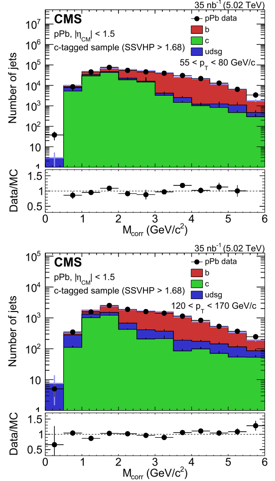
Fig. 2. Corrected secondary vertex mass distributions from PYTHIA+HIJING for c jets (green), light parton jets (blue), and b jets (red) in the jet p_T range 55–80 GeV/c (upper) and 120–170 GeV/c (lower). Relative normalizations of these three distributions are fit to a distribution from pPb collision data (black). Statistical uncertainties are shown in black for data and for individual simulated flavor components and are shown in blue for the sum of the simulated distributions. The bottom panels of both plots show the ratio of data to simulation. (For interpretation of the colors in this figure, the reader is referred to the web version of this article.)
