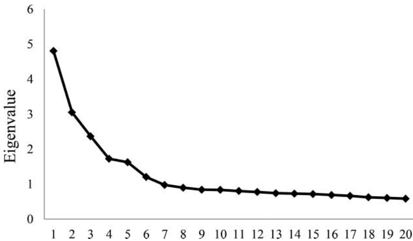
FIGURE 1 Scree plot of exploratory factor analysis.
