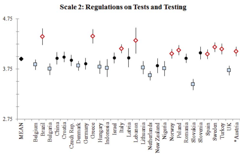
FIGURE 3 Scale Two: Random intercepts and confidence intervals for countries in conditional model.
