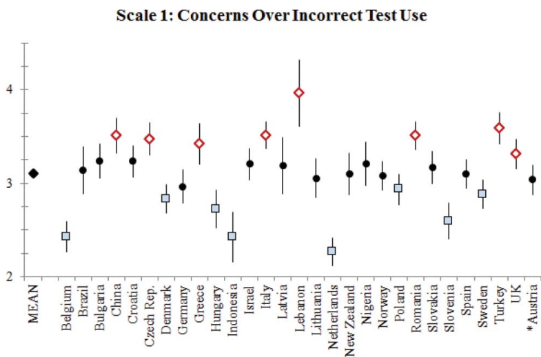
FIGURE 2 Scale One: Random intercepts and confidence intervals for countries in conditional model.
