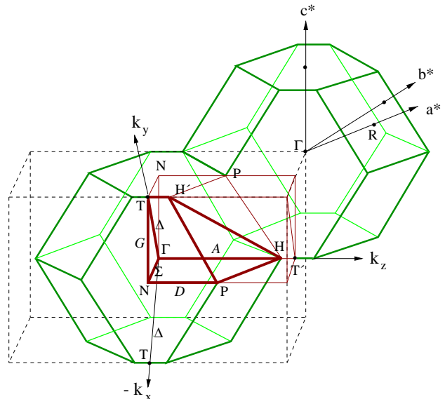
FIG. 2: The irreducible wedge (heavy lines) of the first Brillouin zone for TlSe structure with the high symmetry points and high symmetry lines indicated.
