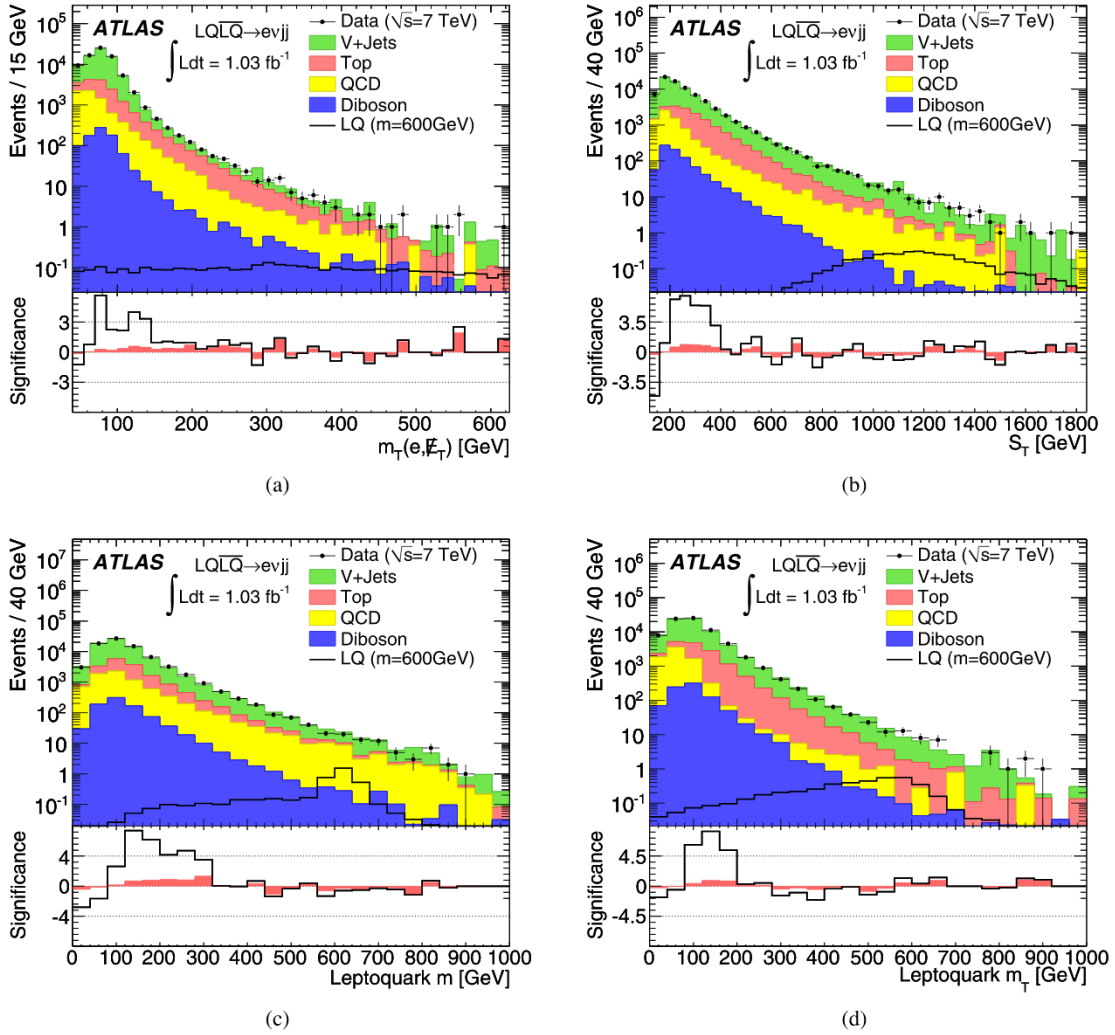
Fig. 2. Data and SM background comparisons of the input LLR variables for the evjj channel. (a) Transverse mass of the electron and the E_T^{\text{miss}} in the event, (b) S_T , (c) LQ mass, and (d) LQ transverse masses. The stacked distributions show the various background contributions, and data are indicated by the points with error bars. The 600 GeV LQ signal is also shown for \beta = 0.5 . The solid line (band) in the lower plots shows the Gaussian statistical (statistical + systematic) significance of the difference between data and the prediction.
