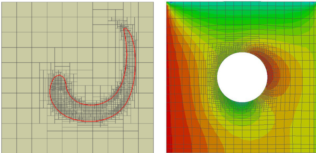
Figure 1. Examples of (a) interface deformation in a decaying vortex using h -refinement and (b) temperature distribution around a cylinder using hr -refinement.
