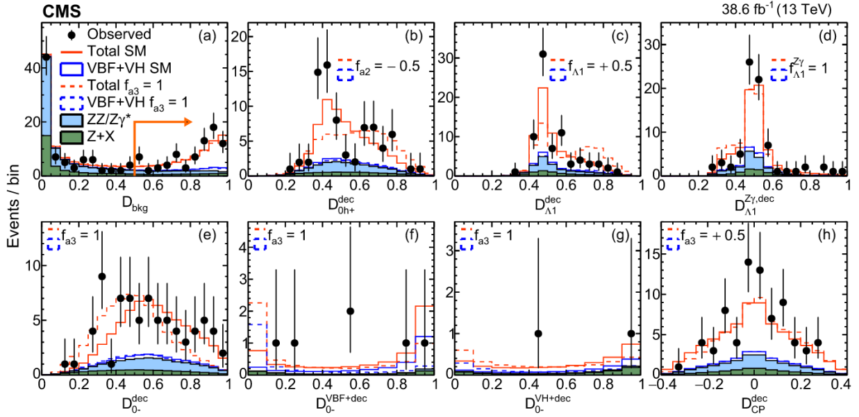
Fig. 2. Distributions of \mathcal{D}_{\text{bkg}} (a) for all events in Run2; \mathcal{D}_{0h+} (b), \mathcal{D}_{\Lambda 1} (c), \mathcal{D}_{\Lambda 1}^{Z\gamma} (d), \mathcal{D}_{0-} (e), and \mathcal{D}_{CP} (h) for the untagged and 2015 events; \mathcal{D}_{0-} in the VBF-jet (f) and VH-jet (g) categories. The arrow in (a) indicates the requirement \mathcal{D}_{\text{bkg}} > 0.5 , used to suppress background on all other plots. Points with error bars show data and histograms show expectations for background and signal, as indicated in the legend in (a). The dashed lines show expectations for BSM hypotheses, as indicated in the individual legends.
