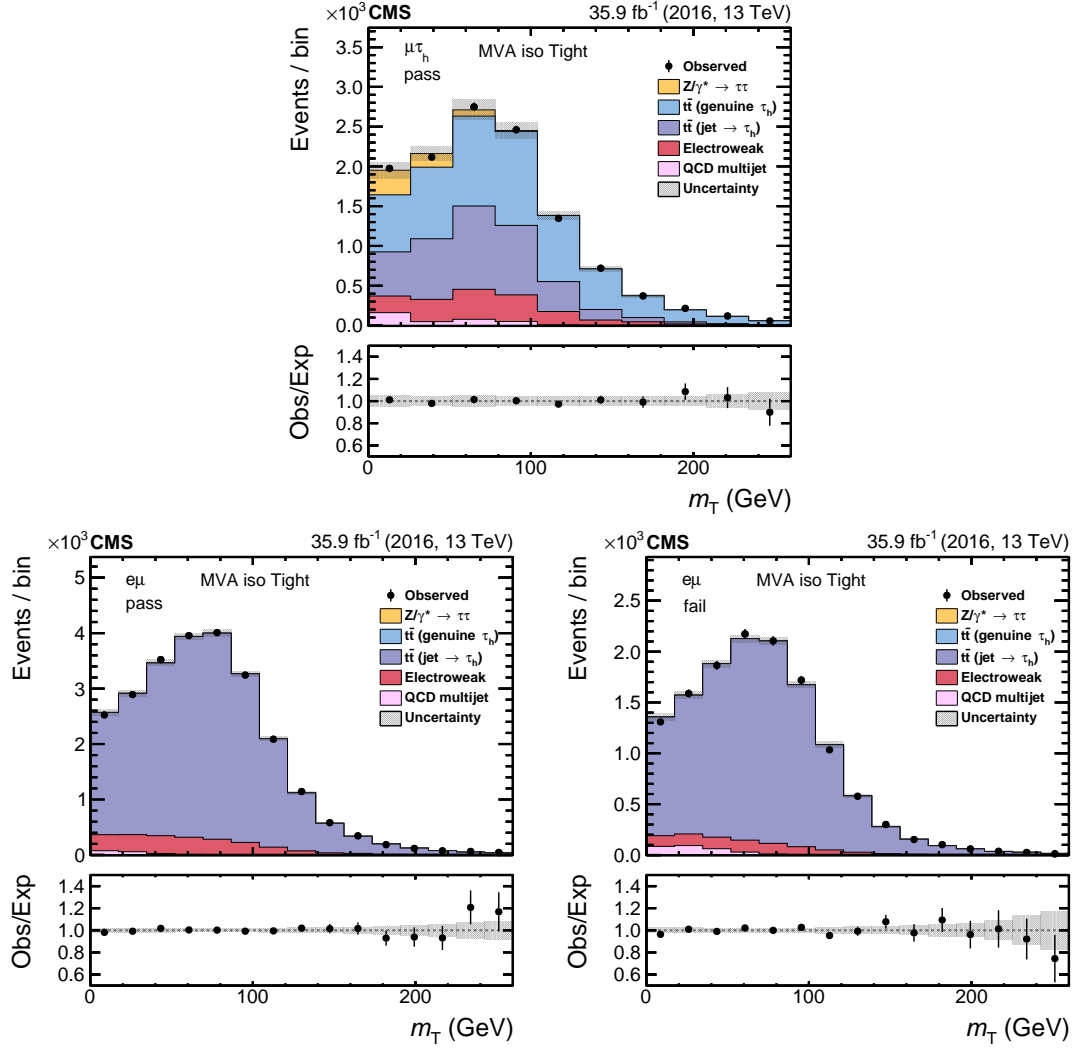
Figure 8. Fitted distributions for the signal (upper), e\mu passing (lower left), and the e\mu failing (lower right) categories, using the m_T for the \vec{p}_T^\mu and \vec{p}_T^{\text{miss}} vectors as observables for the tight WP of the MVA-based isolation with p_T^{\tau_h} between 30 and 40 GeV. The electroweak background includes contributions from W+jets (dominating), diboson, and single top quark events. Vertical bars correspond to the statistical uncertainties in the data points (68% frequentist confidence intervals), while the shaded bands reflect the quadratic sum of the statistical and systematic uncertainties after the fit.
