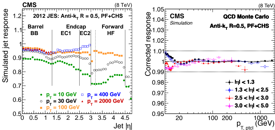
Figure 10. Simulated jet response R_{\text{ptcl}} versus |\eta| for R = 0.5 (left). Simulated jet response R_{\text{ptcl}} , after JEC have been applied, versus p_{T, \text{ptcl}} for R = 0.5 in various \eta regions, and with statistical uncertainties (right).
