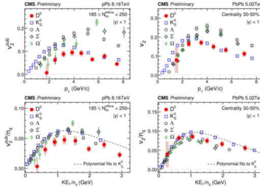
Fig. 3. The top plots show our measurements of D^0 , K_S^0 , \Lambda , \Xi^- , and \Omega^- v_2 vs p_T in pPb (left) and PbPb (Right). The bottom plots, motivated by NCQ scaling [16], show v_2/n_q vs transverse energy KE_T/n_q in pPb (left) and PbPb (right) [7].
