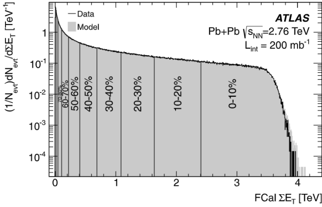
Fig. 1. Measured FCal \Sigma E_T distribution divided into 10% centrality intervals (black). Proton–proton data at \sqrt{s} = 2.76 TeV, convolved with a Glauber Monte Carlo calculation with x = 0.088 (grey), as described in the text.
