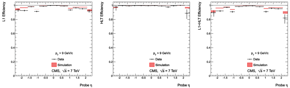
Figure 34. Single-muon trigger efficiencies for Soft Muons as a function of the Soft Muon \eta , for muons with p_T in the range of 9 < p_T < 20 \text{ GeV}/c : the efficiency of the Level-1 trigger with p_T threshold at 3 GeV/c (left), the efficiency of the HLT with p_T threshold of 5 GeV/c with respect to Level-1 (middle), and the combined efficiency of Level-1 and HLT (right). The efficiencies obtained using J/\psi \rightarrow \mu^+ \mu^- events (points with error bars) are compared with predictions from the MC simulation ( \pm 1\sigma bands); the uncertainties are statistical only.
