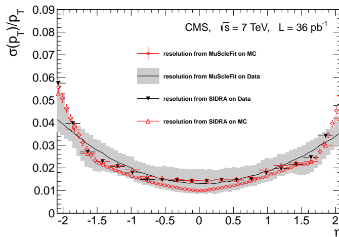
Figure 21. Relative transverse momentum resolution \sigma(p_T)/p_T in data and simulation measured by applying the MuSleFit and SIDRA methods to muons produced in the decays of Z bosons and passing the Tight Muon selection. The thin line shows the result of MuSleFit on data, with the grey band representing the overall (statistical and systematic) 1\sigma uncertainty of the measurement. The circles are the result of MuSleFit on simulation. The downward-pointing and upward-pointing triangles are the results from SIDRA obtained on data and simulation, respectively; the resolution in simulation was evaluated by comparing the reconstructed and “true” p_T once the reconstructed p_T was corrected for \phi -dependent biases. The uncertainties for SIDRA are statistical only and are smaller than the marker size.
