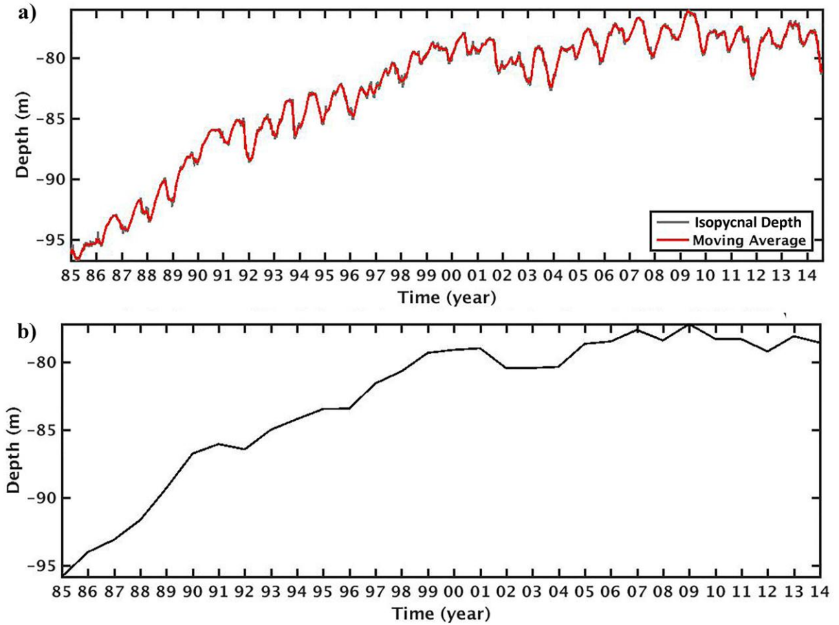
Figure 44: Daily isopycnal ( 15.4 \text{ kg/m}^3 ) depth variation from 1985 to 2014 (a) and annual mean isopycnal ( 15.4 \text{ kg/m}^3 ) variations from 1985 to 2014 (b).
