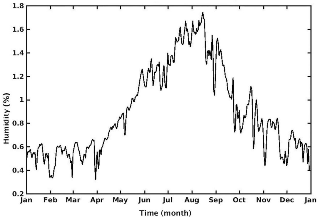
Figure 10: Basin-averaged mean values for specific humidity calculated from ECMWF Era-Interim dataset averaged over the time frame 1985-20142 m dew point temperature and surface pressure.
