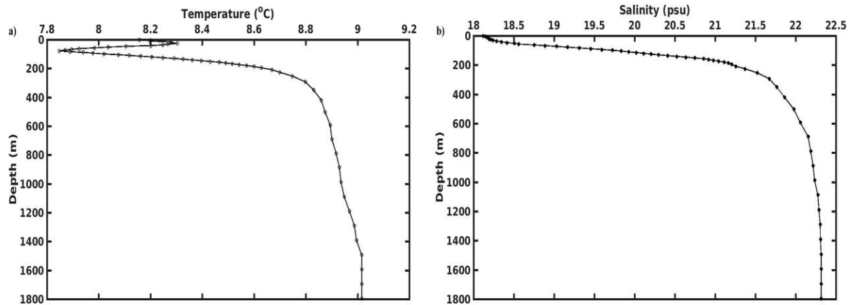
Figure 6: Decadal averaged initial temperature (a) and salinity (b) profiles for January from WOA 2013 (Locarnini et al., 2013; Zweng et al., 2013).
