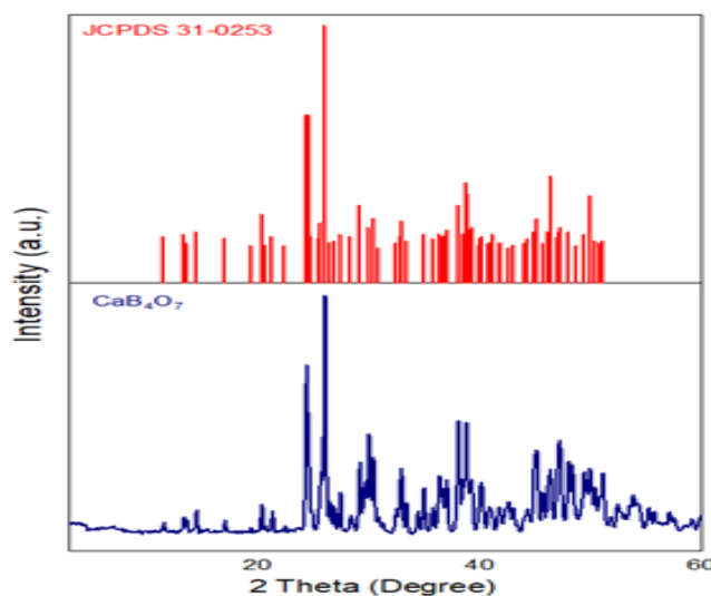
Figure 1 The X-ray pattern of synthesized calcium tetraborate
