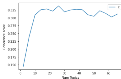
Figure 5: Coherence score for the topic numbers
